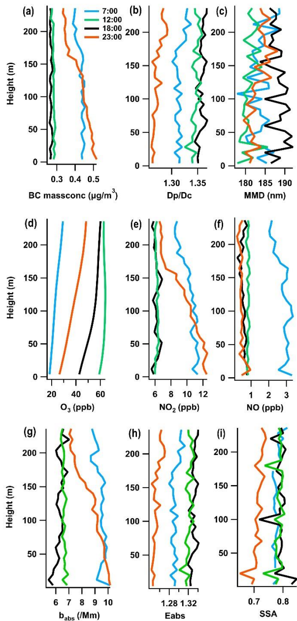
Figure. 4 The diurnal variation of the average profiles of BC properties including (a) BC, (b) D_p/D_c , (c)MMD. The average profiles of (d) O_3 and its precursors (e) NO_2 and (f) NO . The averaged profiles of aerosol optical properties including (g) absorption coefficient, (h) absorption enhancement of BC due to coatings, (i) single scattering albedo.
