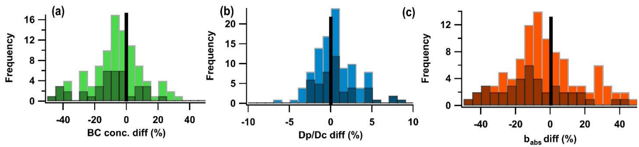
705 Figure. 7 Histogram of the number frequency of the relative differences between 240 m and the ground for a) BC concentration , (b) D_p/D_c and (c) b_{abs} . The shaded black area denotes the number frequency at night and morning (6:00,7:00, 8:00, 22:00, 23:00), the black line denotes no difference between 240m and the ground.
