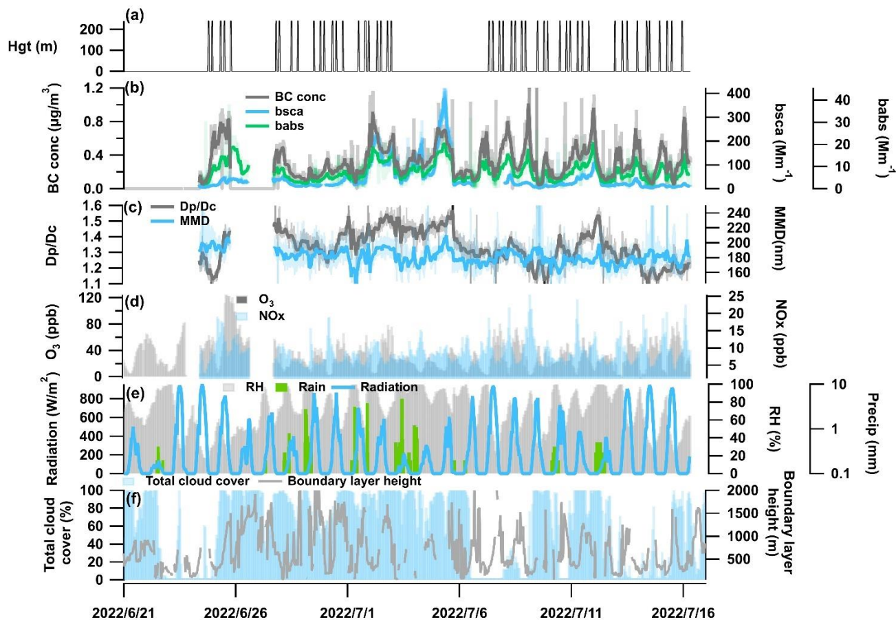
670 Figure. 1 Time series of the major parameters during the observation. (a) The height of the moveable container. (b) Mass concentration of black carbon and absorption ( b_{\text{abs}} ) and scattering coefficient ( b_{\text{sca}} ), the solid and light-coloured lines denote the data with 1-hour and 1-min average. (c) The coating thickness ( D_p/D_c ) and mass median diameter (MMD) of BC, the solid and light-coloured lines denote the data with 1-hour and 1-min average. (d) The 1-min averaged mixing ratio of \text{O}_3 and \text{NO}_x . (e)(f) The meteorological conditions during the observation period.
