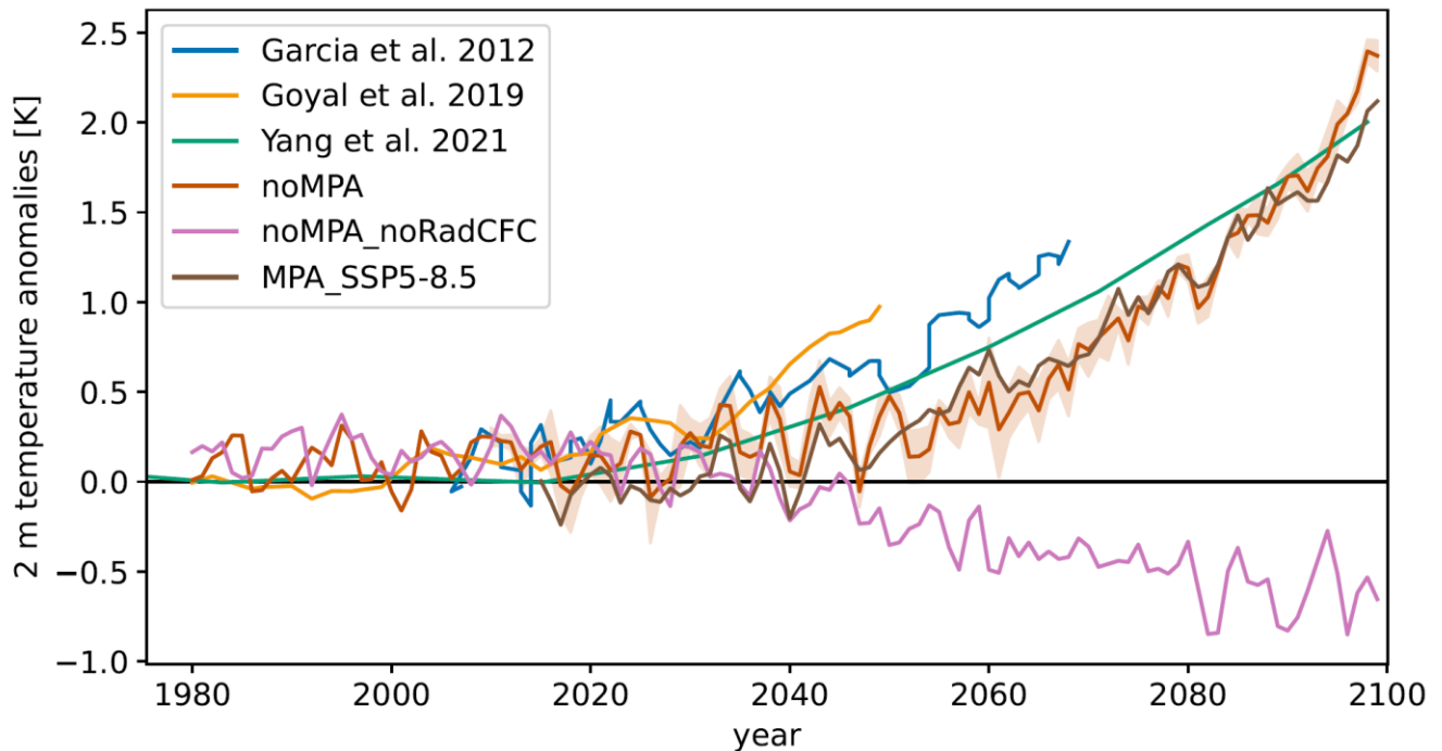
Figure 4: Global mean surface air temperature deviation for the noMPA (red line), MPA-ssp585 (brown line), and noMPA_noRadCFC (violet line) from the reference MPA-ssp245 run. Light-A light red shadow illustrates internal variability in the noMAP run. For comparisons, the same quantity is shown using digitized data from Garcia et al. (2012, blue line), Goyal et al. (2019, yellow line), and 255 Young et al. (2021, light green line).
