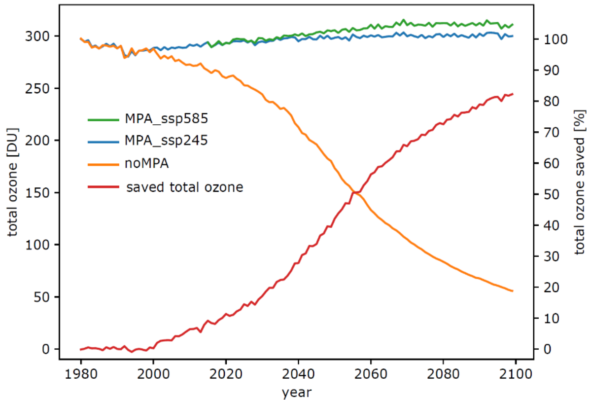
155 Figure 1: Time evolution of the global mean annual mean total ozone (DU) for the MPA_ssp245 (blue line), MPA_ssp585 (green line), and noMPA (orange line) simulations, the red line illustrates saved total ozone by the MPA limitations (MPA_ssp245-noMPA).
