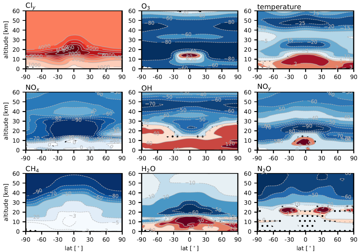
220 Figure 3: Zonal, annual, and ensemble mean of total inorganic chlorine ( \text{Cl}_y ), \text{O}_3 , \text{NO}_x(\text{N}+\text{NO}+\text{NO}_2) , OH, \text{H}_2\text{O} , total reactive nitrogen ( \text{NO}_y ), \text{CH}_4 , \text{H}_2\text{O} , \text{N}_2\text{O} (in %), and temperature (in K) response to the absence of the MPA regulations (noMPA relative to - MPA-ssp245) averaged over 2080–2099. All differences are statistically significantly different from zero at the 90% level except areas with black dots.
