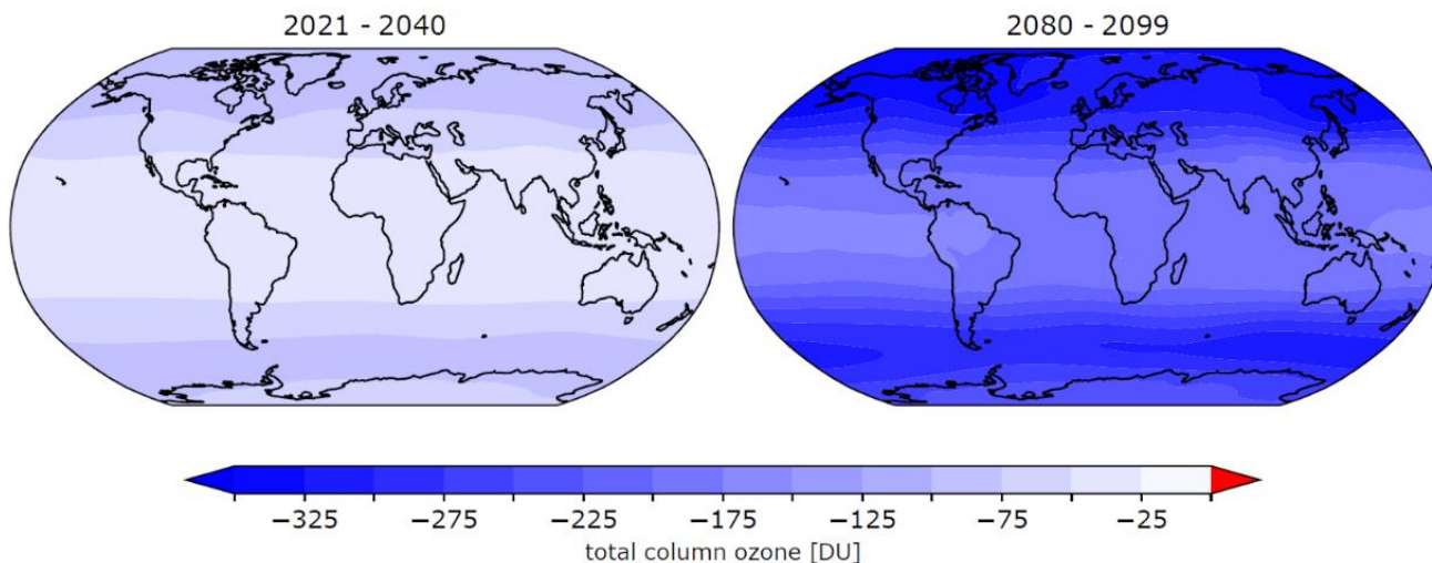
165 Figure 2: Geographical distribution of the annual mean total ozone difference (in D.U.) between noMPA and MPA-ssp245 simulations, averaged over the periods 2021-2040 (left) and 2080-2099 (right). All differences are statistically significantly different from zero at the 90% level
