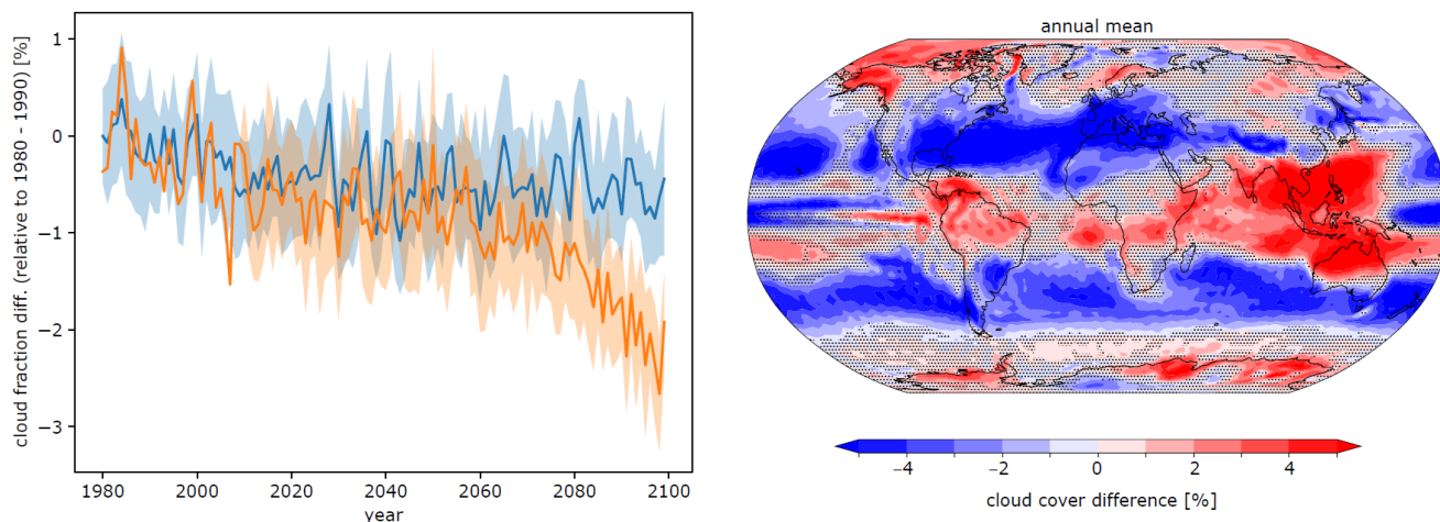
295 Figure 6: Time evolution of global and annual mean cloud cover change (left panel) for MPA-ssp245 (blue) and for noMPA (orange) cases relative to 1980-1990 mean and geographical distribution (right panel) of the annual mean difference in cloud cover (%) between noMPA and MPA_ssp245 simulations, averaged over the period 2090–2100. Areas, where the statistical significance of the signal is less than 90%, are marked by dots.
