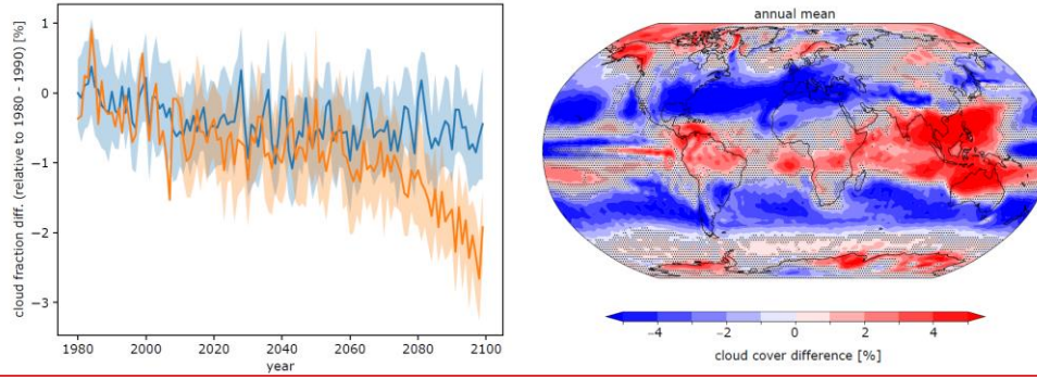
305 Figure 6: Time evolution of global and annual mean cloud cover change (left panel) for MPA-ssp245 (blue) and for noMPA (orange) cases relative to 1980-1990 mean and geographical distribution (right panel) of the annual mean difference in cloud cover (%) between noMPA and MPA_ssp245 simulations, averaged over the period 2090–2100. Areas, where the statistical significance of the signal is less than 90%, are marked by dots.
