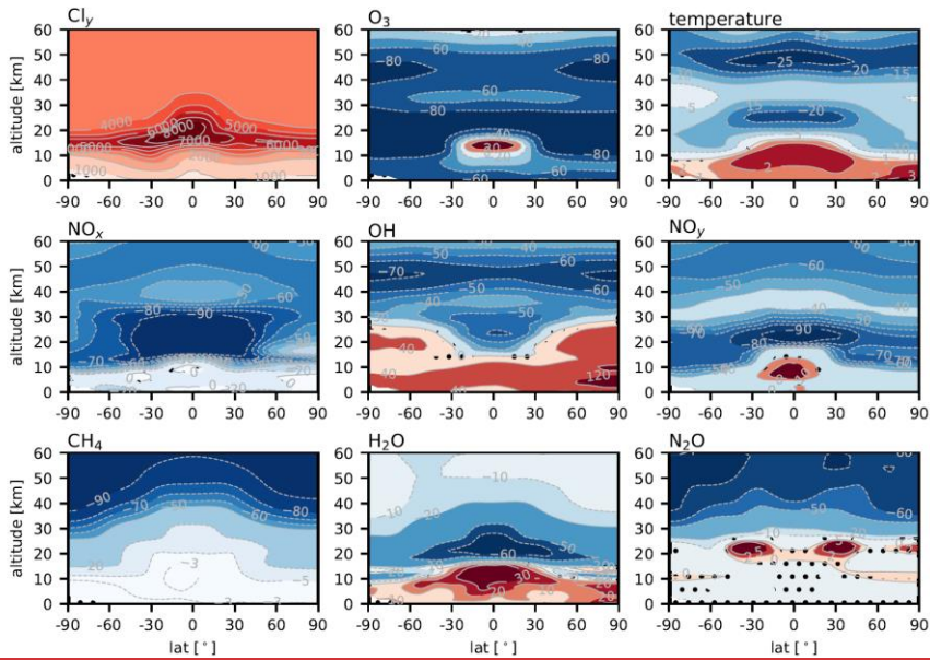
Figure 3: Zonal, annual, and ensemble mean of total inorganic chlorine ( \text{Cl}_y ), \text{O}_3 , \text{NO}_x(\text{N}+\text{NO}+\text{NO}_2) , OH, \text{H}_2\text{O} , total reactive nitrogen ( \text{NO}_y ), \text{CH}_4 , \text{H}_2\text{O} , \text{N}_2\text{O} (in %), and temperature (in K) response to the absence of the MPA regulations (noMPA relative to - MPA-ssp245) averaged over 2080–2099. All differences are statistically significantly different from zero at the 90% level except areas with black dots. The colored areas mark statistically significant results at the better than 95% level.
