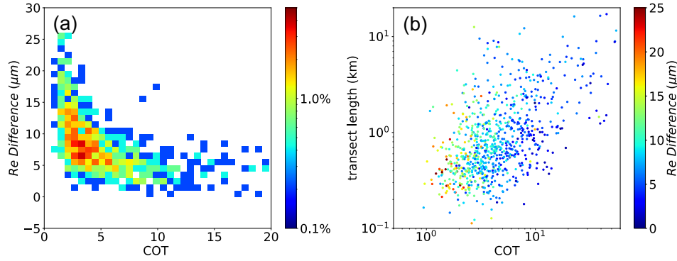
Figure 8. (a) Density plot of cloud element mean Re difference (bi-spectral – polarimetric Re ) vs. mean COT. (b) Scatter plot of Re difference (color) vs. transect length and COT using cloud element means.
