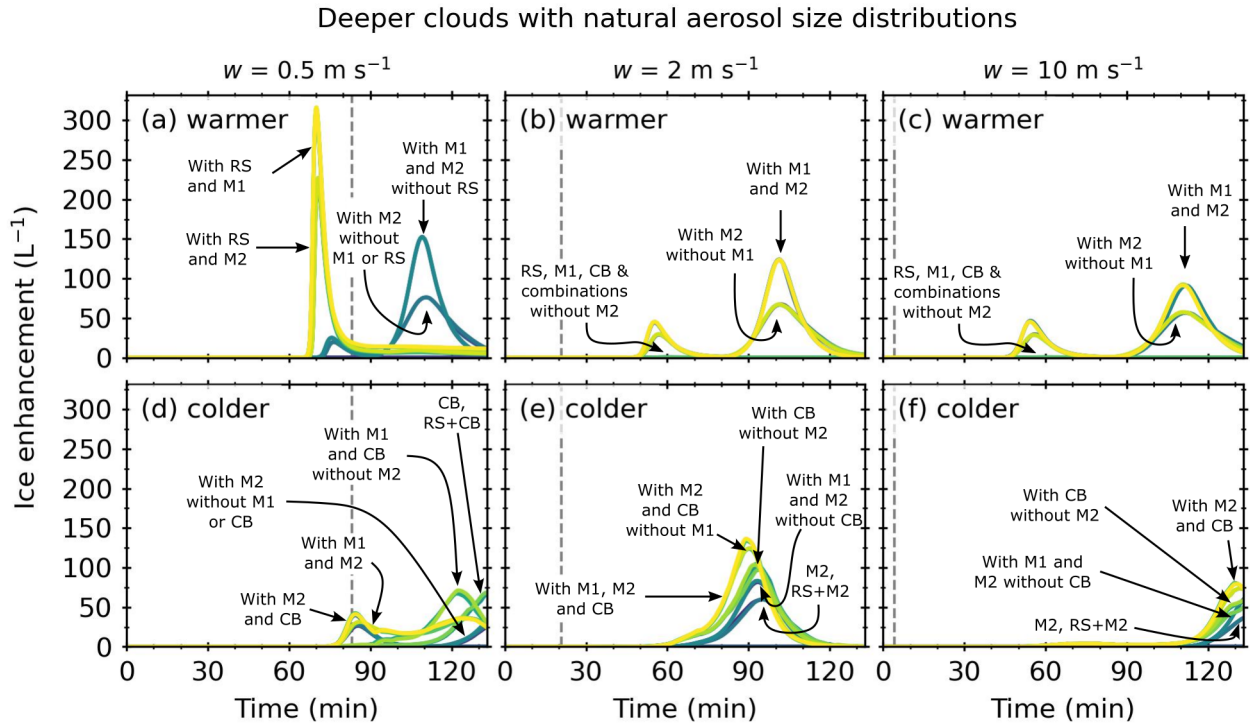
Figure 10. Ice enhancement against simulation time for a deeper (2.4 km) cloud with a natural aerosol size distribution. Warmer refers to cloud base temperatures of 7 °C, and colder refers to cloud base temperatures of 0 °C. The grey dashed lines indicated the threshold time where the updraft was turned off. Plots are annotated to indicate the processes that were active.
