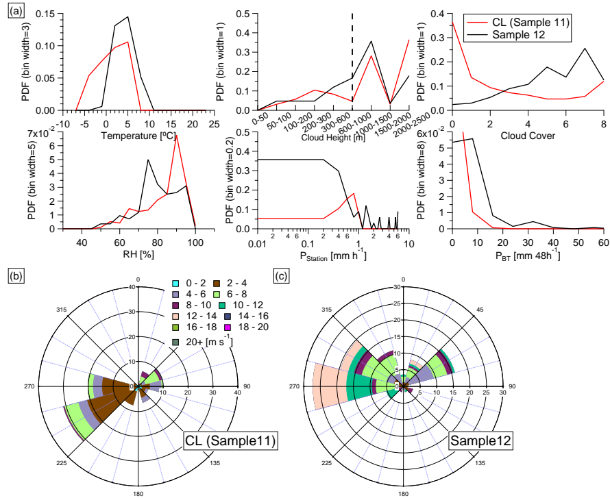
Figure 6. (a) Probability density function (PDF) of temperature, cloud height, cloud cover, RH, precipitation measured at the station ( P_{Station} ), and cumulative precipitation along the backward trajectory in the past 2 days ( P_{BT} ) during samples 11 (red) and 12 (black). The dashed line in the cloud height panel shows the measurement station height. (b) The wind rose plot during sample 11. (c) The wind rose plot during sample 12.
