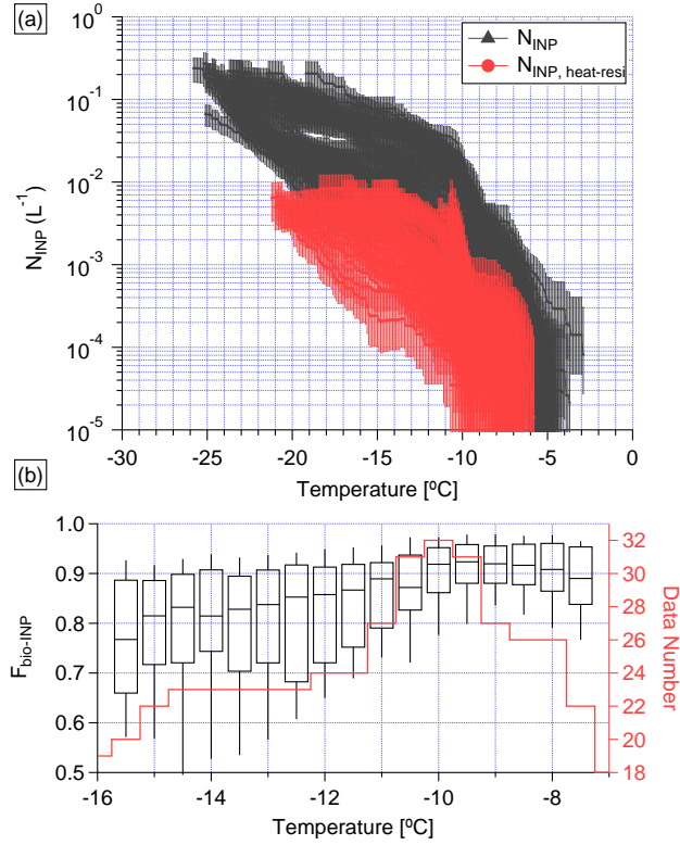
Figure 3. (a) Values for N_{\text{INP}} and N_{\text{INP,heat-resi}} as function of temperature in black triangles and red dots, respectively. (b) Boxplot of F_{\text{bio-INP}} as a function of temperature. The red line shows how many different samples contributed to the boxplot at different temperatures (relating to the right axis).
