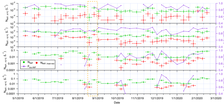
Figure 2. Time series of N_{\text{INP}} (green circles) and heat-resistant N_{\text{INP}} ( N_{\text{INP,heat-res}} , red circles) at -8 , -10 , -15 , -18 °C (from top to bottom). The fraction of bio-INP is shown as purple line. The orange box highlights samples 11 and 12, which are two samples used for a case study (discussed in Sect. 3.4).
