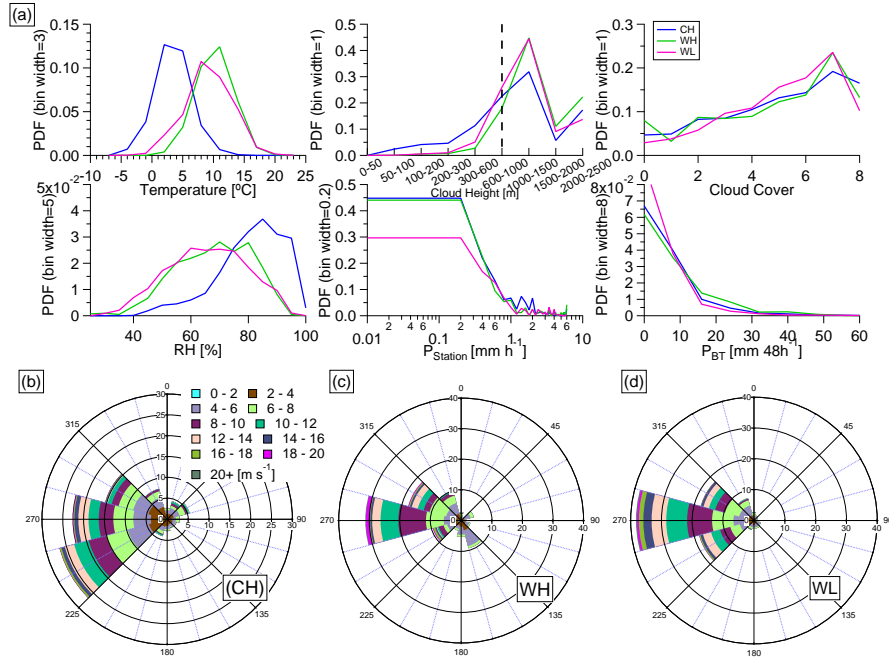
Figure 10. (a) Probability density function (PDF) of temperature, RH, cloud cover, cloud height, precipitation measured at the station ( P_{\text{Station}} ), and cumulative precipitation along the backward trajectory in the past 2 days ( P_{\text{BT}} ) averaged for all samples collected during cold season high (CH, blue lines), warm season high (WH, green lines), and warm season low (WL, magenta lines). (b, c, d) The wind rose plots for CH, WH and WL.
