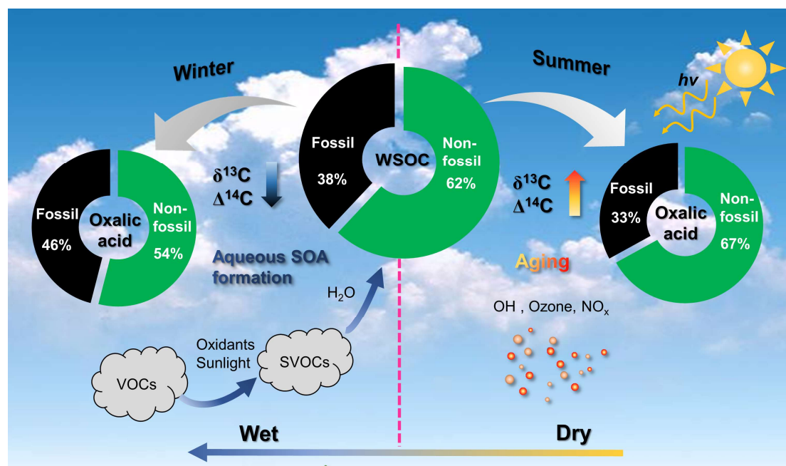
Figure 7. Schematic of the atmospheric fates of secondary organic aerosols (SOAs) in winter and summer. VOCs means volatile organic compounds, SVOCs means semi-volatile organic compounds, and WSOC means water-soluble organic carbon.
