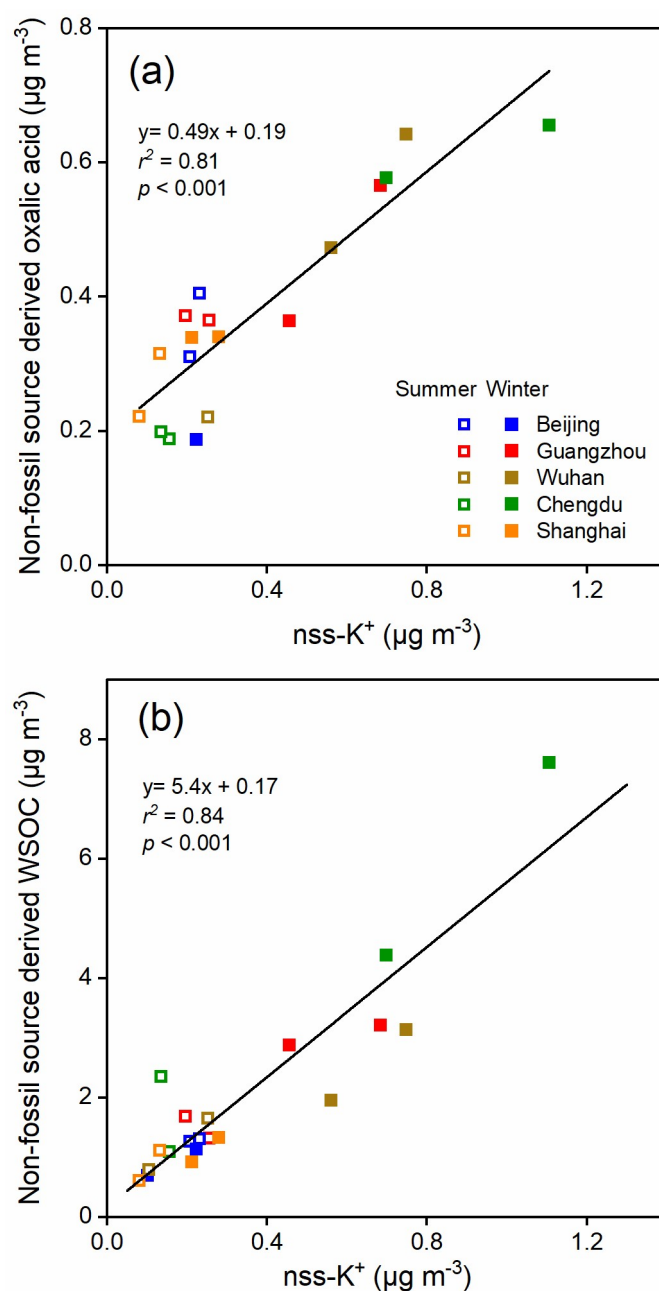
276 277 Figure 3. Relationships between (a) non-fossil-derived oxalic acid concentrations and 278 non-sea-salt potassium ( \text{nss-K}^+ ) concentrations and between (b) non-fossil-derived 279 water-soluble organic carbon (WSOC) concentrations and \text{nss-K}^+ concentrations.
