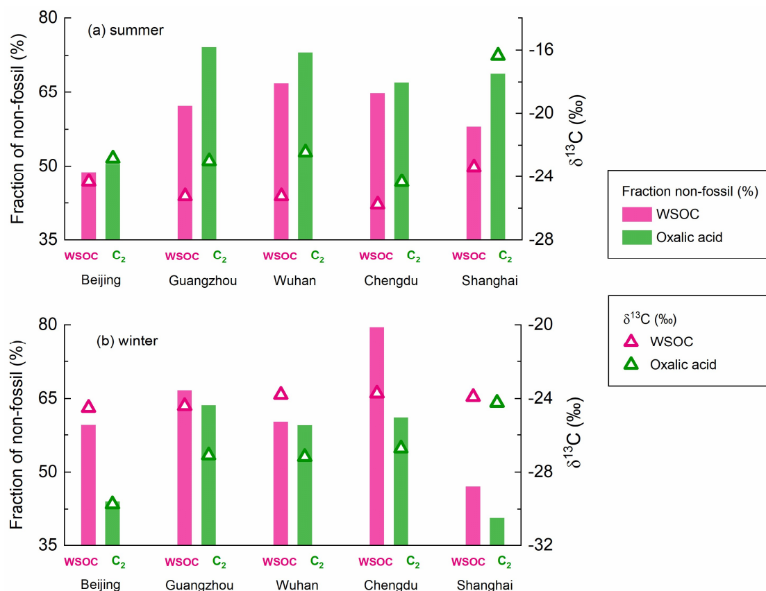
Figure 6. Proportions of non-fossil sources (determined from the ^{14}\text{C} values) and \delta^{13}\text{C} values for water-soluble organic carbon (WSOC) and oxalic acid (C 2 ) in Beijing, Guangzhou, Wuhan, Chengdu, and Shanghai in (a) summer and (b) winter.
