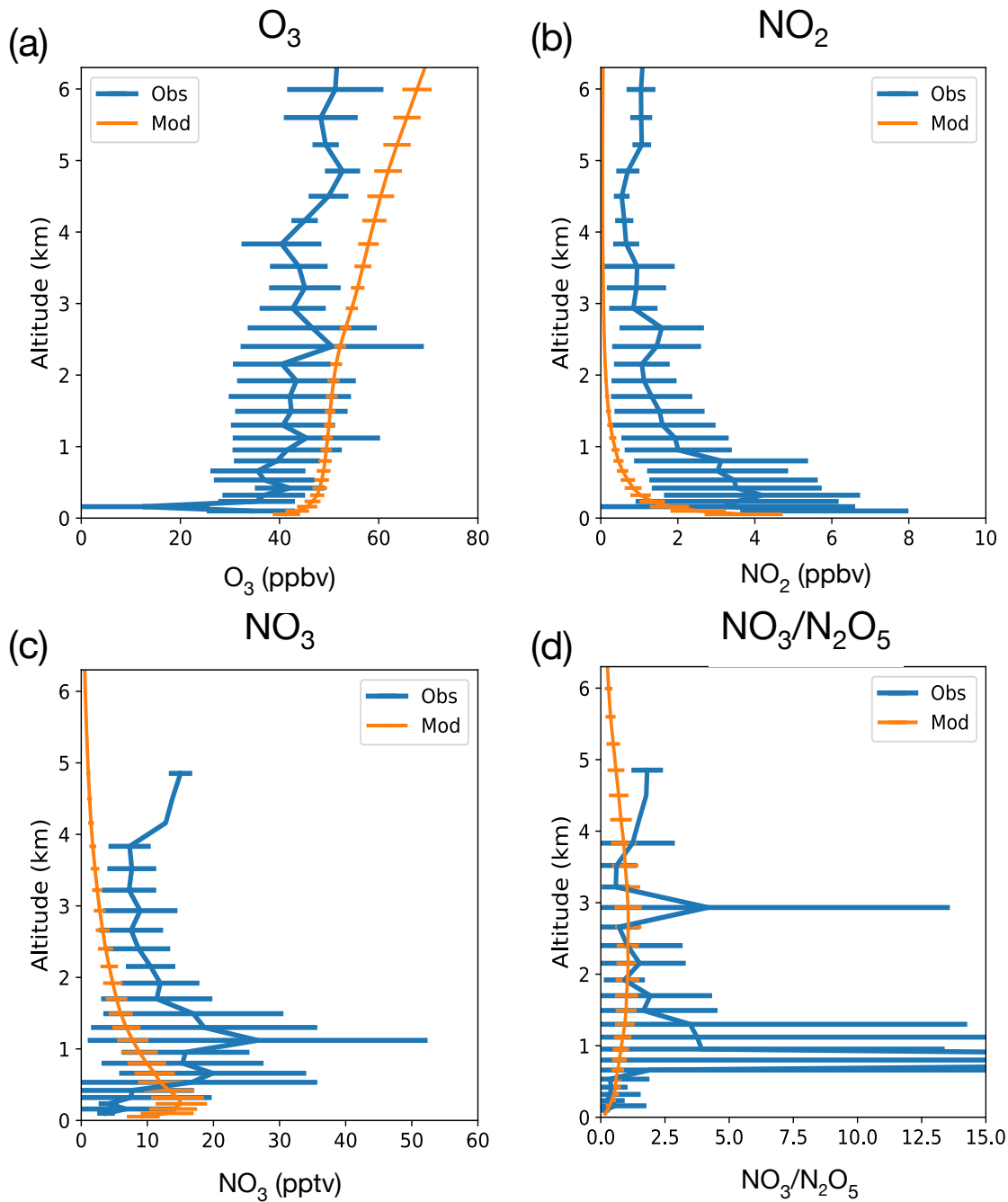
Figure 1. Comparison of vertical profile of night-time concentrations of O 3 (a), NO 2 (b), NO 3 (c) and NO 3 :N 2 O 5 ratio (d) between RONOCO July 2010 flight campaign and 2010-2014 July nighttime values from UKESM1 model simulations from grid cells corresponding to flight regions. Lines show means and error bars show standard deviation.
