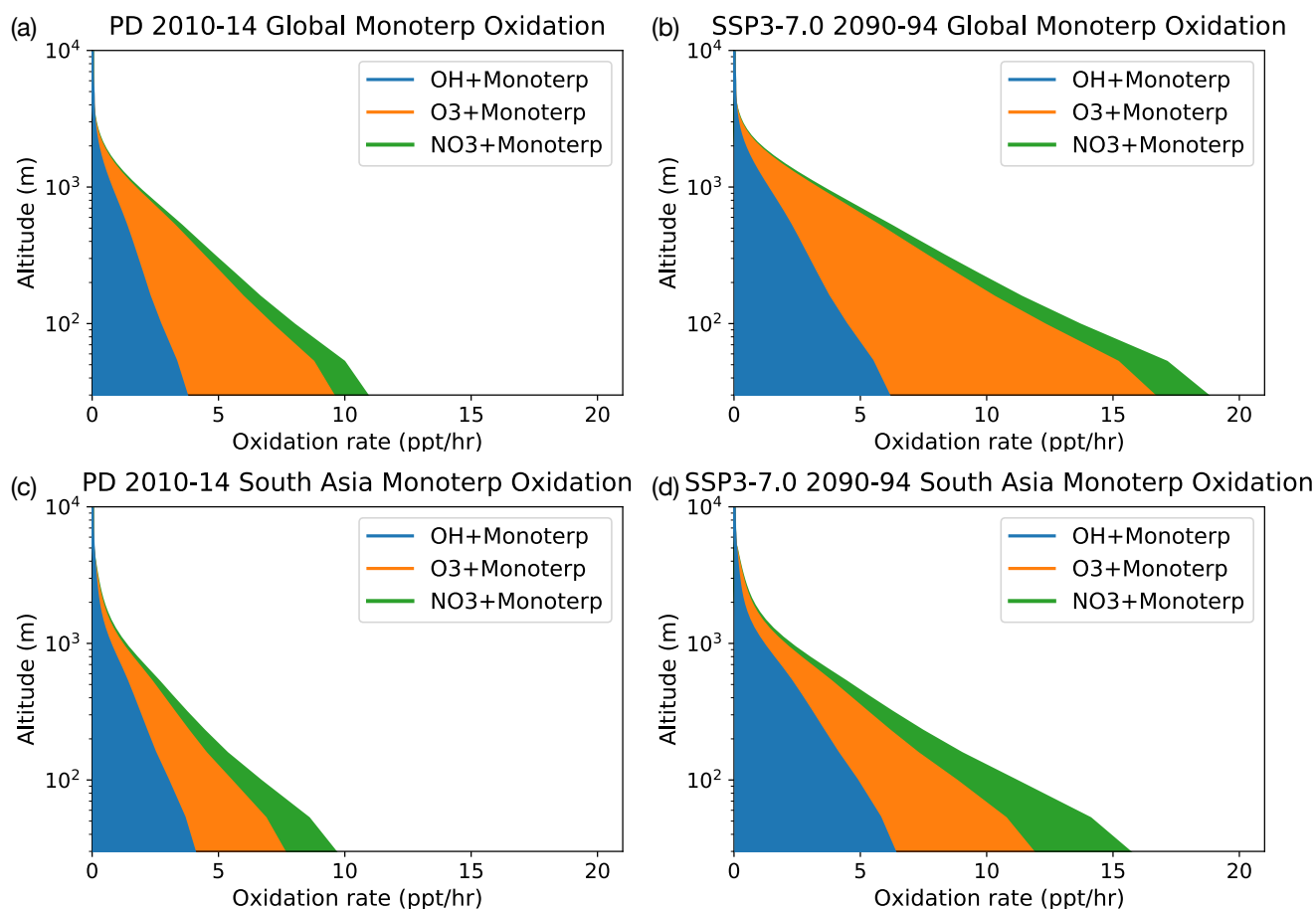
300 Fig. 5. Vertical profile of MONOTERP oxidation via OH, O 3 and NO 3 . Panels (a) and (c) show the model calculated present day global and South Asian oxidation fluxes respectively. Panels (b) and (d) show these fluxes at the end of the 21 st Century under the SSP3-7.0 scenario. The future scenario results in increases in all oxidation fluxes, with the NO 3 initiated oxidation flux increasing by a factor of 2 compared with the present day oxidation rates in South Asia.
