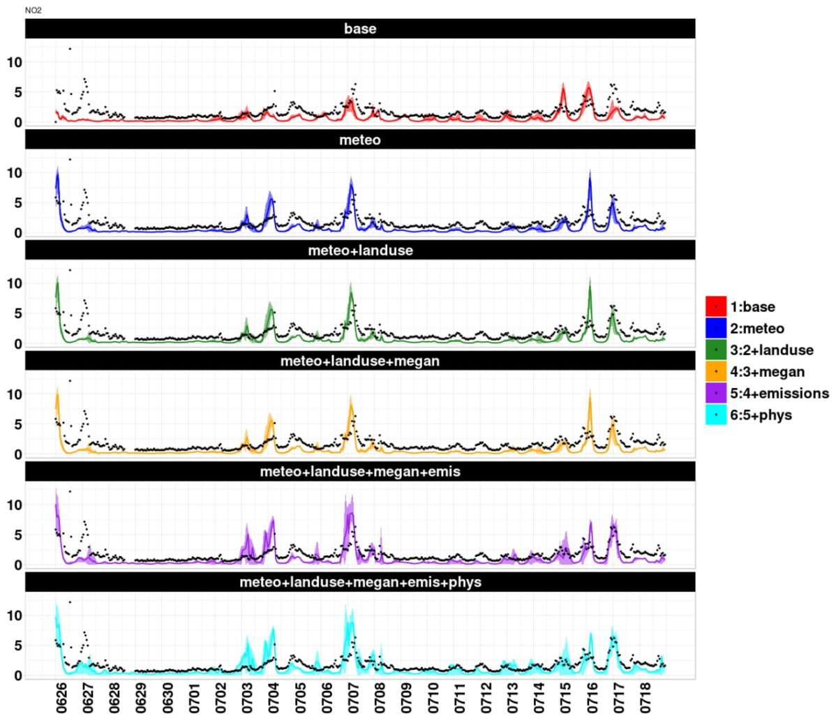
Figure S15 : Comparisons for NO 2 . All values are shown in ppb.
