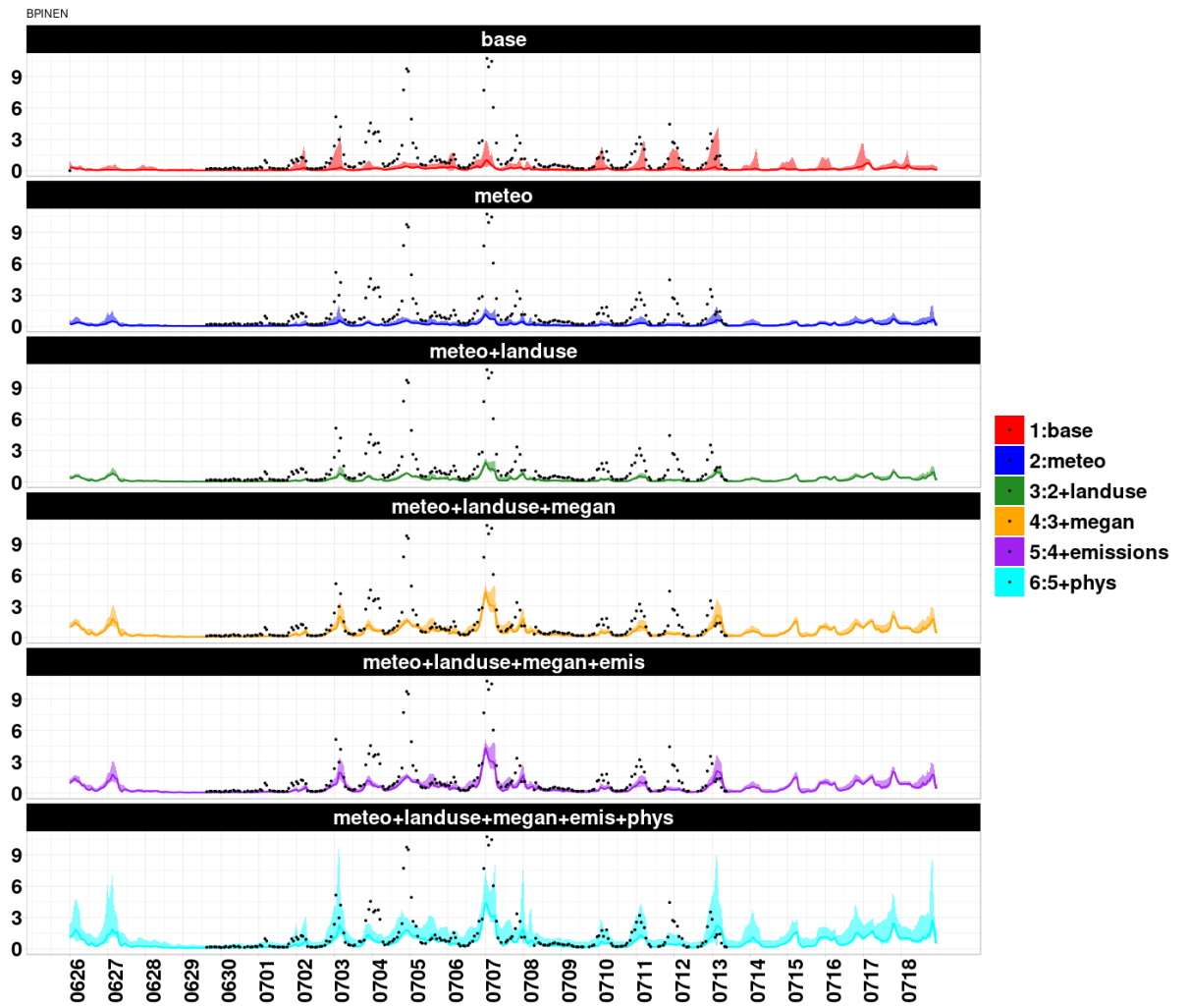
Figure S17: Comparisons for b -pinene, all data is shown in ppb.
