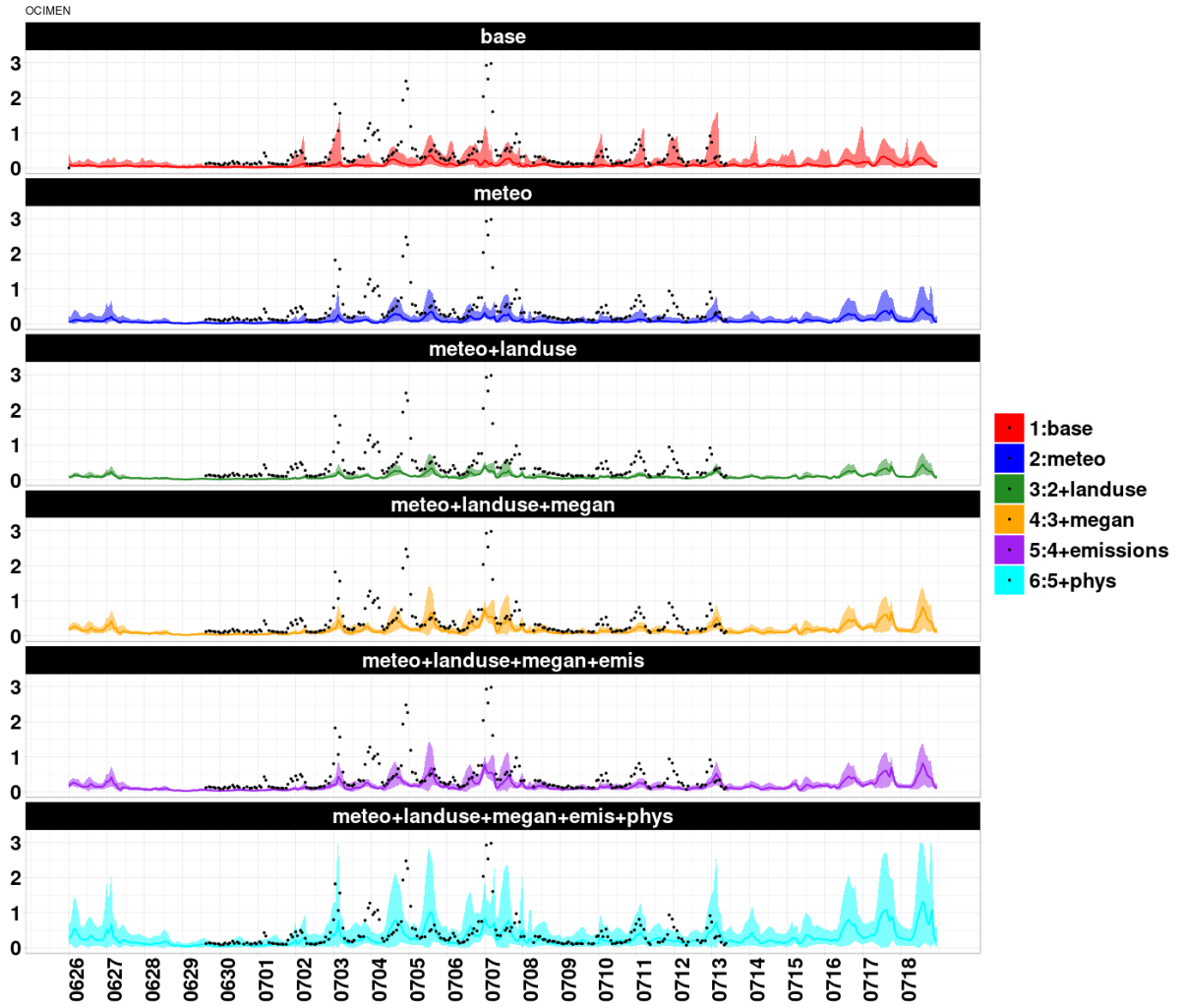
Figure S110: Comparisons for the sum of ocimene and myrcene, all data is shown in ppb.
