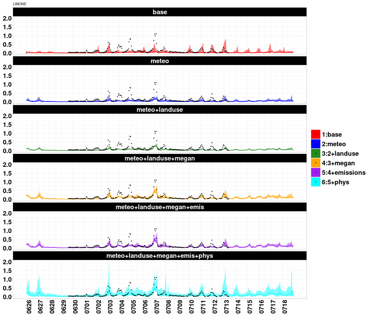
Figure S19: Comparisons for limonene, all data is shown in ppb.
