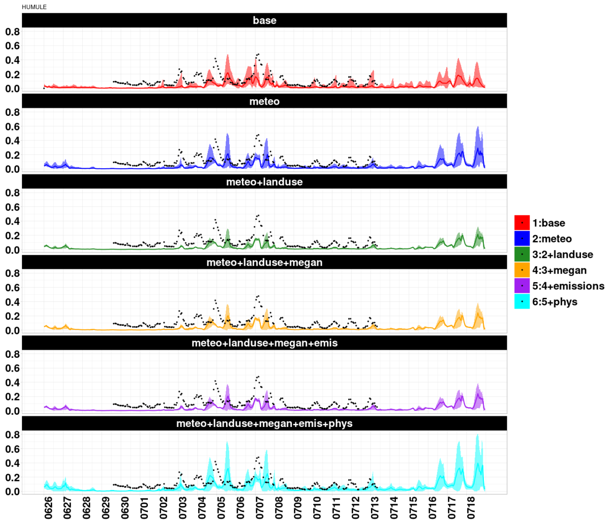
Figure S18: Comparisons for humulene, all data is shown in ppb.
