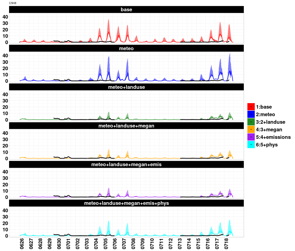
Figure S111: Comparisons for isoprene, all data is shown in ppb.
