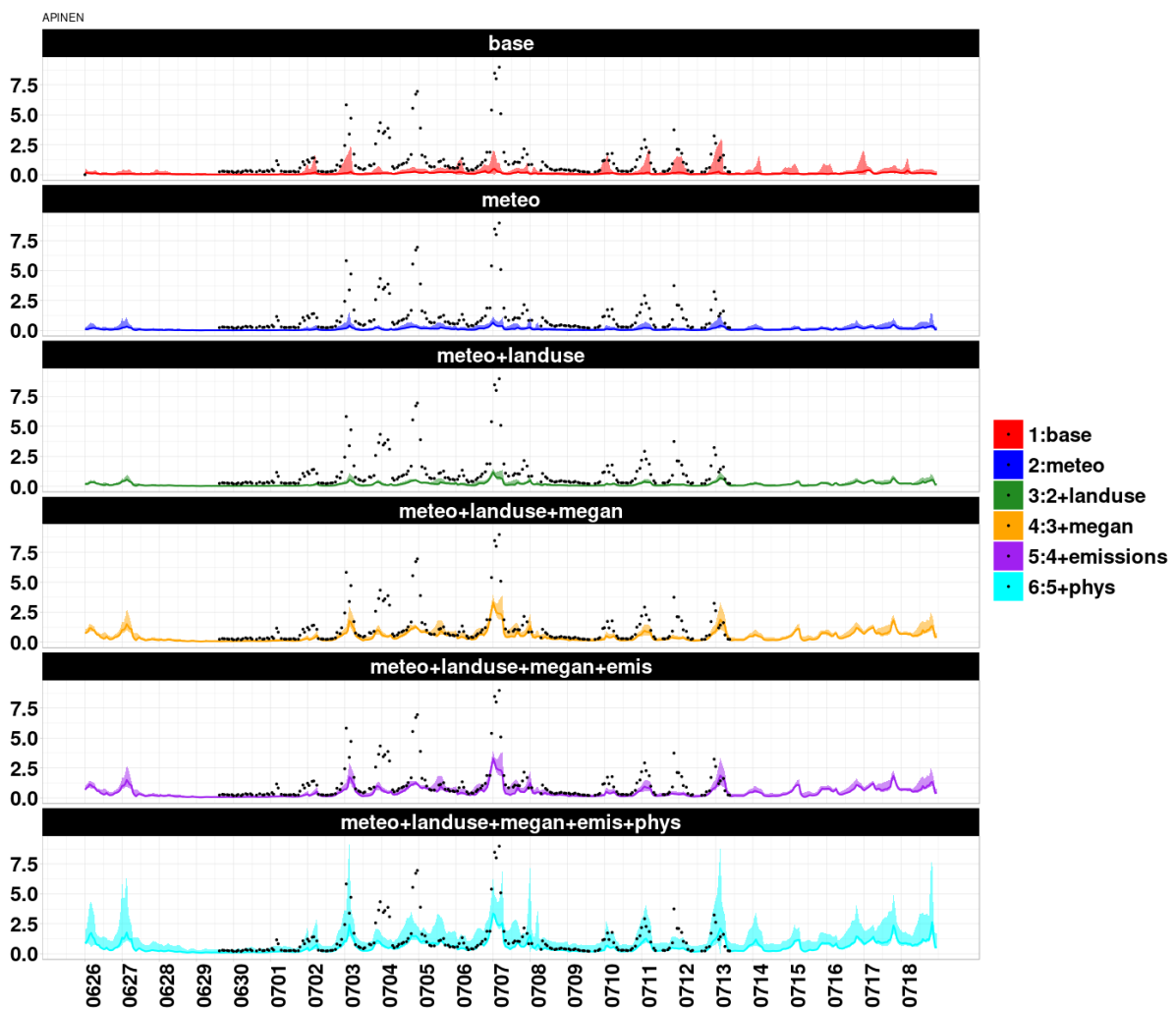
Figure SI6: Comparisons for \alpha -pinene, all data is shown in ppb.
