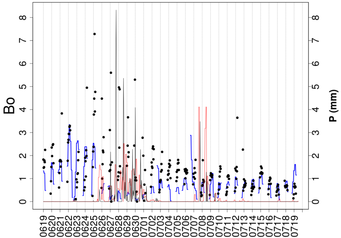
Figure SI2: Bowen ratio (left axis) and precipitation comparisons for the Bilos site. Precipitation (red for model, black lines for observations) and Bowen ratio (blue for model and black dots for observations) are shown here.
