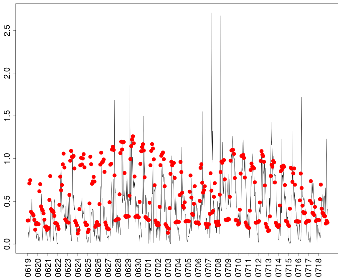
Figure S13 : Deposition speed (m/s) comparisons for ozone : black lines show the measurements and red dots simulations. The temporal resolution for the measurements is hourly, while simulations have a bi-hourly frequency.
