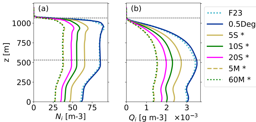
Figure 10. Profiles averaged over the domain and the simulation period of 8–12 hours: (a) N_i , (b) Q_i . One F23 run in dotted cyan (see dotted line in Fig. 9), 0.5Deg in blue, 5S in yellow solid, 10S in green solid, 20S in magenta solid, 5M in yellow dashed, 60M in green dotted. Simulations with significant differences to F23 are indicated with an asterisk. Horizontal dashed lines indicate the cloud’s top and bottom in F23.
