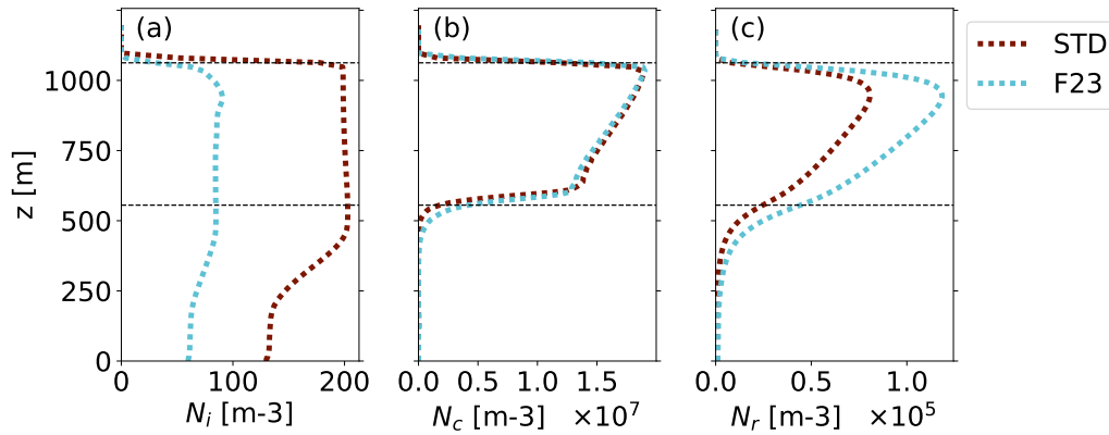
Figure C1. Profiles averaged over the domain and the simulation period of 8–12 hours: (a) N_i , (b) N_c and (c) N_r . One STD in red dotted, and one F23 run in cyan dotted (see dotted lines in Fig. 3). Horizontal dashed lines indicate the cloud’s top and bottom in STD.
