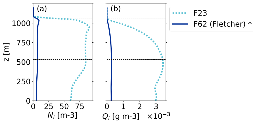
Figure D1. Profiles averaged over the domain and the simulation period of 8–12 hours: (a) N_i , (b) Q_i . The F23 comparison run is plotted in dotted cyan (see dotted line in Fig. 3), and one run with F62 in blue. Simulations with significant differences to F23 are indicated with an asterisk (tested with a two-sided t-test at the 95 % level). Horizontal dashed lines indicate the cloud’s top and bottom in F23.
