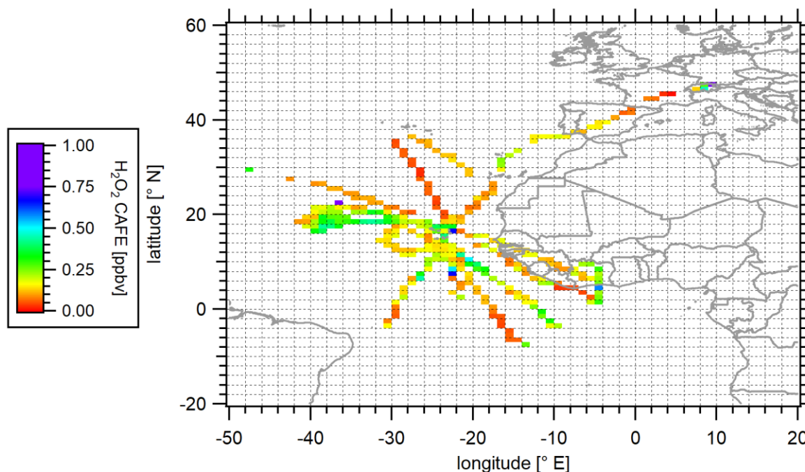
240 Figure 2. Spatial distribution of measured hydrogen peroxide in the upper troposphere ( \geq 8 km) during the CAFE-Africa campaign. Data were binned into 1^\circ \times 1^\circ bins over the full extension of the flight tracks.
