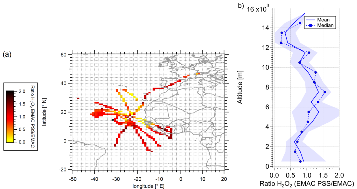
Figure S8. Spatial distribution of \text{H}_2\text{O}_2(\text{PSS EMAC})/\text{H}_2\text{O}_2(\text{EMAC}) ratio (a) and the corresponding vertical profile (b) in the upper troposphere ( \geq 8 km) during CAFE-Africa campaign. For the purposes of the spatial distribution analysis, data were binned into 1^\circ \times 1^\circ bins over the full extension of the flight tracks. The vertical distribution was estimated within 1000 m altitude bins over the entire probed column based on the simulated data within the region of the base of operation in Sal, Cape Verde (approx. 16^\circ 35' - 16^\circ 51' \text{ N} ; -22^\circ 52' - -23^\circ \text{ E} ).
