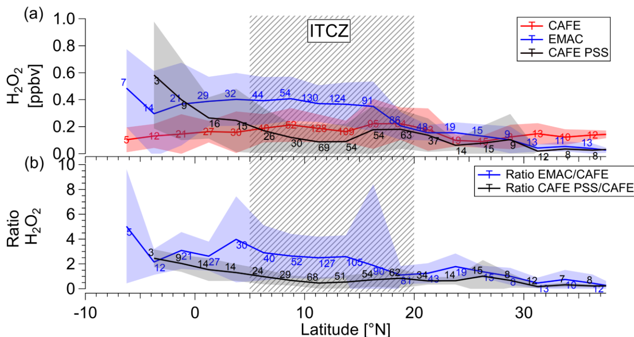
350 Figure 5. Latitudinal dependence of hydrogen peroxide mixing ratios (mean \pm 1\sigma ) compared to EMAC simulations and calculations based on PSS (red: CAFE-Africa; black: PSS CAFE-Africa; blue: EMAC; a) and calculated ratios between the simulations and the observations and PSS-modelled calculations, and the observations, respectively (b). The data with 6 min time resolution and mean values was binned for 2.5^\circ of latitude for altitudes \geq 8 km. The corresponding numbers indicate the total amount of data points per bin. The shaded pattern marks the ITCZ region.
