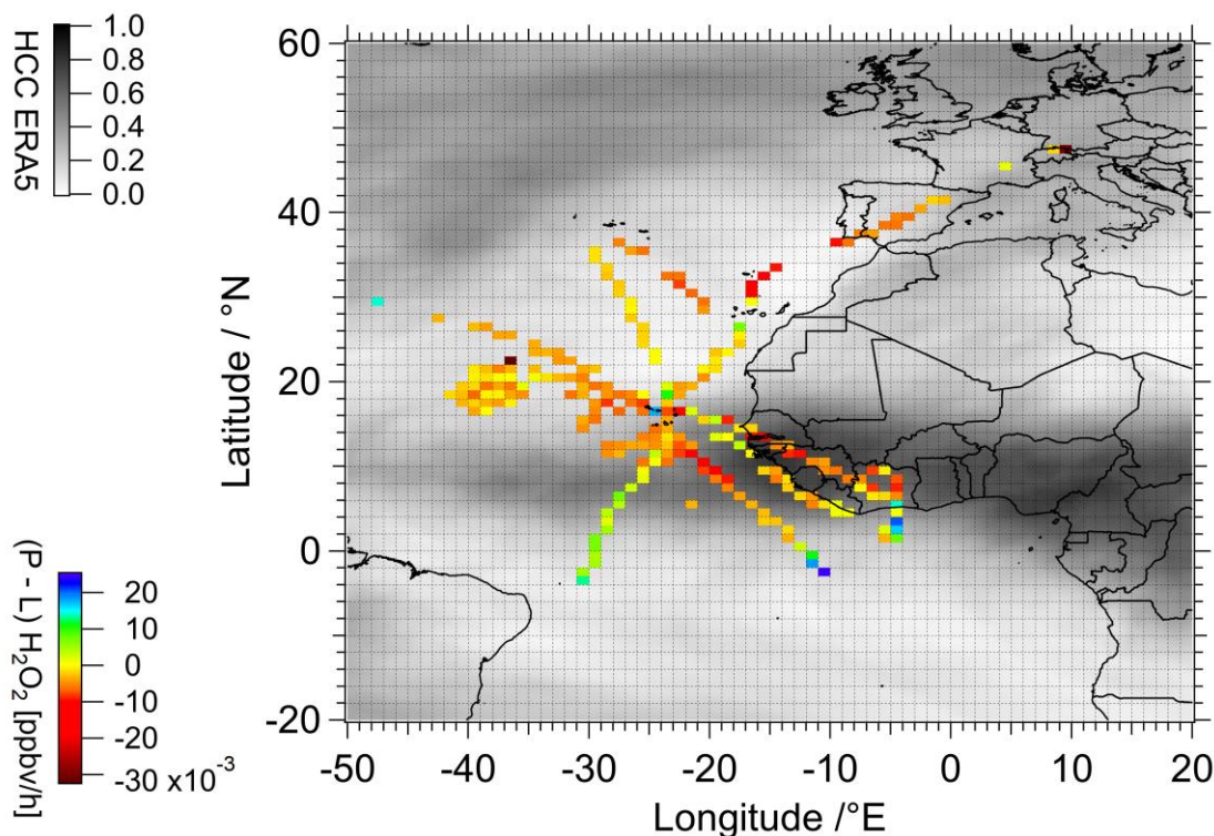
325 Figure 4. Color-coded spatial resolution of calculated deviation from PSS based on the difference between the observed hydrogen peroxide photochemical production and loss. The calculated data were binned into 1^\circ \times 1^\circ bins over the full extension of the flight tracks. Shaded background is the average high cloud coverage ( \geq 6 km) during the measurement period based on ERA5 reanalysis results (HCC; Hersbach et al., 2019).
