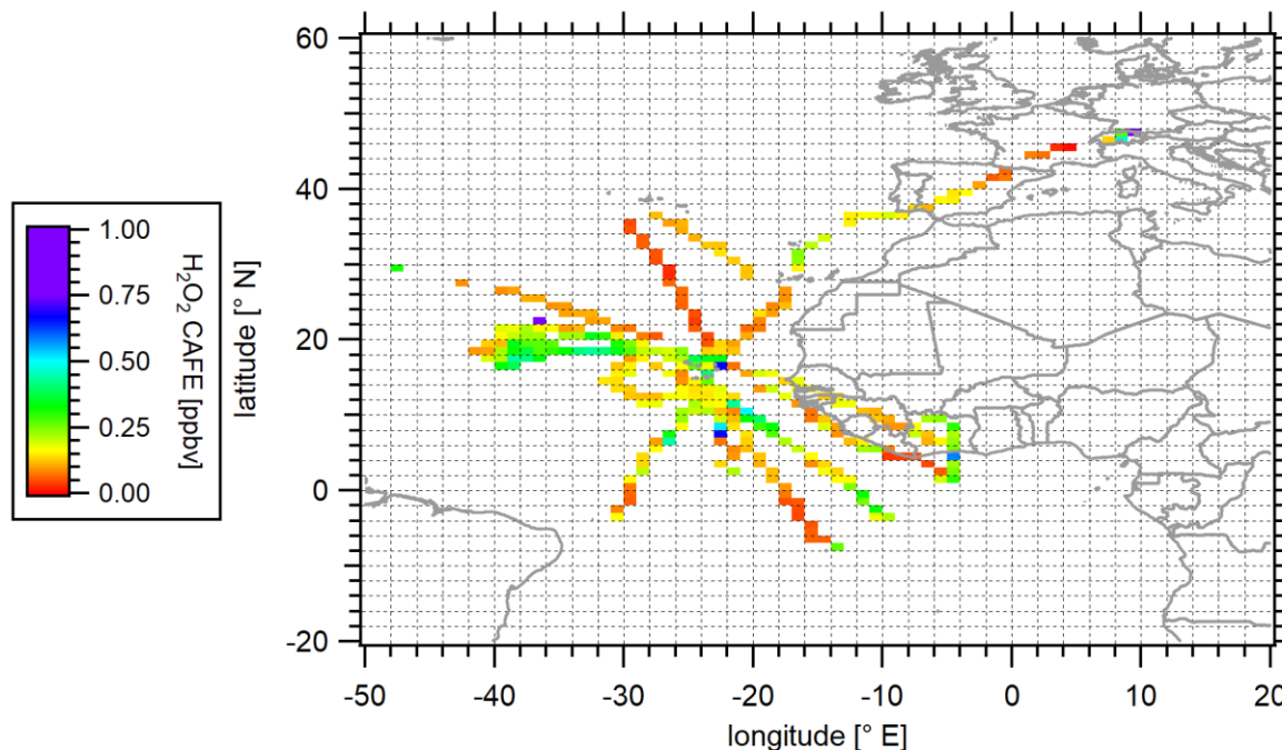
255 Figure 2. Spatial distribution of measured hydrogen peroxide in the upper troposphere ( \geq 8 km) during the CAFE-Africa campaign. Data were binned into 1^\circ \times 1^\circ bins over the full extension of the flight tracks.
