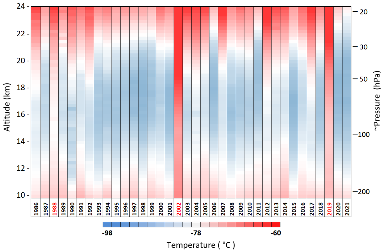
Figure 9. The average temperature during 24 September to 15 October (ozone hole minimum period over South Pole Station). The blue to red transition temperature falls at -78^{\circ}\text{C} , to highlight the polar stratospheric cloud formation threshold temperature.
