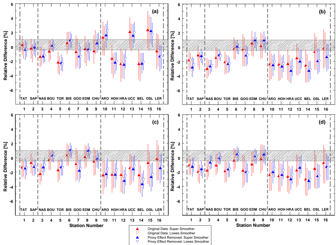
Fig. A1. The same as Fig. 4 but for the ozone recovery index, \text{ORI}_1(1997, 2020) , based on the \text{TCO}_3 monthly means averaged over the entire year (January--December).
