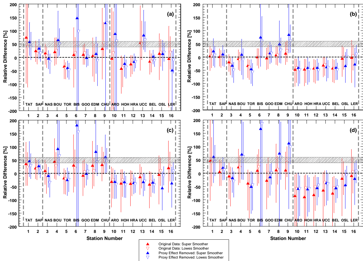
Fig. 5. The same as Fig. The TCO 3 recovery faster than in the ESSC pattern only occurs at one station (Bismark). It can be found using ORI_1(2020) from all original datasets except MOD. In addition, there is a faster recovery for the ozone recovery index, ORI_2(1997, 2020) , based on Eq. (2). The reference range (hatched area) is between 40 % and 60 % according estimates in Sect. 3.4.
