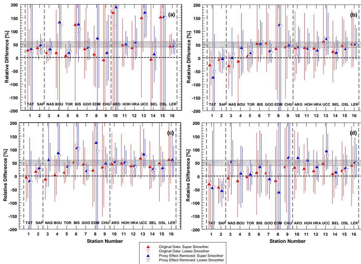
Fig. A4. The same as Fig. A3 but for the ozone recovery index, ORI_2(1997, 2020) .
