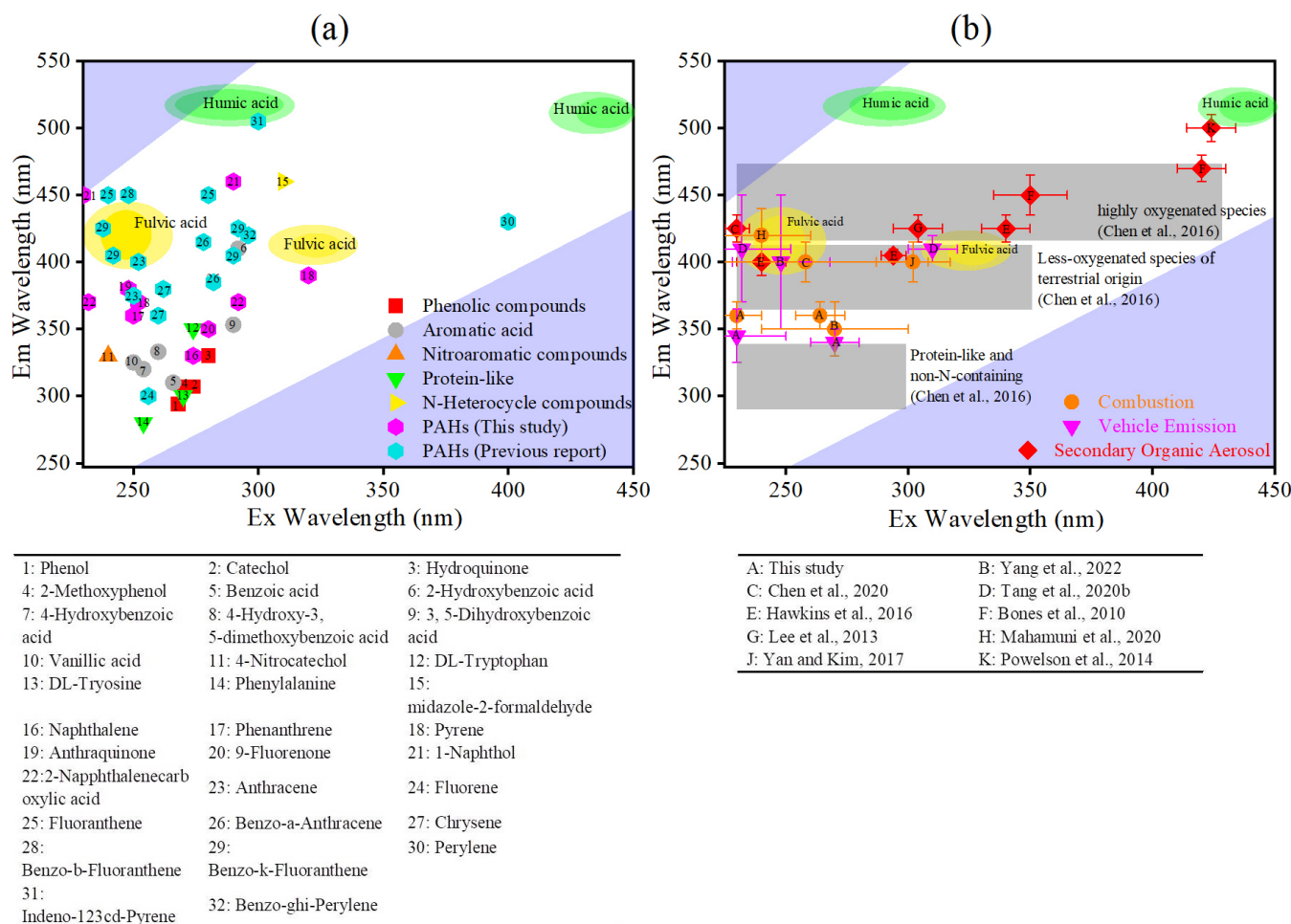
Figure 1. Comparison of the chemical characteristics of molecules assigned to each fluorescence component of BrC model compounds (a) and source WSOM (b).
