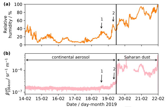
Figure A1. (a) Relative humidity observed during the comparison period (14–22 February 2019) on 19 February 2019 at WFJ (mountaintop site). The two peaks in relative humidity during the transition time are indicated with 1 and 2. (b) Observed lidar attenuated backscatter coefficient \beta_{1064\text{nm}}^{\text{att}} at the height of WFJ (2687 m a.s.l.). The two characteristic time periods for continental background aerosol and Saharan dust are indicated. Two perturbations in \beta_{1064\text{nm}}^{\text{att}} during the transition time are indicated with 1 and 2, respectively.
