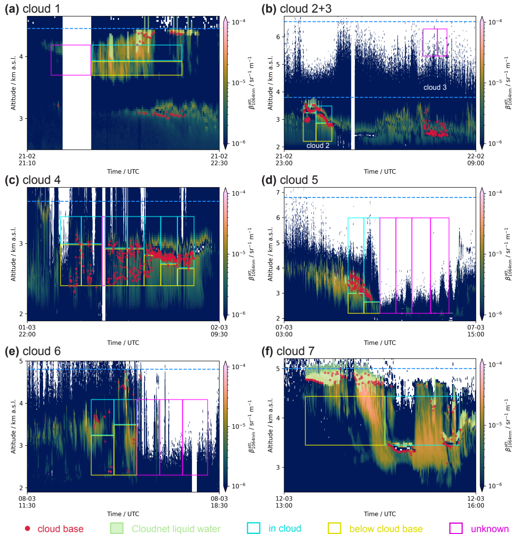
Figure C1. Time slicing and classification of the ICNC-ice crystal number concentration data indicated in Figure B1 (red rectangle encompasses rectangles presented in this plot). White background represents regions where the lidar was either fully attenuated or the instrument underwent automatic maintenance. The attenuated backscatter coefficient at 1064 nm ( \beta_{1064\text{nm}}^{\text{att}} ) is presented in the background. A (liquid) cloud base estimate derived from the attenuated backscatter coefficient at 532 nm ( \beta_{532\text{nm}}^{\text{att}} ) is indicated by red circles. The automated liquid water classification by the Cloudnet algorithm is presented by lime tiles. Empty rectangles in cyan, yellow, and magenta indicate regions classified as above cloud base, below cloud base, and unknown cloud base, respectively. Cloud top derived from radar observations (Figure B1) is indicated by the dashed blue line. The dotted lightblue line in (d) indicates the height above which homogeneous freezing is possible ( T < -38 °C).
