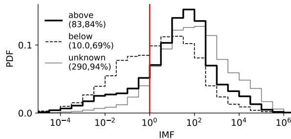
Figure 11. Probability density functions (PDFs) of obtained IMFs-ice multiplication factors (IMFs, Equation 12) for ICNC-ice crystal number concentration data above cloud base (solid black), below cloud base (dashed black), and of unknown cloud base (solid gray). The solid red line indicates unity. The median IMF and the percentage of IMF larger unity for each PDF are given in the legend.
