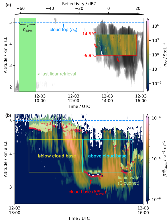
Figure 9. Exemplary illustration of data processing workflow to obtain in cloud ice multiplication factors (IMFs) for the cloud observed on 12 March 2019. (a) Reflectivity of the cloud radar is given in shades of gray. ICNC-Ice crystal number concentration ( n_{ice} ) is overlaid in color. The limit of used data for the IMF calculation with height is indicated in red (height span h_d , time span t_d ). Additionally, the ambient temperature at the heights of the upper and lower bound of selected data is given in red (see T_{dt} and T_{db} in Table D1). The INP concentration ( n_{INP,ct} ) was taken from the last lidar retrieval (solid green shading) at cloud top (dashed blue line). (b) Attenuated backscatter coefficient at 1064 nm ( \beta_{1064\text{nm}}^{\text{att.}} ) from the lidar in color. Cloud base estimates determined from the attenuated backscatter coefficient at 532 nm ( \beta_{532\text{nm}}^{\text{att.}} ) are indicated by red dots. Regions where the Cloudnet algorithm detected liquid water are indicated in bright green. The height of cloud top is indicated by the dashed blue line. The region within the yellow rectangle was classified as below cloud base and the region within the cyan rectangle as above cloud base, respectively. Overviews of all individual cloud events can be found in Figures B1 and C1.
