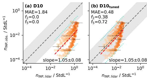
Figure 7. Same as for Figure 4 but comparing in situ INP concentrations ( n_{\text{INP,obs.}} ) measured at WFJ ( mountaintop site, Figure 1 ) to lidar-retrieved INP concentrations ( n_{\text{INP,lidar}} ) using (a) the standard D10 parameterization and (b) the tuned D10 parameterization (see Equation 11) for continental aerosol. Note that (a) is the same as Figure 5a.
