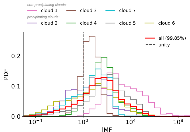
Figure D1. Probability density functions (PDFs) of obtained IMFs-ice multiplication factors (IMFs, Equation 12) for each of the seven observed clouds and all IMFs combined (thick solid red) using all ICNC-ice crystal number concentration data (not only above cloud base). The dashed black line indicates unity. The median IMF and the percentage of IMF larger than unity for the combined histogram are given in the legend.
