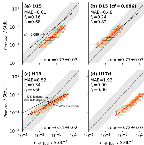
Figure 4. Comparison of in situ INP concentrations ( n_{\text{INP,obs.}} ) measured at WFJ ( mountaintop site, Figure 1 ) to lidar-retrieved INP concentrations ( n_{\text{INP,lidar}} ) during the Saharan dust event (19–21 February 2019) for three dust parameterizations: (a) D15 (DeMott et al., 2015), (b) D15 with a calibration factor ( cf = 0.086 ) applied as proposed by Schrod et al. (2017), (c) H19 (Harrison et al., 2019), and (d) U17d (Ullrich et al., 2017). Notably, we compare INP concentrations at temperatures between -20 °C (dark orange) and -5 °C (light orange). The 1:1 line is shown in dashed gray. The dashed red lines show a linear regression fit through the logarithmically transformed data points, including the 95 % confidence interval in dotted cyan. Shown in every panel are the mean absolute error (MAE), the fraction of data points falling within a factor of two and five with respect to the 1:1 line ( f_2 and f_5 ), and the slope of the fit (including the standard error). The gray shaded area indicates a deviation of one order of magnitude from the 1:1 line which is the upper limit uncertainty of the lidar based INP retrieval (Mamouri and Ansmann, 2016). For D15 (a), the data fit is also presented applying the calibration factor from (b) for comparison (black dashed). For H19 (c), the data fit is also presented assuming a K-feldspar fraction of 10 % (black dashed) and 1 % (black dotted), respectively. Uncertainties in INP concentration are indicated for representative samples in blue.
