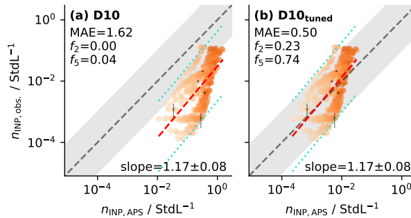
Figure 6. Same as for Figure 5a but comparing in situ INP concentrations ( n_{\text{INP,obs.}} ) measured at WFJ ( mountaintop site, Figure 1 ) to predicted INP concentrations ( n_{\text{INP,APS}} ) based on D10 now applied to in situ aerosol concentrations (from APS) during continental background (cf. Figure 3). (a) D10 applied to in situ aerosol concentrations (from APS) in its standard form. (b) D10 shifted towards the 1:1 line maximizing the fraction of data points within one order of magnitude around the 1:1 line (cf. Equation 11).
