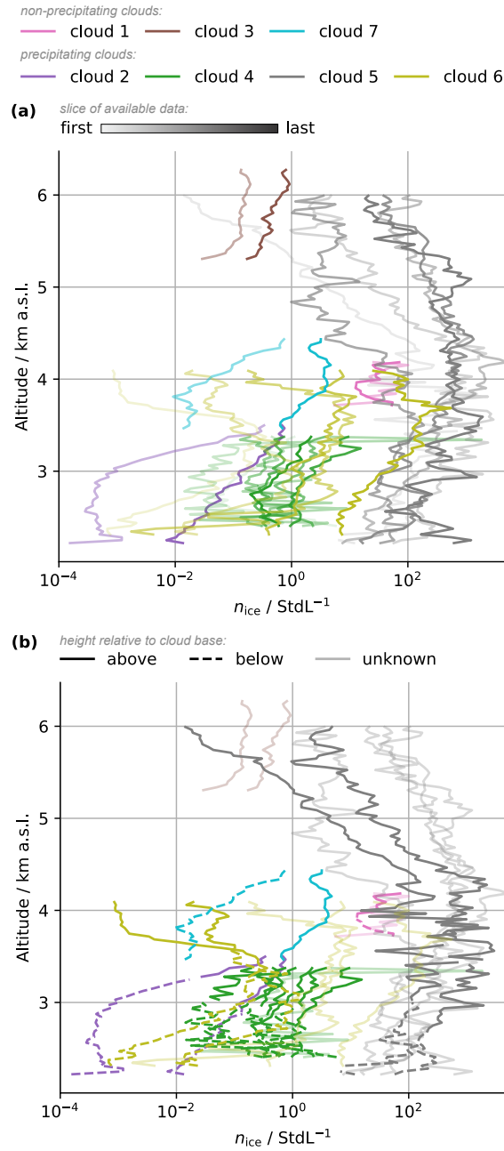
Figure 10. Median ice crystal number concentrations (ICNCs) as a function of altitude for each cloud and for time slices of approximately one hour. (a) Temporal evolution of the ICNC ( n_{ice} ) profiles: Faintest colors correspond to the first slice of data and the strongest colors correspond to the last slice of data. (b) Cloud regime classification for each time slice: ICNCs ( n_{ice} ) taken above cloud base (solid), below cloud base (dashed) and unknown cloud base (faint color). For cloud 3, the cloud base could not be determined.
