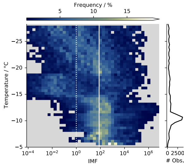
Figure 13. As for Figure 12, but with the height altitude converted to temperature using data from the COSMO-1 analysis.
