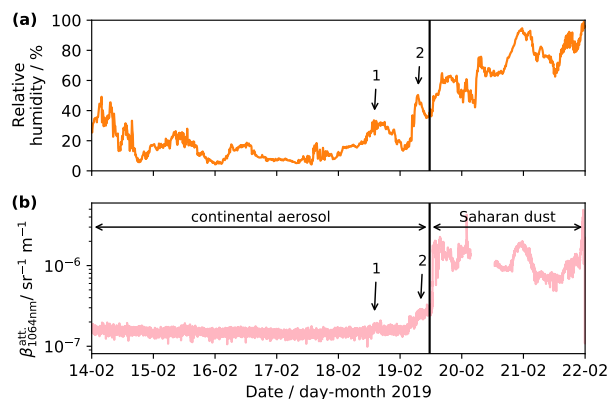
Figure A1. (a) relative humidity observed during the comparison period (14–22 February 2019) on 19 February 2019 at WFJ ( mountaintop site ). The two peaks in relative humidity during the transition time are indicated with 1 and 2, respectively. (b) observed lidar attenuated backscatter coefficient \beta_{1064\text{nm}}^{\text{att}} at the height of WFJ (2687 m a.s.l.). The two characteristic time periods for continental background aerosol and Saharan dust are indicated. Two perturbations in \beta_{1064\text{nm}}^{\text{att}} during the transition time are indicated with 1 and 2, respectively.
