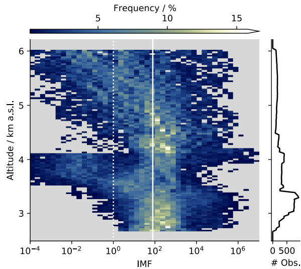
Figure 12. Frequency histogram of all observed IMF-ice multiplication factors (IMFs) above cloud base combined with height/altitude . Frequencies are normalized to the number of observations (right axis) per height bin. Gray background indicates where no ICNC-ice crystal number concentration data was observed. The dashed white line indicates an IMF of unity. The median IMF of all data is indicated in solid white.
