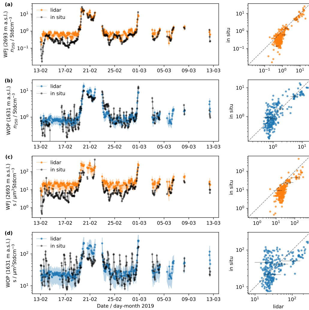
Figure 2. Comparison of aerosol properties observed in situ and with lidar. (a) Time series of aerosol number concentration with a-radius larger than radii \geq 250 nm ( n_{250} ) measured in situ (black) and with lidar (orange) at WFJ. (b) Same as (a) but measured at WOP (lidar data in blue). (c) Time series of surface area concentration ( s ) measured in situ (black) and with lidar (orange) at WFJ. (d) Same as (c) but measured at WOP (lidar data in blue). Right of each time series panel a scatter plot compares the in situ to the lidar observations of the data presented on the left. Uncertainties are indicated by the shading for the time series and at representative data points of the scatter plots in black. Note: The lidar retrieval height at WOP was 2052 m a.s.l. (see Figure 1).
