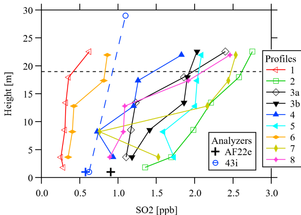
Figure 6: Measurements of SO 2 mixing ratio with height. Profile numbers correspond to those listed in Table 1. Open symbols are profiles measured at YAJP. Closed symbols are profiles measured at site 1004. Circle (○) plot markers (blue with dashed line) show average measurements of two 43i instruments over a period coincident with Profile 4. Plus (+) plot markers show average measurement of AF22e instrument over two periods coincident with Profiles 3a and 3b (black) and Profile 4 (blue). The approximate canopy height is shown as a dashed horizontal line.
