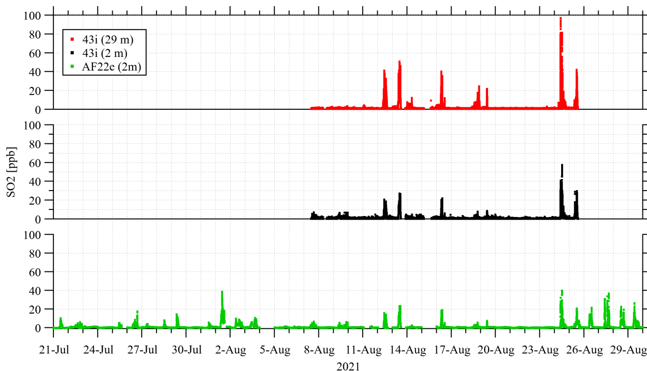
Figure 3: SO 2 measurements from gas analyzers at YAJP tower. 43i measurements are every 5-sec, AF22e are every minute.
