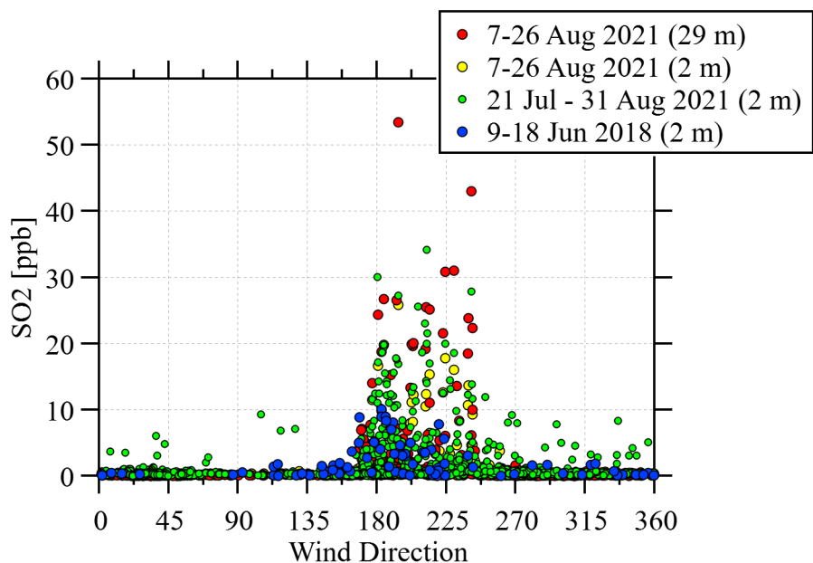
Figure 4: SO 2 measurements as a function of wind direction. Green dots are AF22e measurements. All others are 43i measurements. All measurements here are 30-min averages.
