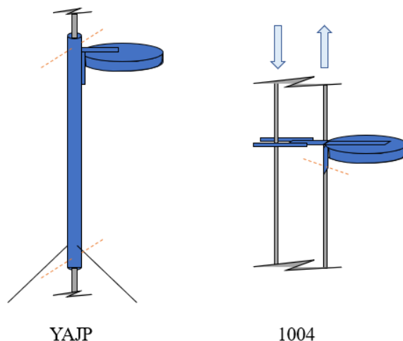
485 Figure 1: Schematic of passive sampler mounts (not to scale). Grey lines indicate pulley rope (YAJP) or pulley cable loop (1004). Orange dashed lines show where the system is fixed against the rope or cable. The YAJP system used guy ropes and the 1004 system used a tong or forked support against the looped pulley cable to inhibit rotation. Multiple passive samplers were fixed to the underside of the rain shelter lids.
