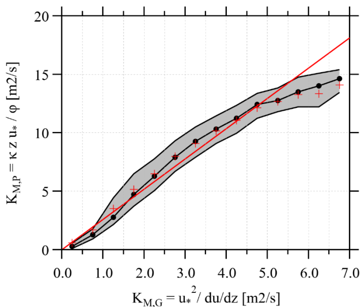
Figure 2: A comparison of momentum diffusion coefficients ( K_M ) determined through flux/gradient method ( K_{M,G} ), compared to the parameterization of Eq. 5 and 6 ( K_{M,P} ). The parameterized values are binned by flux/gradient values. Black circles show medians, grey shading shows 25 th and 75 th percentiles, red pluses show averages, and the red straight line shows a least-squares fit to all 30-min data.
