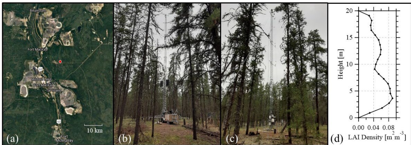
585 Figure 1: (a) The study area and surrounding location showing the location of the towers (red dot) relative to oil sands mining and production facilities. (b) A photo of YAJP tower. (c) A photo of WBEA 1004 tower. (d) The LAI density profile near the YAJP station. Map image is © Google Maps. Photos taken by authors.
