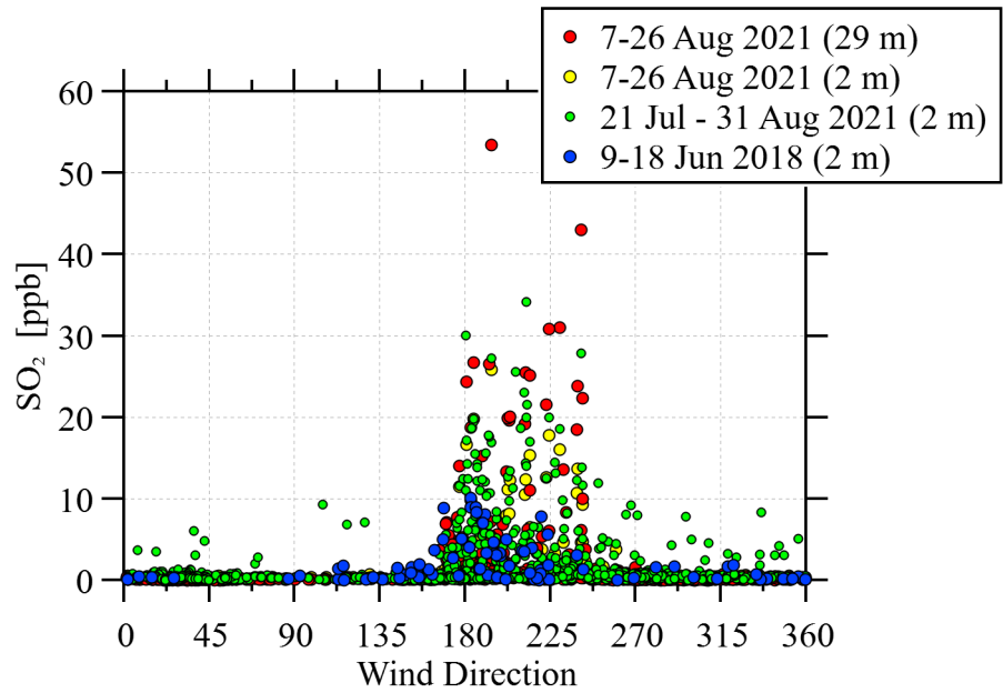
Figure 5: SO 2 measurements as a function of wind direction. Green dots are AF22e measurements. All others are 43i measurements. All measurements here are 30-min averages.
