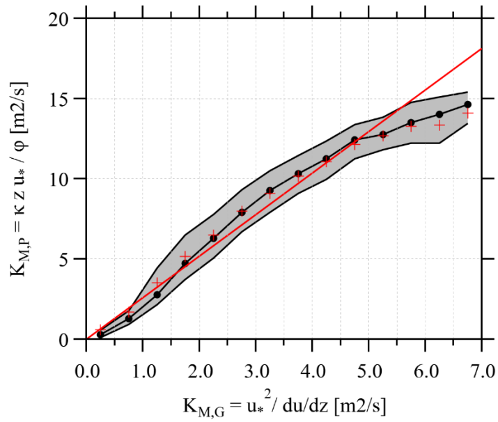
Figure 3: A comparison of momentum diffusion coefficients ( K_M ) determined through flux/gradient method ( K_{M,G} ), compared to the parameterization of Eq. 5 and 6 ( K_{M,P} ). The parameterized values are binned by flux/gradient values. Black circles show medians, grey shading shows 25 th and 75 th percentiles, red pluses show averages, and the red straight line shows a least-squares fit to all 30-min data.
