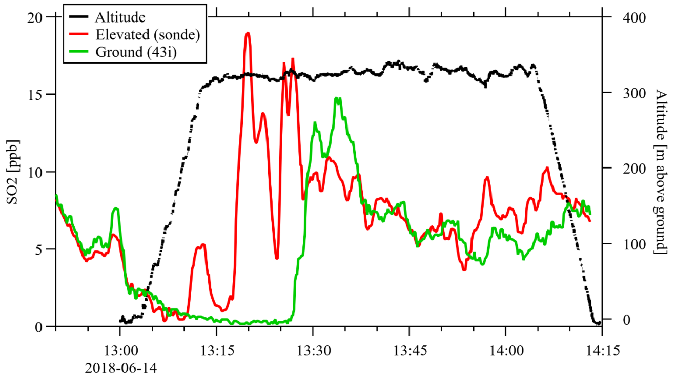
Figure 6: SO 2 measurements on a tethered balloon flight (SO 2 sonde, red line) and ground level measurements (43i, green line). Balloon altitude (black line) also shown. Ground level is ~340 m ASL.
