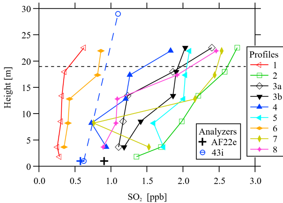
620 Figure 7: Measurements of SO 2 mixing ratio with height. Profile numbers correspond to those listed in Table 1. Open symbols are profiles measured at YAJP. Closed symbols are profiles measured at site 1004. Circle (○) plot markers (blue with dashed line) show average measurements of two 43i instruments over a period coincident with Profile 4. Plus (+) plot markers show average measurement of AF22e instrument over two periods coincident with Profiles 3a and 3b (black) and Profile 4 (blue). The approximate canopy height is shown as a dashed horizontal line.
