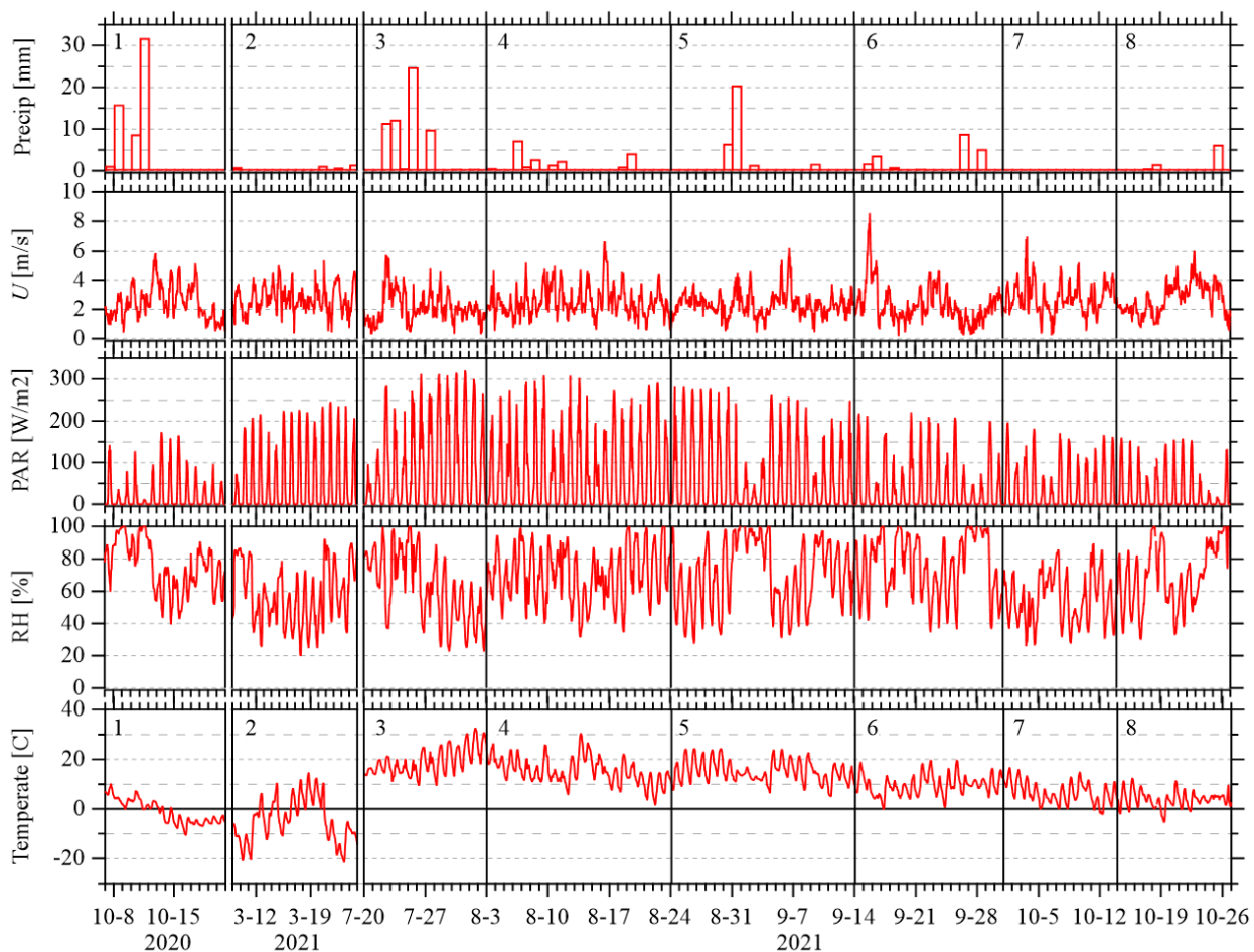
630 Figure A1: Meteorological data during the 8 sampling periods. Daily precipitation is from Mildred Lake (ECCC), which is 12 km SW of the towers. Wind speed at 29-m ( U ), photosynthetically active radiation (PAR), relative humidity (RH), and temperature are from the 1004 tower.
