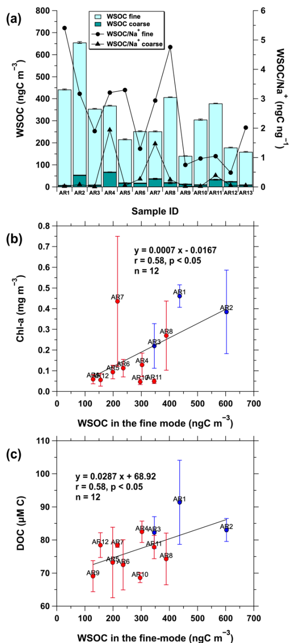
Figure 4: (a) Concentration of WSOC (ngC m -3 ) and WSOC/Na + ratio (ngC ng -1 ) in both fine- ( D < 2.5 \mu\text{m} ) and coarse-modes aerosols ( 2.5 \mu\text{m} < D < 10 \mu\text{m} ). Relationships of WSOC concentration in the fine-mode aerosols (ngC m -3 ) with (b) in situ surface chlorophyll-a (Chl-a) concentration (mg m -3 ) and (c) surface dissolved organic carbon (DOC) concentration (μM C). Chl-a and DOC concentrations are presented in their mean values and standard deviations for each aerosol sampling time. The blue and red solid circles in (b) and (c) indicate the samples collected from the coastal and sea ice-covered areas, respectively. Chl-a and DOC concentrations were not measured during the collection of the AR13 aerosol sample.
