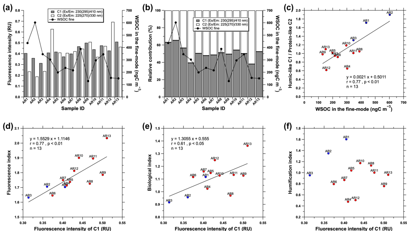
Figure 7: (a) Variations in the fluorescence intensities and (b) relative contributions of C1 and C2 in the fine-mode aerosols collected over the western Arctic Ocean during the summer of 2016. The black lines with circles in (a) and (b) indicate the WSOC concentration in the fine-mode aerosols. (c) Relationship between the fluorescence intensity ratio of the humic-like C1/protein-like C2 and the WSOC concentration in the fine-mode aerosol particles. (d) Fluorescence index (FI), (e) biological index (BIX), and (f) humification index (HIX) as a function of the fluorescence intensity of the humic-like C1 in the fine-mode aerosols. The blue and red solid circles in (c)–(f) indicate the samples collected from the coastal and sea ice-covered areas, respectively.
