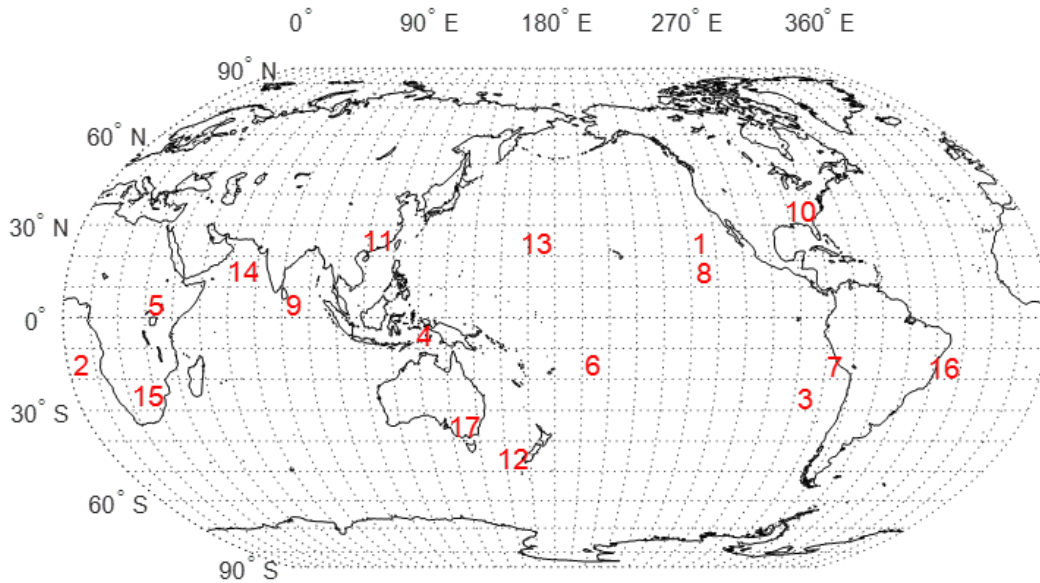
615 Figure 8: Center locations of selected sites for regional analysis of water vapor trends.
