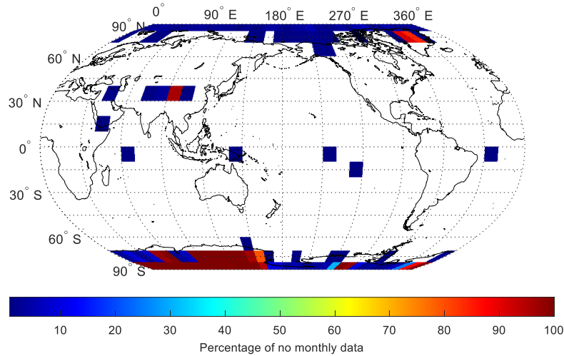
535 Figure 6: The percentage of missing monthly data over the 2007 to 2018 interval on the global 10^\circ \times 10^\circ grids. The percentage of missing data is shown as color-coded. Grids with complete monthly data and without gaps, i.e., covering all months, are represented as white blank spaces.
