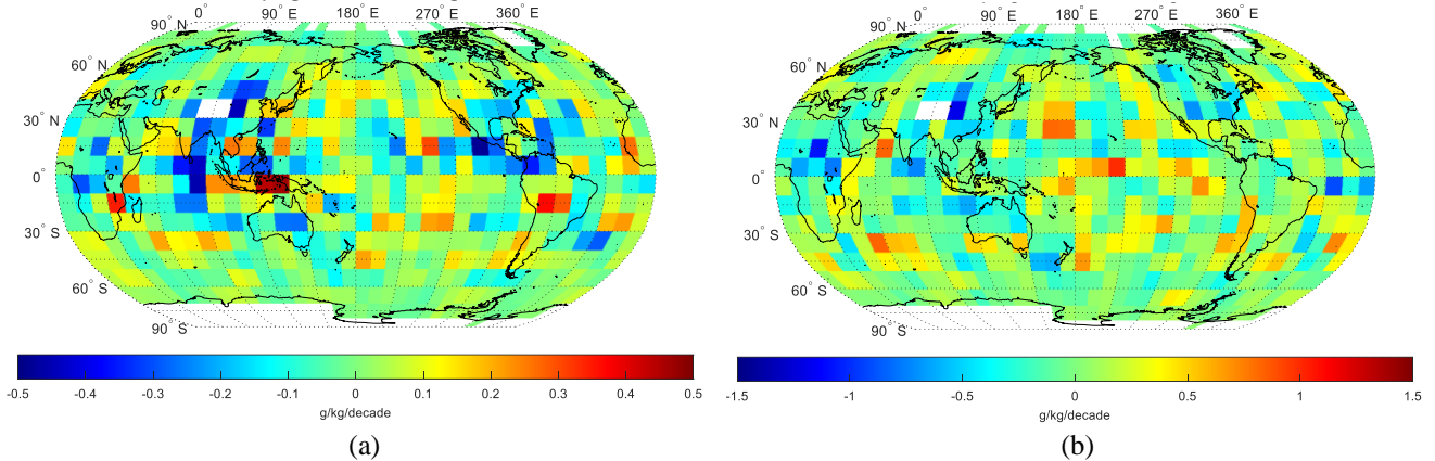
Figure A.5: (a) and (b) The distribution of trends of sampling error Q_{SE} time series at 500 and 850 hPa, respectively. The white blanks in (a) and (b) are grids with > 1.5\% missing monthly data over the 2007 to 2018 interval.
