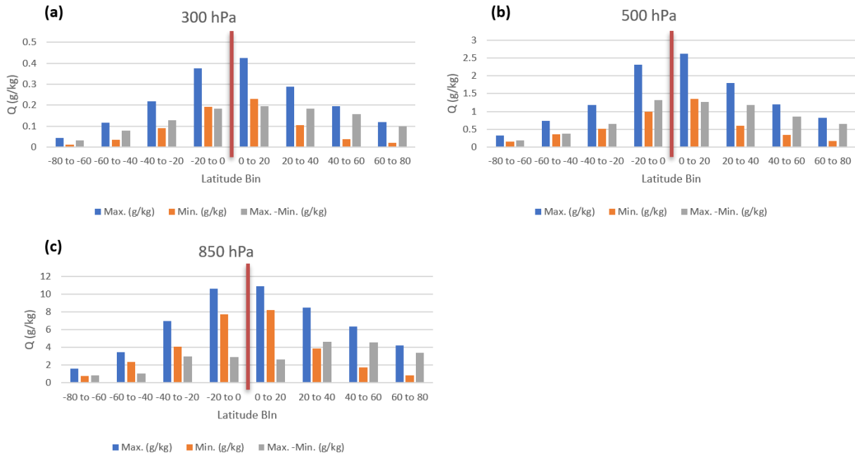
825 Figure A.3: Maximum, minimum, and maximum-minimum annual monthly water vapor statistics at three pressure levels (a) 300, (b) 500, and (c) 850 hPa from COSMIC retrievals. The vertical red line in each panel separates the latitude bins in the southern (to its left) and northern (to its right) hemispheres.
