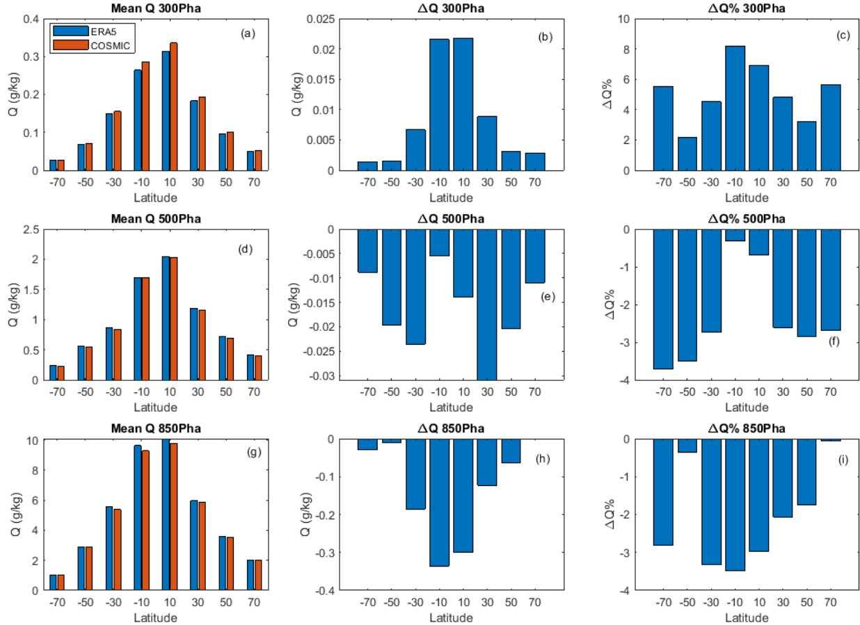
360 Figure 3: (a, d, g) Comparison of bin-mean water vapor between COSMIC retrieved data and ERA5 data at three pressure levels. Panels (b, e, h) and (c, f, i) show the value-difference and percent-difference (COSMIC minus ERA5) of latitude bin-mean water vapor data between COSMIC retrieved data and ERA5 data, respectively. The Top, middle, and bottom rows show the comparisons at 300, 500, and 850 hPa, respectively. In all bar-chart panels, the bar centers on the x-axis are placed at the centers of the 20-degree latitudinal bins. For this figure, collocated COSMIC and ERA5 water vapor data for all months of the considered 12-year period (2007-2018) have been used to calculate the mean water vapor in the corresponding latitude bins.
