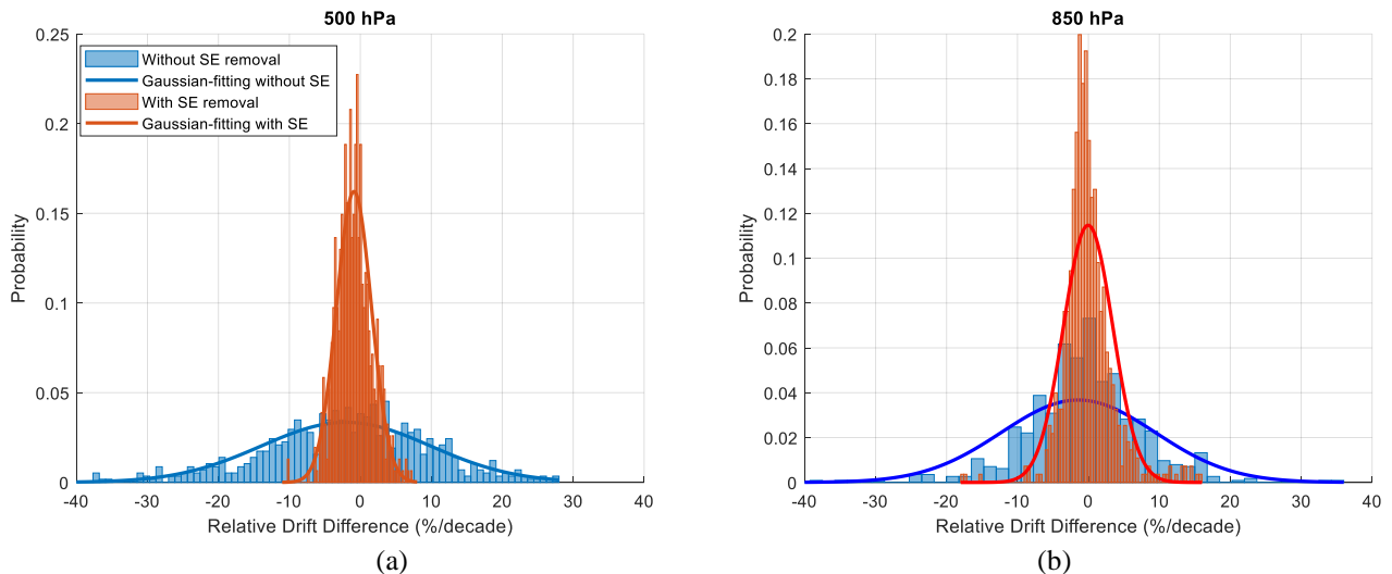
Figure A.6: (a, b) The histogram of relative water vapor trend difference (%/decade) between COSMIC and ERA5 water vapor at 955 500 and 850 hPa, respectively. In both panels, blue and orange bar charts are the distribution of the COSMIC water vapor trend difference relative to ERA5 before and after the sampling error removal was applied, respectively. The blue and red lines are the Gaussian-fitted distribution of the relative water vapor trend difference for the FWHM calculation.
