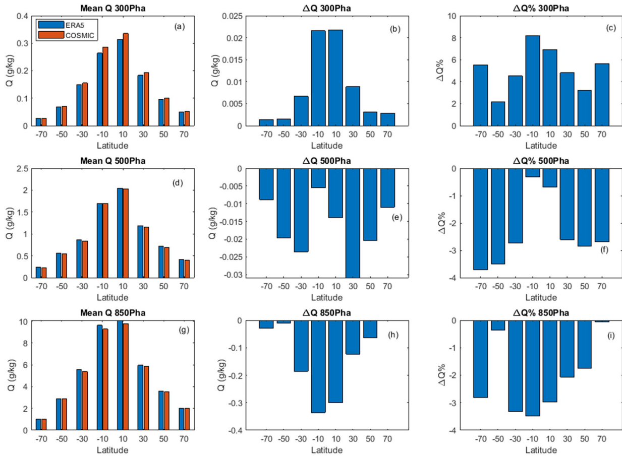
365 Figure 3: (a, d, g) Comparison of bin-mean water vapor between COSMIC retrieved data and ERA5 data at three pressure levels. Panels (b, e, h) and (c, f, i) show the value-difference and percent-difference (COSMIC minus ERA5) of latitude bin-mean water vapor data between COSMIC retrieved data and ERA5 data, respectively. The Top, middle, and bottom rows show the comparisons at 300, 500, and 850 hPa, respectively. In all bar-chart panels, the bar centers on the x-axis are placed at the centers of the 20-degree latitudinal bins. For this figure, collocated COSMIC and ERA5 water vapor data for all months of the considered 12-year period (2007-2018) have been used to calculate the mean water vapor in the corresponding latitude bins.
