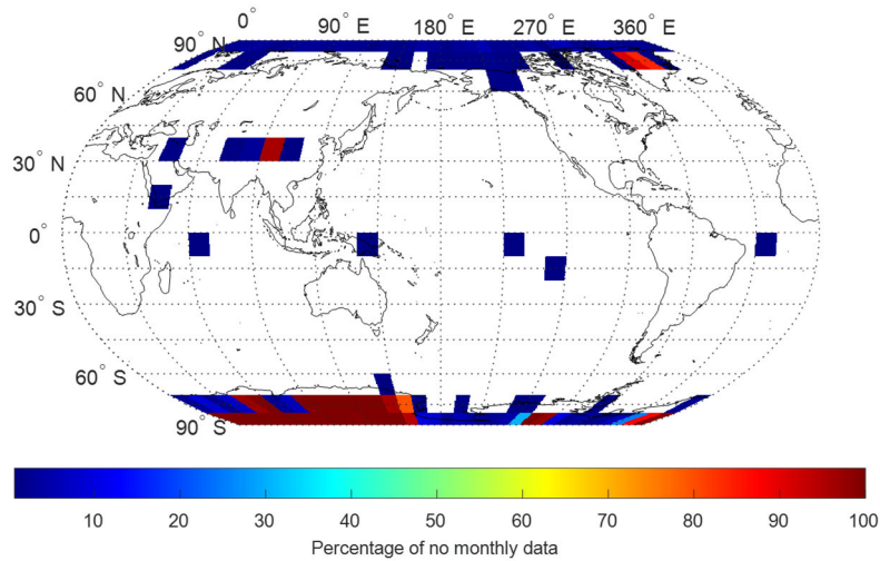
540 Figure 6: The percentage of missing monthly data over the 2007 to 2018 interval on the global 10^\circ \times 10^\circ grids. The percentage of missing data is shown as color-coded. Grids with complete monthly data and without gaps, i.e., covering all months, are represented as white blank spaces.
