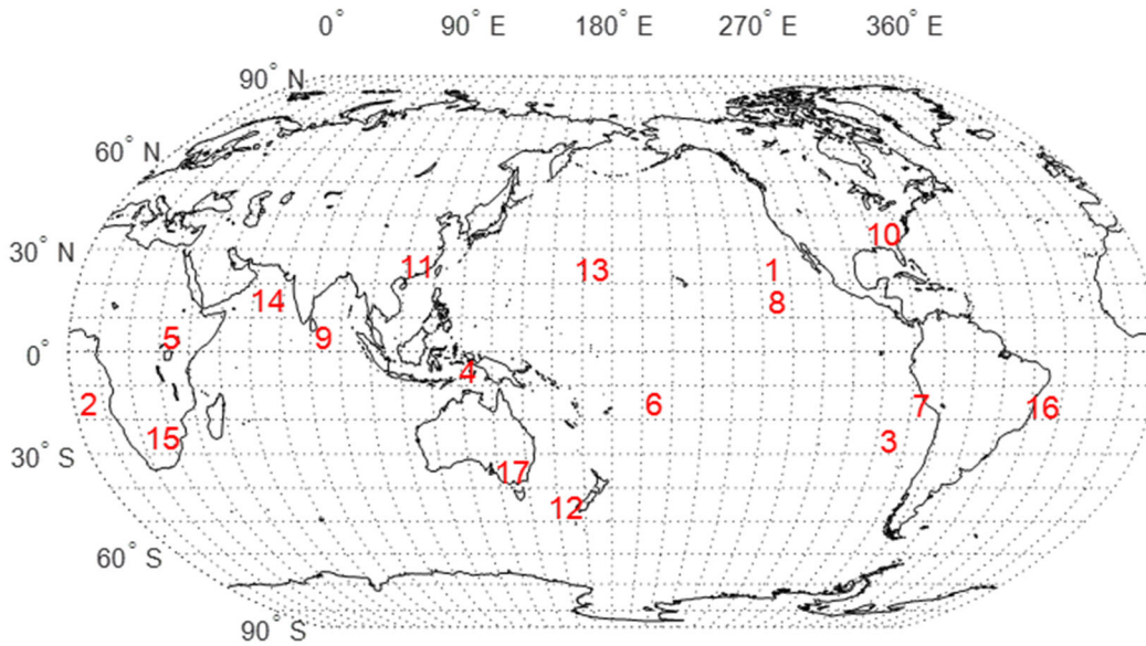
Figure 8: Center locations of selected sites for regional analysis of water vapor trends.
