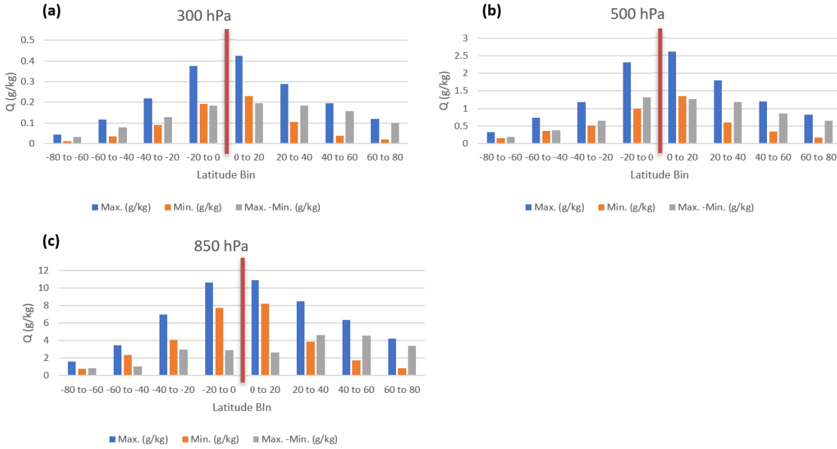
830 Figure A.3: Maximum, minimum, and maximum-minimum annual monthly water vapor statistics at three pressure levels (a) 300, (b) 500, and (c) 850 hPa from COSMIC retrievals. The vertical red line in each panel separates the latitude bins in the southern (to its left) and northern (to its right) hemispheres.
