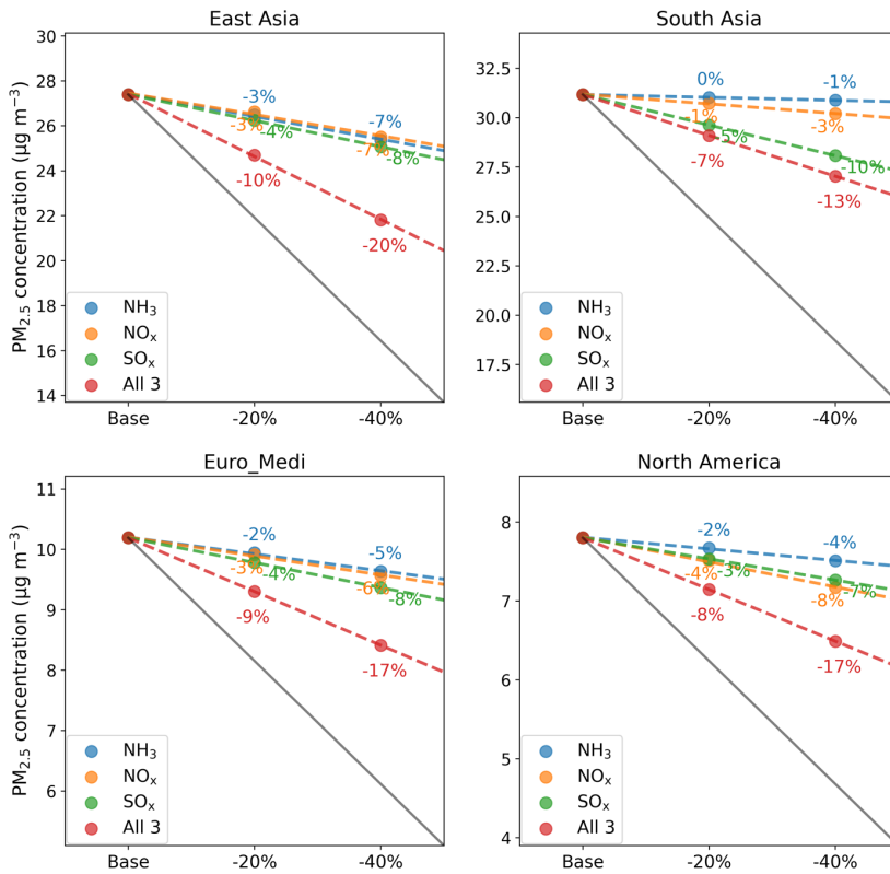
Figure 10: The absolute and relative sensitivities of regionally-averaged annual mean surface concentrations of PM 2.5 to 20% and 40% emissions reductions in NH 3 (blue), NO x (orange) and SO x (green) individually, and collectively (red), for the four regions defined in Fig. 1. The solid grey line in each panel illustrates the one-to-one relative response to emissions reductions, whilst the coloured dashed lines are the linear regressions through each set of three model simulations and illustrate the actual responses to emissions reductions of a given precursor. The numbers show the corresponding relative responses to each emissions reduction (with respect to baseline).
