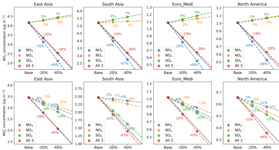
Figure 3: The absolute and relative sensitivities of regionally-averaged annual mean surface concentrations of \text{NH}_3 (upper row) and \text{NH}_4^+ (lower row) to 20% and 40% emissions reductions in \text{NH}_3 (blue), \text{NO}_x (orange) and \text{SO}_x (green) individually, and
