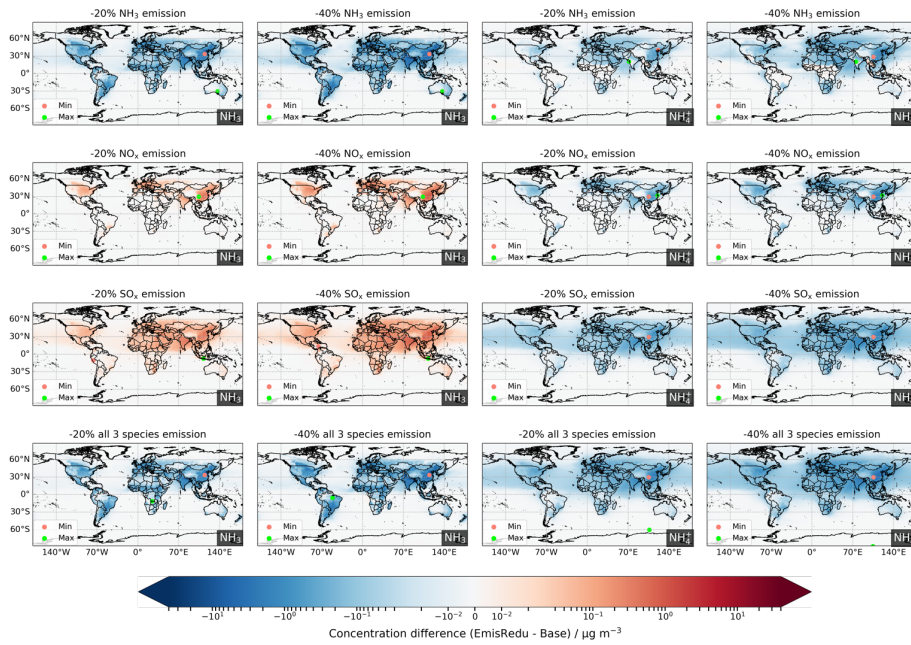
Figure 2: \Delta for 20% and 40% emissions reductions in \text{NH}_3 , \text{NO}_x , and \text{SO}_x individually and collectively. Red and green dots in each map locate the minimum and maximum difference, respectively.
