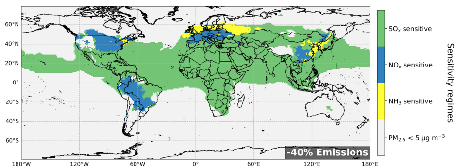
485 Figure 8: Spatial variation in sensitivity regime of PM 2.5 mitigation based on data from 40% individual reductions in emissions of NH 3 , NO x , or SO x . The regime is defined according to the precursor that yields the greatest decreases in grid PM 2.5 concentration: NH 3 sensitive (yellow), NO x sensitive (blue), SO x sensitive (green). Model grids with baseline annual mean PM 2.5 concentrations <5 μg m -3 are masked out.
