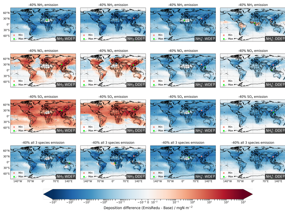
605 Figure 11: Changes in wet (WDEP) and dry deposition (DDEP) of \text{NH}_3 and \text{NH}_4^+ for 40% emissions reductions in \text{NH}_3 , \text{NO}_x , and \text{SO}_2 individually and collectively. Red and green dots in each map locate the minimum and maximum difference, respectively.
