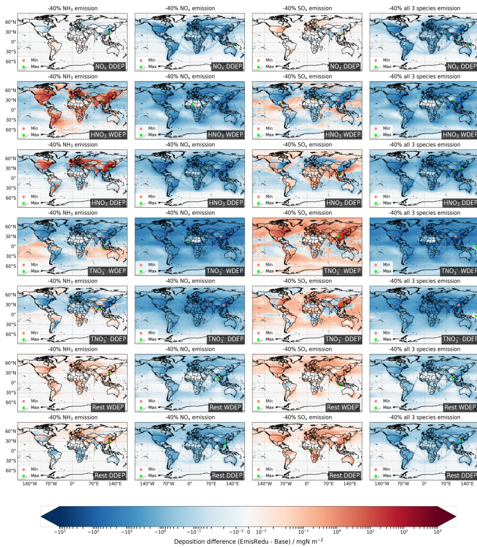
610 Figure 12: Changes in wet (WDEP) and dry deposition (DDEP) of NO x , HNO 3 , TNO 3 (fine + coarse NO 3 ), and Rest OXN species for 40% emissions reductions in NH 3 , NO x , and SO x individually and collectively. Red and green dots in each map locate the minimum and maximum difference, respectively.
