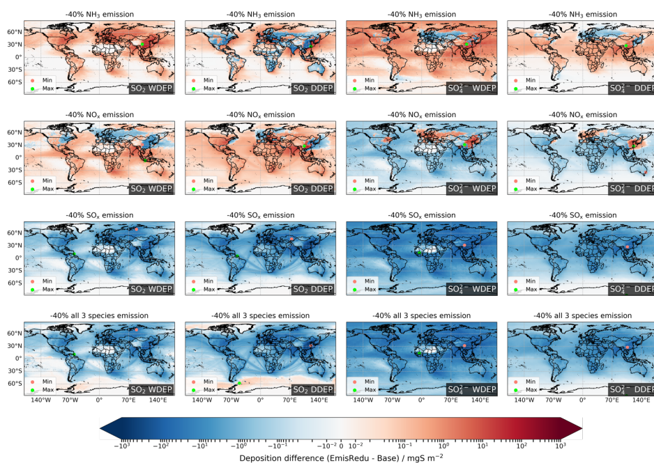
Figure 13: Changes in wet (WDEP) and dry deposition (DDEP) of \text{SO}_2 and \text{SO}_4^{2-} for 40% emissions reductions in \text{NH}_3 , \text{NO}_x , and \text{SO}_2 , individually and collectively. Red and green dots in each map locate the minimum and maximum difference, respectively.
