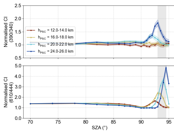
Figure A2. Simulation result (normalised CI) for different PSC layer heights h_{\text{PSC}} ( \tau_{\text{PSC}} = 0.05 ). The PSC is confined in a 2^\circ \times 2^\circ area.
