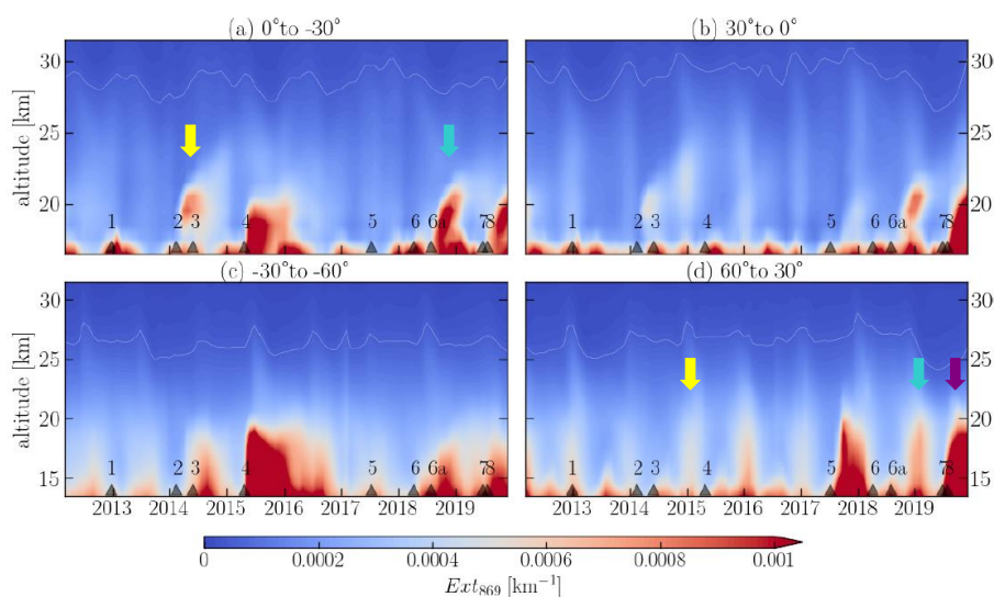
Figure 13. Monthly mean aerosol extinction coefficient ( Ext_{869} ) distribution from the OMPS-LP satellite instrument. The triangles represent volcanic eruptions and biomass burning events. Coloured arrows indicate the events which are important to this study. Adapted from Malinina et al. (2021).
