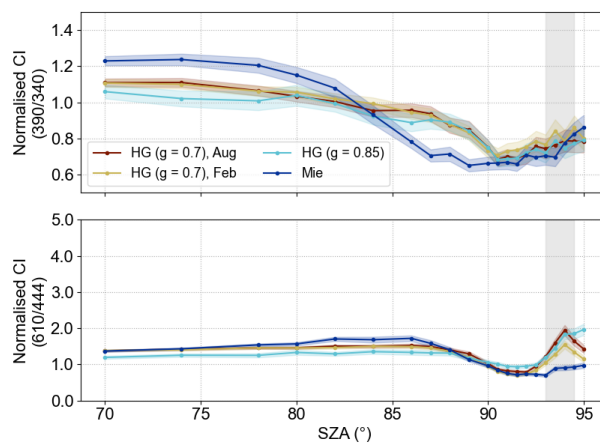
Figure A4. Simulation result (normalised CI) for different scattering phase functions and atmospheric profiles. The PSC layer is described by \tau_{\text{PSC}} = 0.05 and h_{\text{PSC}} = 20 to 22 km. The considered phase functions are presented in Fig. A3.
