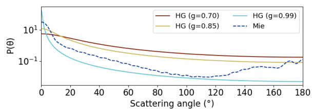
Figure A3. Comparison of different scattering phase functions P(\theta) . It shows different Henyey-Greenstein (HG) phase functions with their respective asymmetry parameter g as well as a computed Mie phase function (details see Sect. 3.1).
