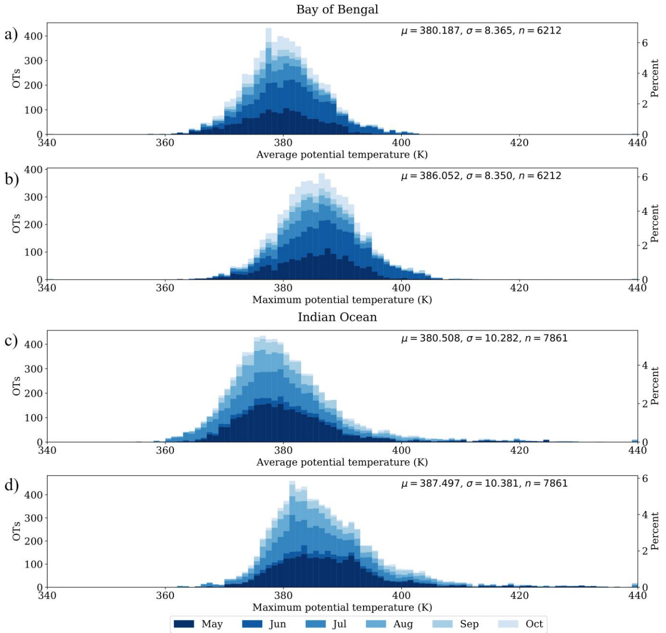
400 Figure 7 As Figure 5, but for the potential temperature distributions of OTs over the Bay of Bengal region (Figures 7a and 7b) and the Indian Ocean region (Figures 7c and 7d).
