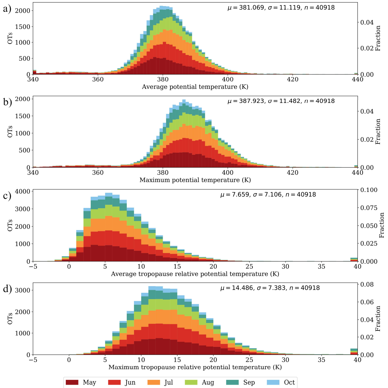
310 Figure 4 The vertical distribution of all OTs within the study region. Figures 4a and 4b show the distributions of the average and maximum potential temperature of each OT binned by 1 K, respectively. Figures 4c and 4d show the distributions of the average and maximum tropopause relative potential temperature of each OT binned by 1 K, respectively. Within each bin, color indicates the fractional contribution of each month. For example, the 12 K average tropopause relative potential temperature bin is
