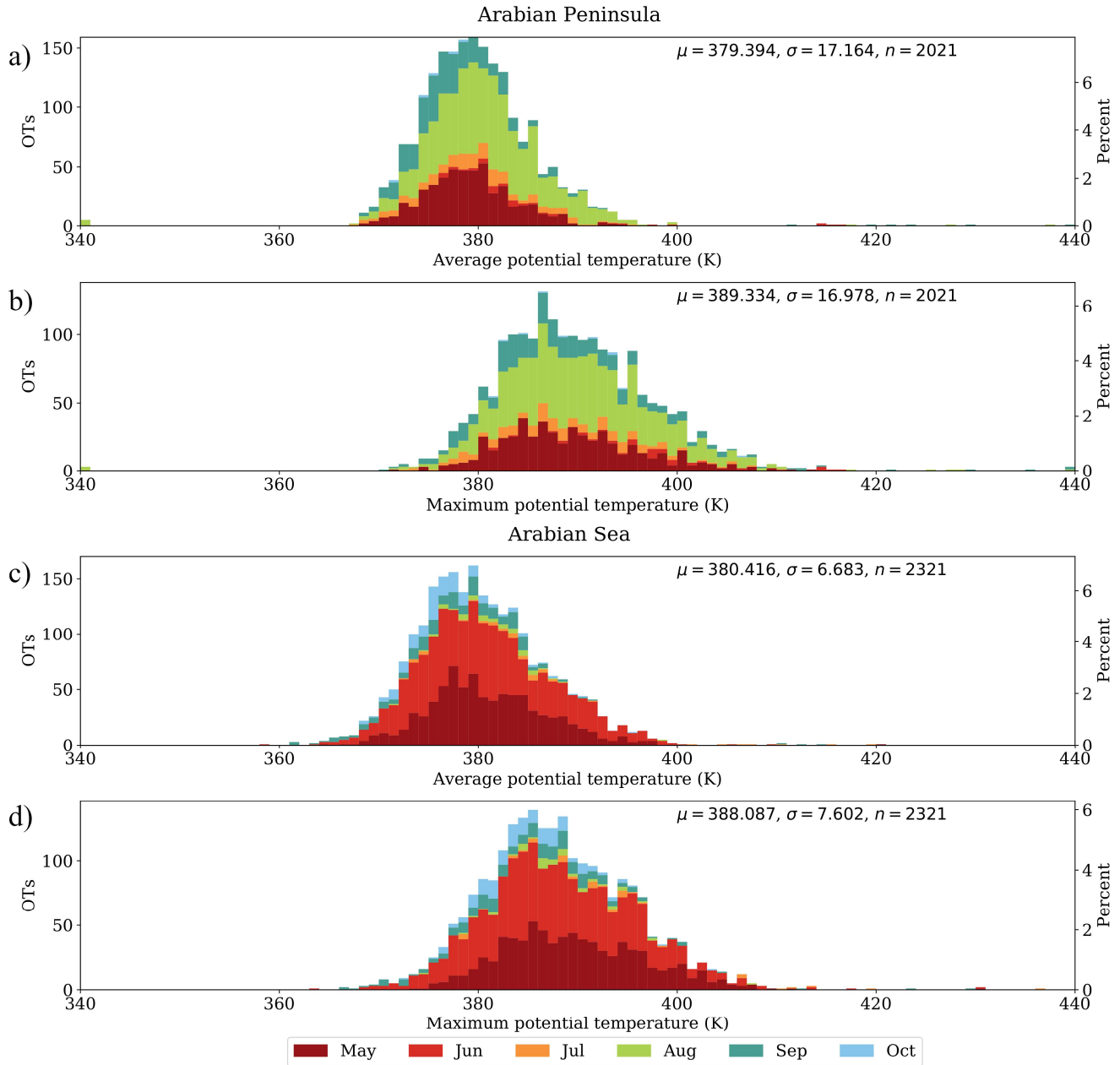
Figure 8 As Figure 5, but for the potential temperature distributions of OTs over the Arabian Peninsula region (Figures 8a and 410 8b) and the Arabian Sea region (Figures 8c and 8d).
