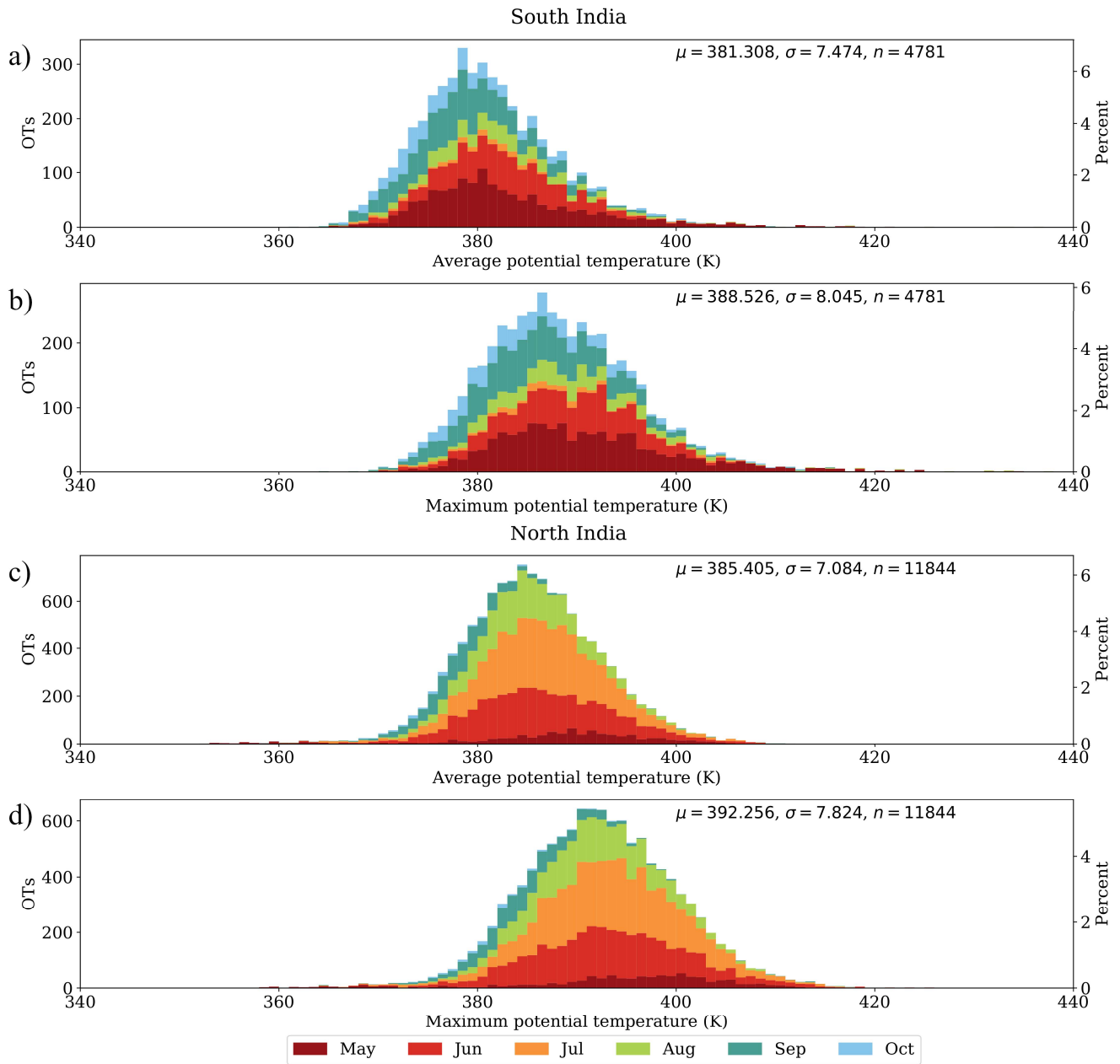
345 Figure 5 The potential temperature distribution of OTs within the South India (Figures 5a and 5b) and North India (Figures 5c and 5d) regions. Figures 5a and 5b show the distributions of the average and maximum potential temperature of OTs occurring within the South India region binned by 1 K, respectively. Figures 5c and 5d show the distributions of the average and maximum potential temperature of OTs occurring within the North India region binned by 1 K, respectively. Within each bin, color indicates the fractional contribution of each month, as in Figure 4. The mean, standard deviation, and number of OTs for each distribution is indicated in the upper-right corner. 350
