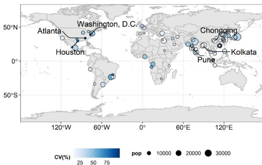
415 Figure 14. Temporal coefficient of variation (CV) of monthly mean AOD (intra-annual variability) expressed in percentages for megacities urban domain (~40kmx40km around cities centre). The circle radius is proportional to cities population. Three cities with the highest temporal CV are Atlanta, Houston and Washington, D.C. and the three cities with lowest values are Kolkata, Chongqing and Pune.
