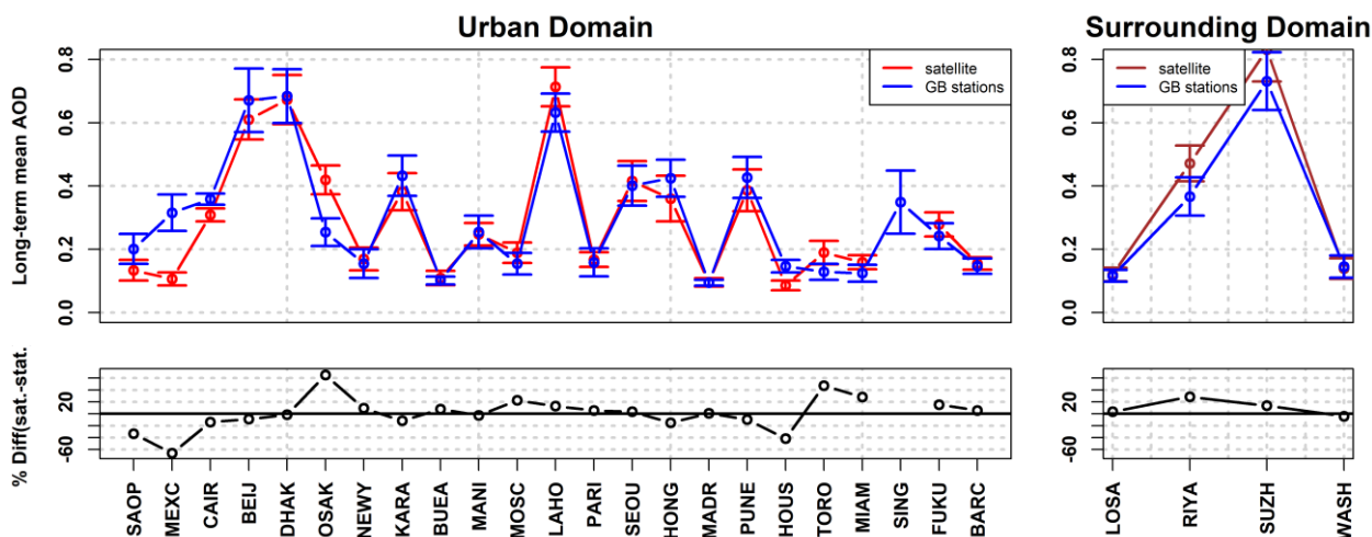
Figure 17. Upper panels: Satellite derived (red line) and GB (blue) long term mean AOD for urban domain (left) and surrounding domain (right). Lower panel: Relative difference of mean AOD between satellite and GB measurements expressed in percentage for urban domain (left) and surrounding domain (right).
