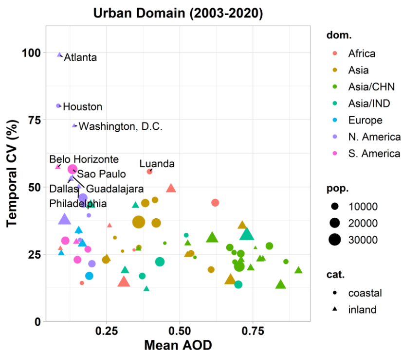
420 Figure 15. Temporal coefficient of variation expressed in percentages (CV%) against the long-term mean AOD for the urban domain. The size and the colour of the points denote cities' population and geographical domain, respectively. The shape of the points denotes coastal or inland cities.
