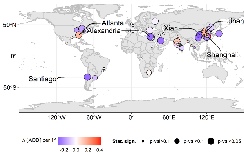
Figure 8. Spatial AOD gradients per 1 degree ( \Delta(\text{AOD}) per 1^\circ ) from city center to surroundings. The circle radius is proportion statistical significance of the trends. Three cities with greatest negative AOD gradient are Xian, Alexandria and Santiago and the three cities with greatest positive AOD gradient are Shanghai, Jinan and Atlanta.
