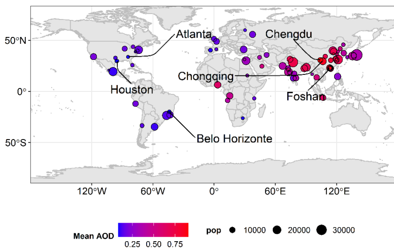
305 Figure 9. Long term (2003-2020) mean AOD for megacities urban domain (~40kmx40km around cities centre). The circle radius is proportion to cities population. Three cities with greatest mean AOD are those of Chengdu, Foshan and Chongqing and the three cities with lowest mean AOD values are those of Atlanta, Houston and Belo Horizonte.
