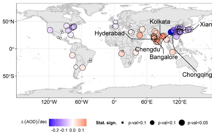
375 Figure 12. Linear trend of AOD per decade for urban domain (~40kmx40km around cities centre). The circle radius is proportion statistical significance of the trends. Three cities with greatest increase of AOD are Hyderabad, Kolkata and Bangalore and the three cities with greatest decrease of AOD are Chengdu, Chongqing and Xian.
