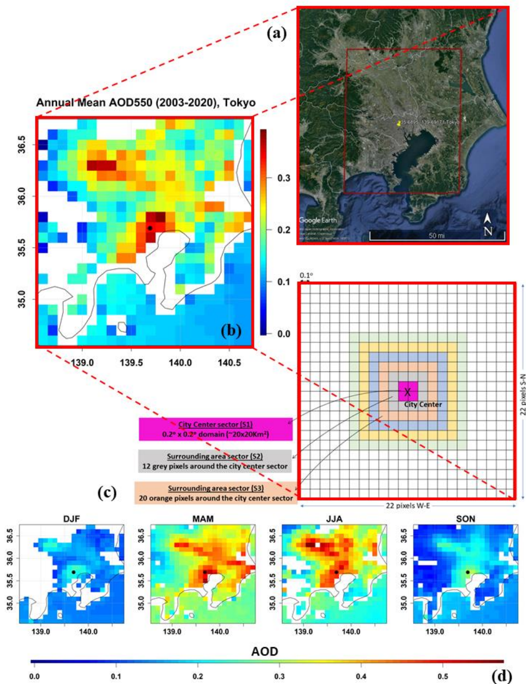
Figure 2. (a) Geographical limits of the study area for the megacity of Tokyo on © Google Earth maps. (b) Geographical distribution of the long-term (2003-2020) annual averaged AOD for the broader area of Tokyo megacity. (c) Spatial representation equal lat/lon grid of AOD data and the sectors under investigation with different colours. (d) Geographical distribution of the seasonally averaged AOD for the broader area of Tokyo megacity. Blanc pixels do not fulfil the data availability criteria. The black circle denotes the pixel of the megacity centre.
