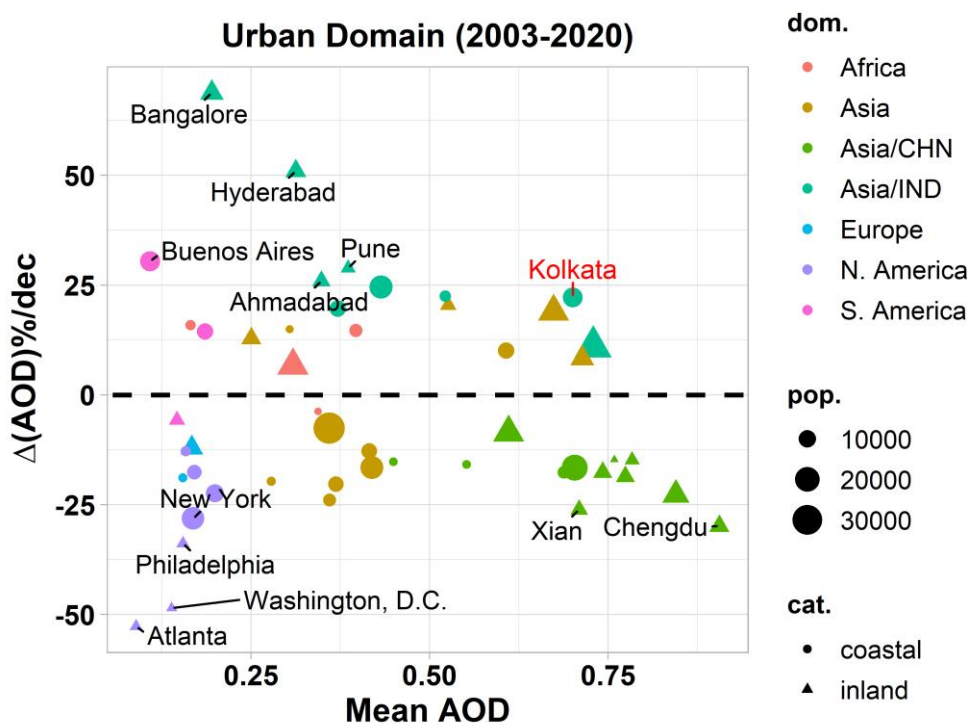
395 Figure 13. AOD decadal changes expressed in percentages ( \Delta(\text{AOD})\% per decade) versus the long-term mean AOD for the urban domain. Only statistically significant AOD trends are presented ( P < 0.1 ). Cities with absolute values of \Delta(\text{AOD})\% per decade greater than 25% are denoted in the figure.
