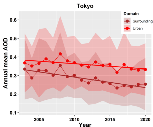
215 Figure 6. Annual mean AOD values for the Tokyo megacity (red points) and the surrounding area (brown points) and the corresponding standard deviations (shaded areas). The linear trends are depicted with the straight lines.
