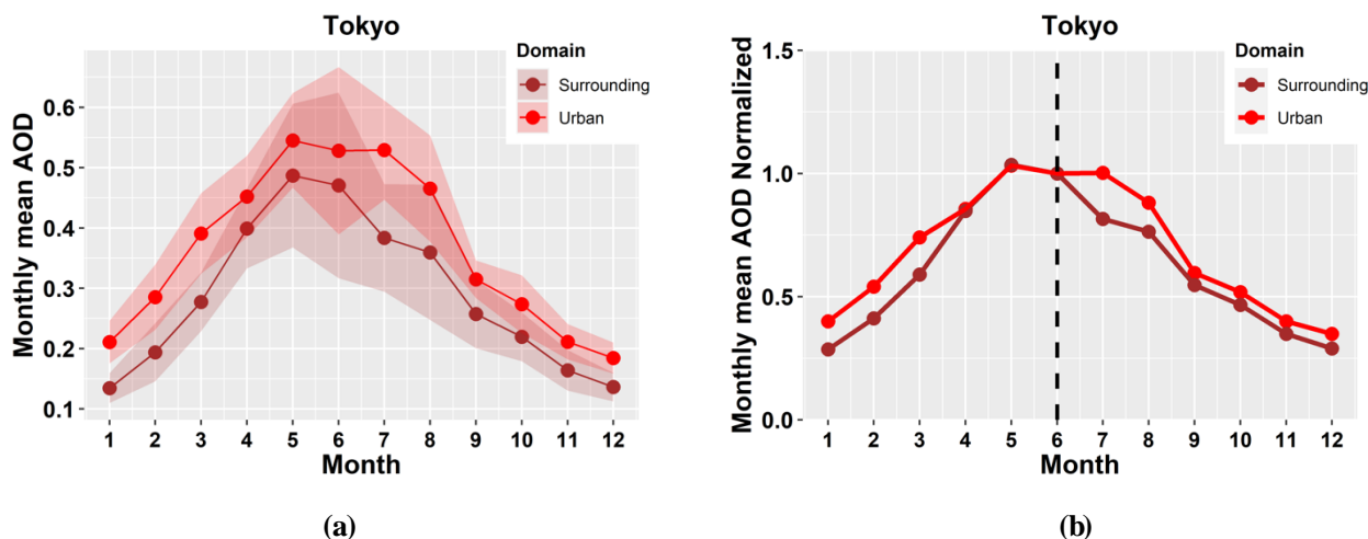
225 Figure 7. (a) AOD intra-annual variability for Tokyo megacity (red line) and the surrounded area (brown line). (b) Normalized monthly mean AOD values with respect to June mean AOD value.
