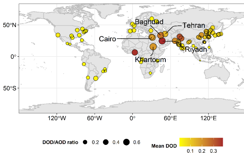
310 Figure 10. Long term (2003-2020) mean DOD for megacities urban domain (~40kmx40km around cities centre). The circle radius is proportion to DOD to AOD ratio. Five cities with greatest dust contribution (mean DOD/AOD ratio) are Khartoum, Riyadh, Baghdad, Cairo and Tehran.
