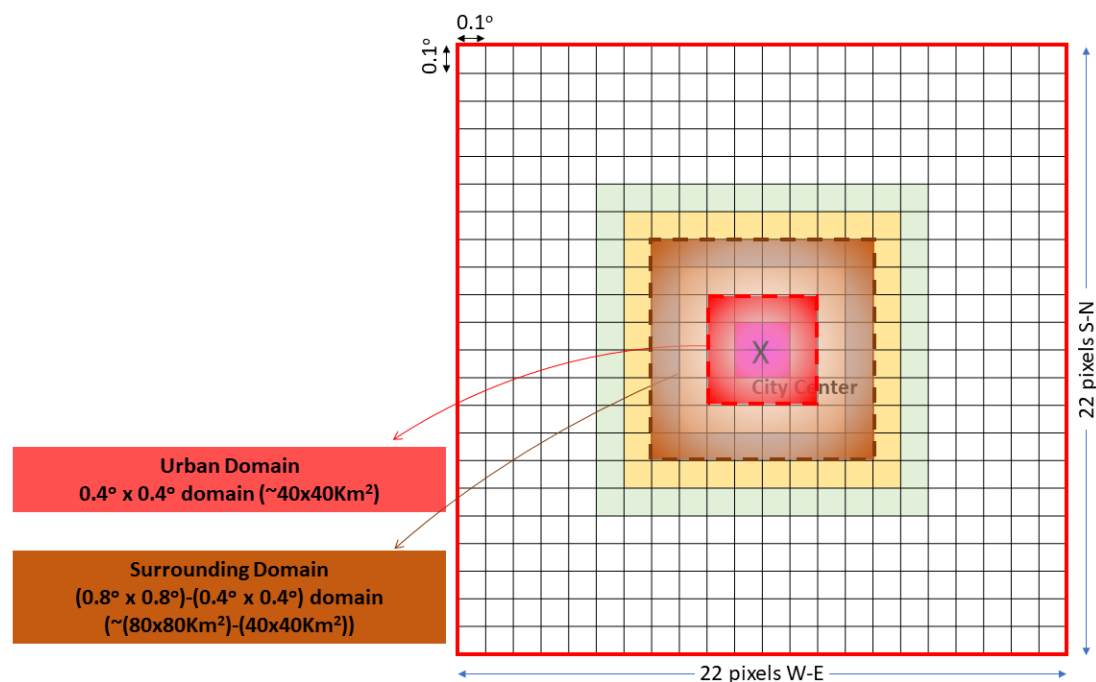
Figure 5. Spatial representation of equal lat/lon grid of the AOD data and the urban domain (red) and surrounding area domain (brown) under investigation.
