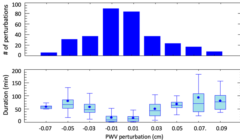
390 Figure 6: Top: Distribution of the 345 water vapor perturbations found in the 10 days analyzed. Bottom: Duration of water vapor perturbations binned by the amplitude of the perturbation, N= 6, 31, 37, 89, 83, 37, 23, 17, 8 for a total of 331 points. The 14 missing cases are distributed in the bins below -0.07 cm and above 0.09 cm with less than 5 points in
