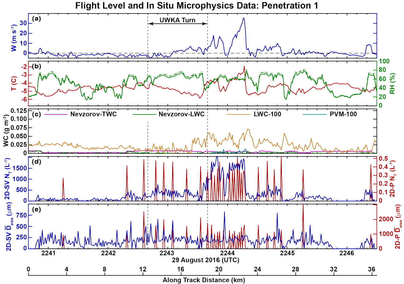
Figure 4. UWKA flight-level and in situ microphysics data for penetration 1 (Fig. 1d, Table 2). (a) Vertical air velocity (blue), (b) temperature (red), relative humidity with respect to liquid (green-solid) and relative humidity with respect to ice (green-dashed), (c) bulk water content (WC) from the Nevzorov-TWC probe (magenta), Nevzorov-LWC probe (green), LWC-100 probe (gold) and PVM-100 probe (cyan), (d) total concentration ( N_T ) from the 2D-SV probe (blue) and 2D-P probe (red), and (e) area-weighted mean diameter ( \bar{D}_{area} ) from the 2D-SV probe (blue) and 2D-P probe (red). Along-track distance for the penetration shown at bottom.
