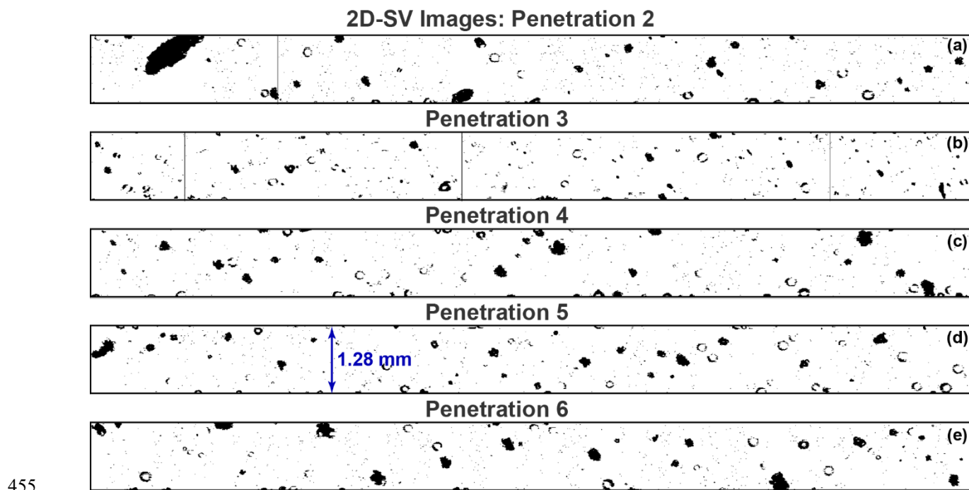
Figure 15. Sampling of 2D-SV particle images for penetrations 2-6 (Fig. 1d, Table 2). Vertical distance of each horizontal strip represents 1.28 mm.
