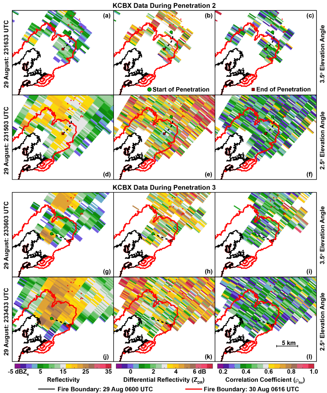
365 Figure 12. KCBX data approximately coincident with the execution of penetration 2 (a-f) and penetration 3 (g-l). Left column (a,d,g,j) 370 shows reflectivity, middle column (b,e,h,k) shows differential reflectivity ( Z_{DR} ) and right column (c,f,i,l) shows correlation coefficient ( \rho_{hv} ). Colour scales at bottom of each column indicate plotted values. Top row (a-c) is for data at 231633 UTC 29 August 2016 (3.5° elevation angle), second row (d-f) for data at 231503 UTC 29 August 2016 (2.5° elevation angle), third row (g-i) for data at 233603 UTC 29 August 2016 (3.5° elevation angle) and fourth row (j-l) for data at 233433 UTC 29 August 2016 (2.5° elevation angle). Perimeters of the Pioneer Fire at 0600 UTC 29 August 2016 and 0616 UTC 30 August 2016 are indicated with black and red lines, respectively. Black- dashed lines show the locations of penetrations 2 and 3, with green circles and red squares indicating the start and end of each penetration,
