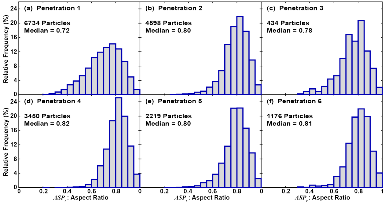
Figure 8. Histograms of 2D-SV particle aspect ratio ( ASP_r ) for (a-f) penetrations 1-6 (Fig. 1d, Table 2). Number of particles and distribution median indicated for each penetration.
