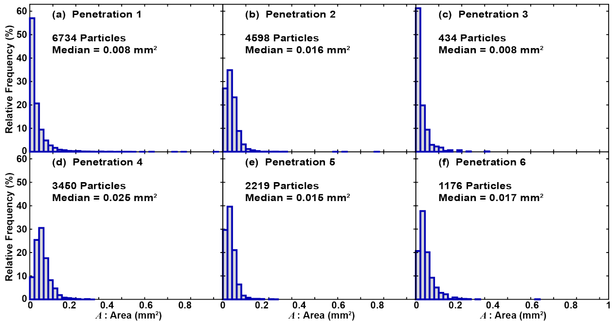
Figure 9. Same as Fig. 8 except for particle area ( A ).
