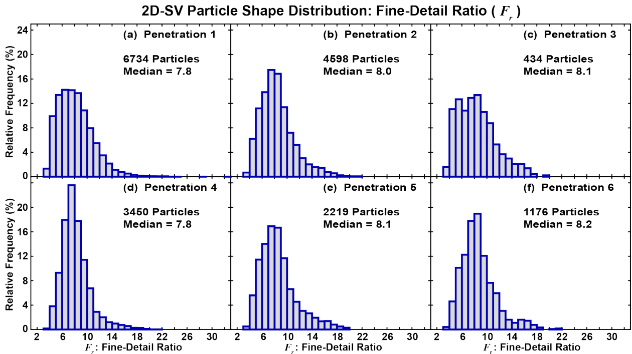
330 Figure 11. Same as Fig. 8 except for particle fine-detail ratio ( F_r ).
