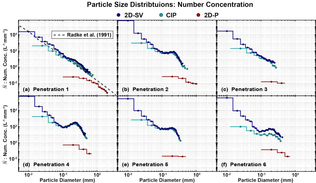
Figure 5. Size distributions of particle number concentration ( \hat{N} ) for (a-f) penetrations 1-6 (Fig. 1d, Table 2). Data from the 2D-SV, CIP, and 2D-P probes indicated by the blue, cyan, and red filled circles, respectively. Number concentration size distribution of giant ash particles from Radke et al. (1991) also plotted in (a).
