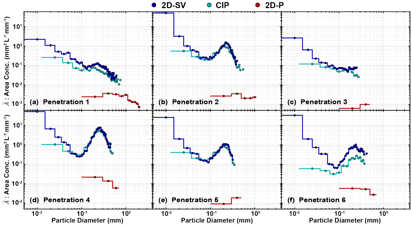
Figure 6. Same as Fig. 5 except for particle area concentration ( \hat{A} ).
