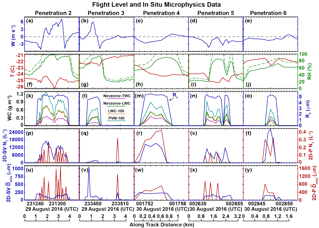
Figure 14. UWKA flight-level and in situ microphysics data for penetrations 2-6 (Fig. 1d, Table 2). (a-e) Vertical air velocity (blue), (f-j) temperature (red), relative humidity with respect to liquid (green-solid) and relative humidity with respect to ice (green-dashed), (k-o) bulk water content (WC) from the Nevzorov-TWC probe (magenta), Nevzorov-LWC probe (green), LWC-100 probe (gold), PVM-100 probe (cyan), and cloud-droplet effective radii ( R_e ) from the PVM-100 probe (blue), (p-t) total concentration ( N_T ) from the 2D-SV probe (blue) and 2D-P probe (red), and (u-y) area-weighted mean diameter ( \bar{D}_{area} ) from the 2D-SV probe (blue) and 2D-P probe (red). Along-track distance for each penetration shown at bottom.
