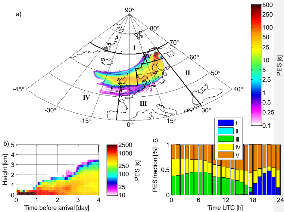
Figure 4: a) Horizontal distribution of vertically integrated PES for air masses arriving at Sammaltunturi on 20.09.2012 11:00 UTC. Source regions are indicated with Roman numerals. b) Vertical distribution of PES in panel a as function of time before arrival at Sammaltunturi. c) Timeline of the PES fraction for each source region for 20.09.2012.
