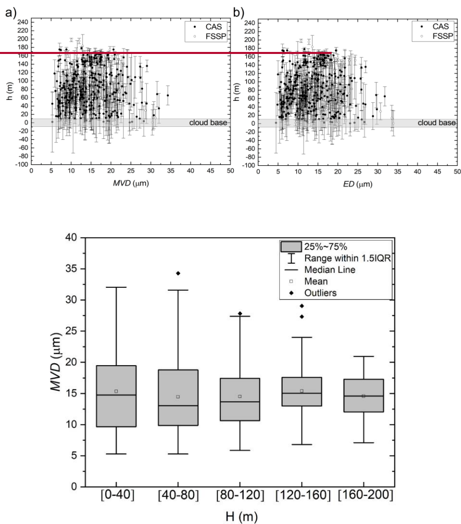
Figure 11. Statistical description of hourly averages of median volume diameter ( MVD ) as they were measured by the cloud and aerosol spectrometer (CAS) and the forward-scattering spectrometer probe (FSSP) where PES was within one region >80\% for five different levels of the position of the probes inside the cloud ( H ) (relative distance of the cloud ground-based spectrometer). Cloud base was measured at the Kenttäröva station.
