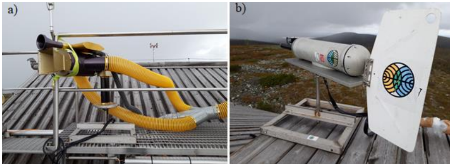
Figure 2. a) CAPS and b) FSSP-100 ground setups as installed on the roof of Sammaltunturi station during PaCE 2017.
