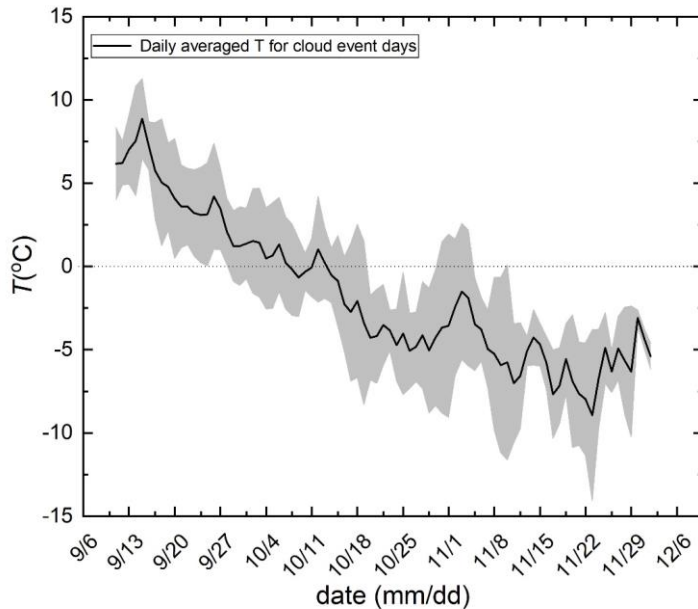
Figure 5: The daily averaged temperatures at the Sammaltunturi site for days with cloud events during all PaCE campaigns. The dotted line is used as a reference line for 0 °C temperature. The definition of a cloud event is provided in the text. The shaded area represents the corresponding standard deviations.
