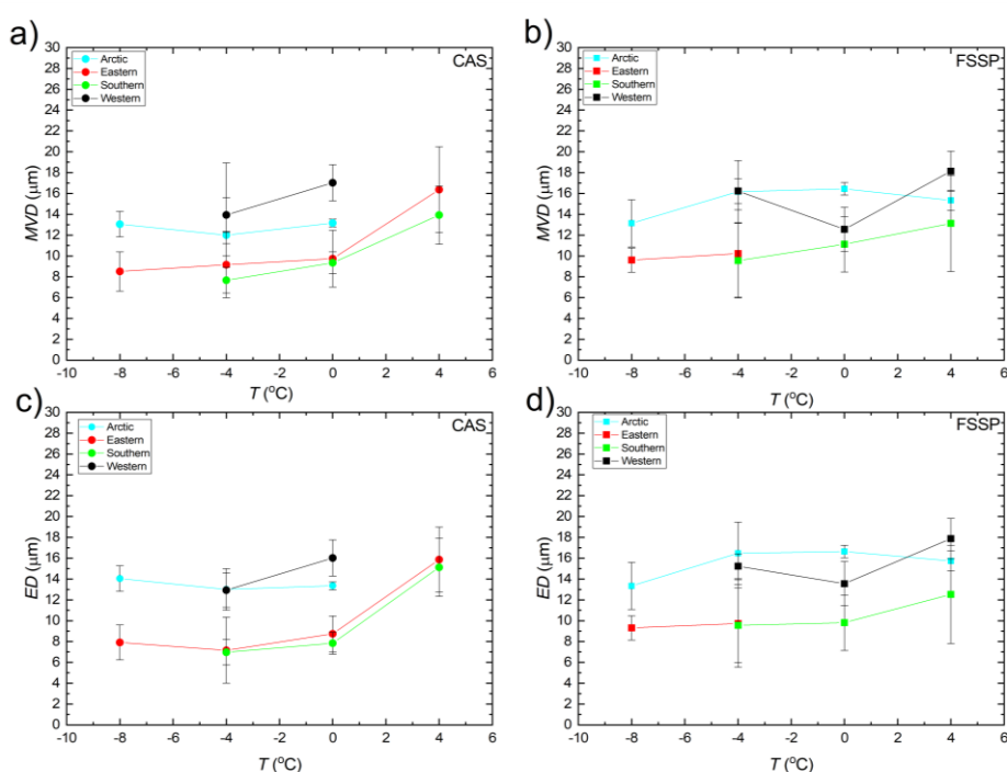
Figure 89. Hourly averages of median volume diameter (MVD) and effective diameter (ED) values versus temperature for all PaCE campaigns as they were measured by the cloud and aerosol spectrometer (CAS) and the forward-scattering spectrometer probe (FSSP) where the PES fraction was within one region >80 %. Solid lines were made to lead readers' eyes.
