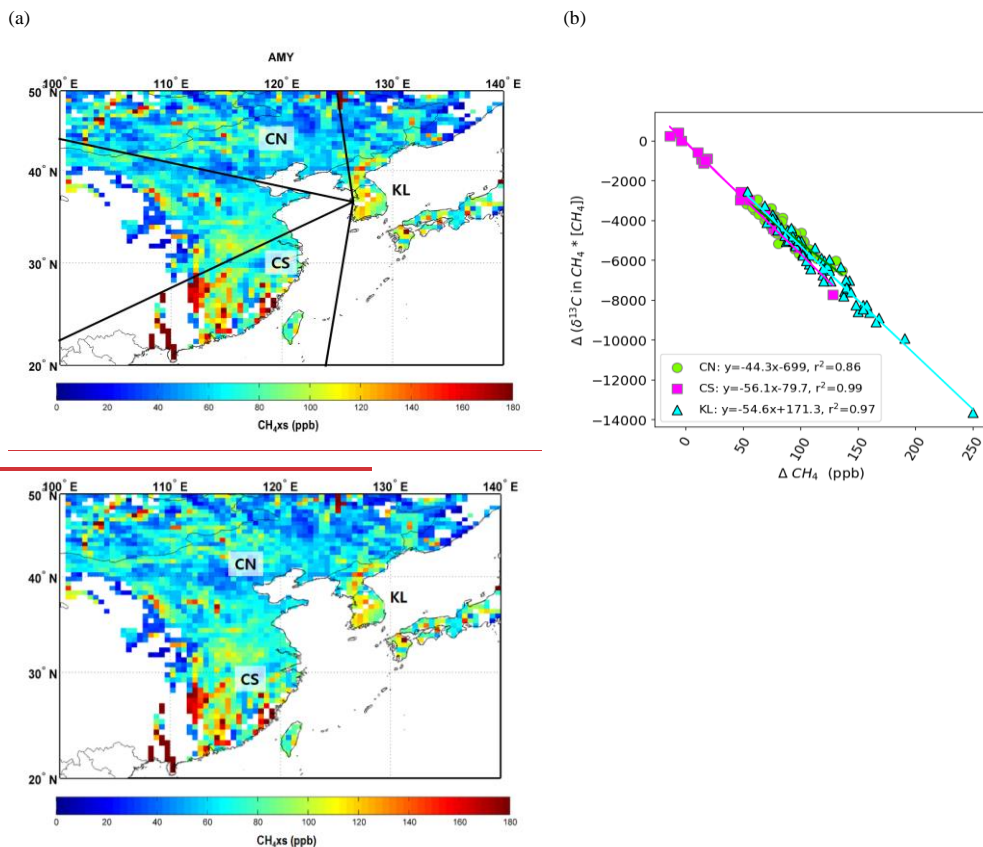
Figure 9. (a) PSS analysis with CH_4 observed at AMY and (b) “Miller-Tans” plots from 2006 to 2020. Miller-Tans plots showing the source signature of methane increments (TAP) into background air (Mauna-Loa).
