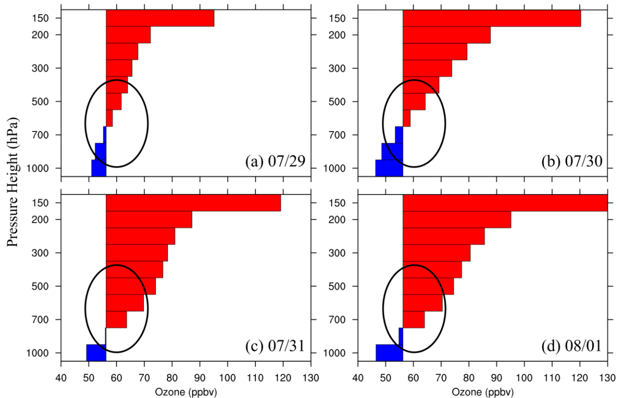
340 Figure 7: Spatially averaged profiles of ozone concentrations (unit: ppbv) over the NCP from the TROPES AIRS L2 ozone products on (a) 29 July, (b) 30 July, (c) 31 July, and (d) 1 August 2021, all indicated as month/day at the bottom right corners. The 10-day averaged ozone concentrations between the surface and 700 hPa over the NCP are used as the baseline, and positive (negative) departure from the 10-day averaged concentrations is shown in red (blue) color.
