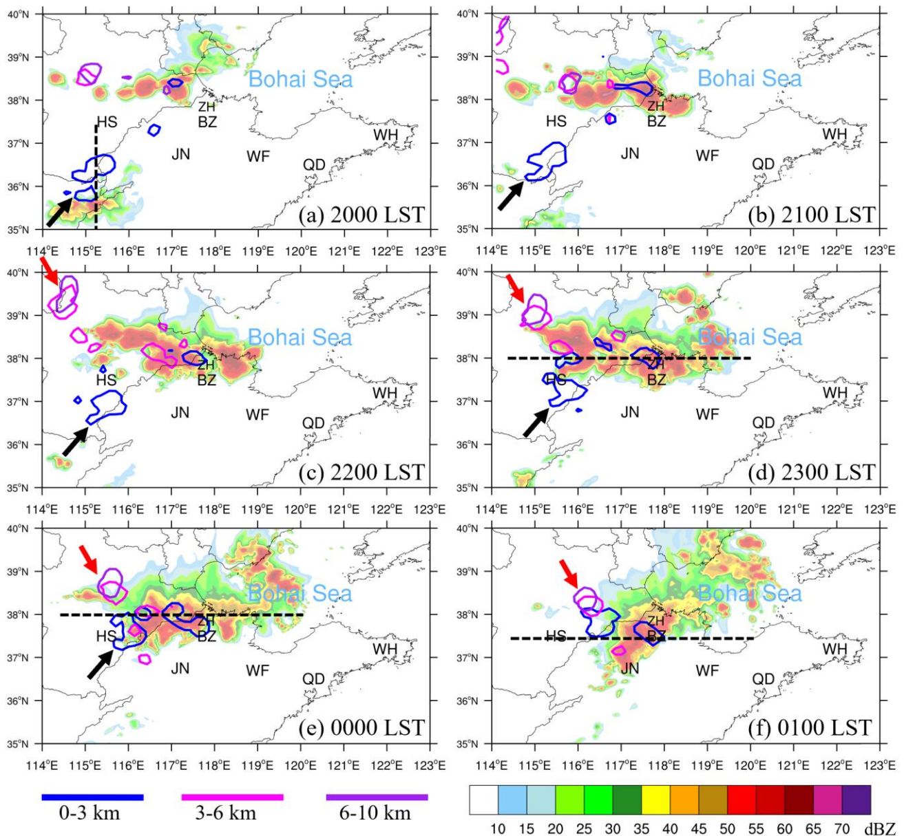
410 Figure 9: WRF-simulated radar reflectivity structure (shaded; dBZ) of the bow-echo MCSs occurred during the night of 31 July 2021. The solid lines represent regions with high tracer particle counts released in Binzhou between 0-3 km (blue lines), 3-6 km (magenta lines) and 6-10 km (purple lines). The black dashed lines are the cross-section lines used in Fig. 11. The red and black arrows highlight the movements of the tracer particles.
