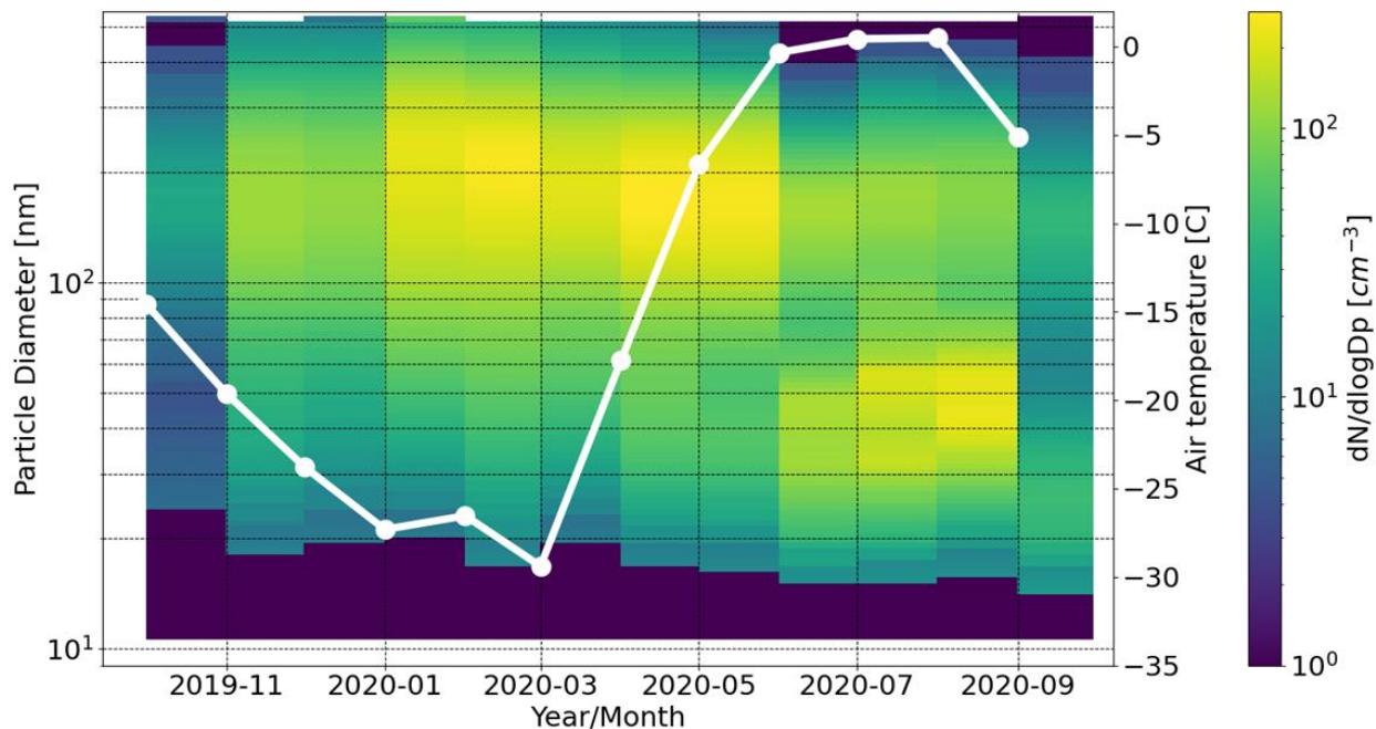
335 Figure 4: The annual aerosol size distribution and air temperature in the central Arctic during MOSAiC. The size distribution data are presented as monthly medians of the PNSD bins, where the concentration of the bins is represented by the color bar in units of dN/d\log D_p . The surface air temperature (in white), depicted as monthly averages, is included to give context to seasonal changes in the aerosol size distribution.
