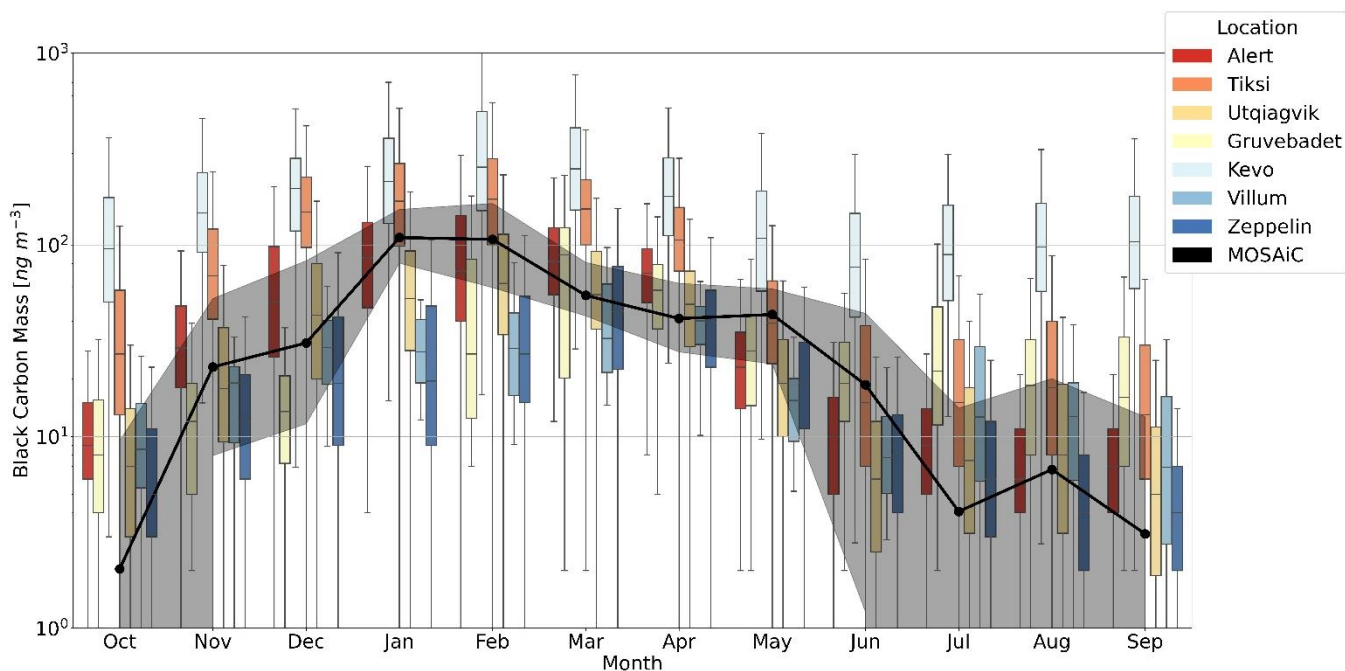
545 Figure 10: A comparison of BC mass concentrations in the Arctic between land-based observatories and MOSAiC. The MOSAiC BC mass concentrations (black line, Aethalometer) are displayed as monthly medians, and the shaded region shows the interquartile range. The boxes for the various sites represent BC and EC mass concentrations spanning several decades, where the time range varies by site (Alert: 1989–2017, Gruvebadet: 2010–2018, Kevo: 1964–2010, Tiksi: 2009–2018, Utqiagvik: 1991–2019, Villum: 2009–2018, Zeppelin: 2001–2017). See Section 2.3 for details on the BC measurement methods, and refer the Schmale et al. (2022) for details on the long term measurements from the land-based sites.
