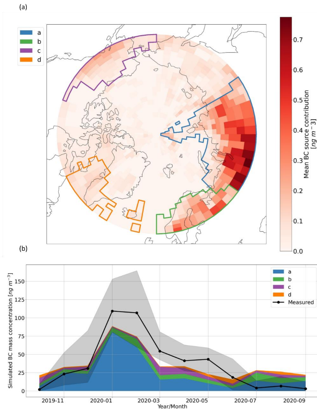
470 Figure 7: Annual cycle of BC mass concentrations and inverse model results. (a) The source contribution map for BC as simulated by the inverse model. The red color bar shows the annual average source contribution according to geographic location, determined using the FLEXPART air tracer data and the measured BC mass concentrations. The polygons on the map indicate the main source region clusters during the year, which were used to evaluate the simulated BC mass concentration time series. Polygon a, b, c, and d are generally characterized as Russia/Siberia, Europe, Alaska, and Greenland/Iceland, respectively. (b) The time series of source region cluster contributions to the simulated BC mass concentrations throughout the year. The BC mass concentrations measured during MOSAiC are included for reference, where the grey shaded region shows the interquartile range.
