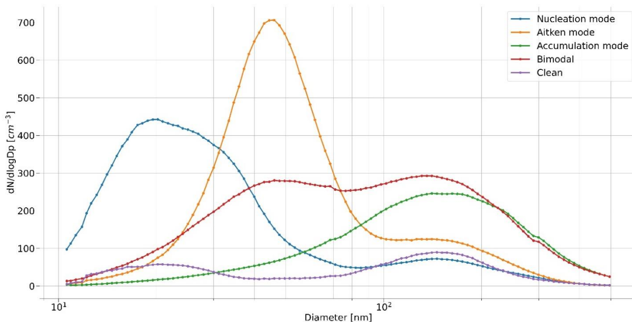
Figure 3: The average distributions of the PNSD clusters. The particle concentration in units of dN/d\log D_p is presented for the average of all days in each cluster according to the particle size. Note that the nucleation and accumulation mode clusters presented here are the result of manually grouping the two nucleation mode clusters and four accumulation mode clusters into a single nucleation and accumulation mode cluster, respectively. Refer to Fig. S3 for the original 9 cluster output.
