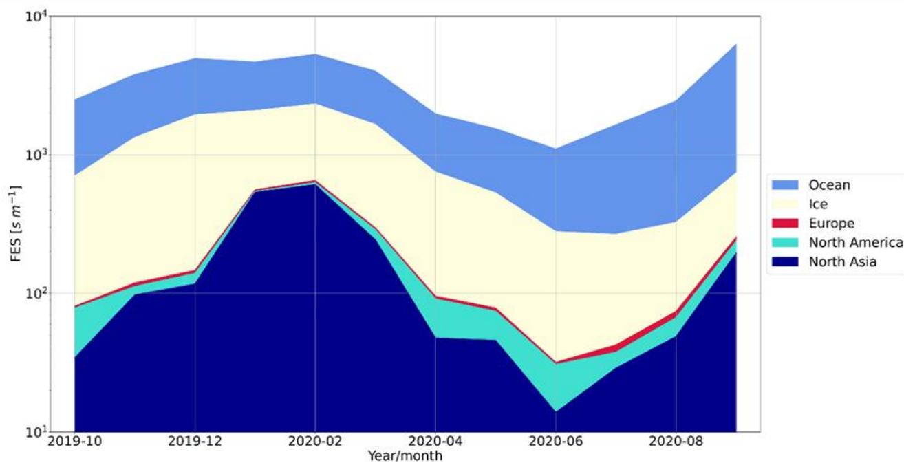
295 Figure 2: The seasonality of surface influence from air mass source regions using FLEXPART. The FLEXPART air tracer data within the lowest 100 meters of the atmosphere, or the FES, was used to identify the influence of different source regions on the observed aerosol throughout the year. The FES was quantified for each source region by applying a geographical mask (a) to the FLEXPART air tracer data.
