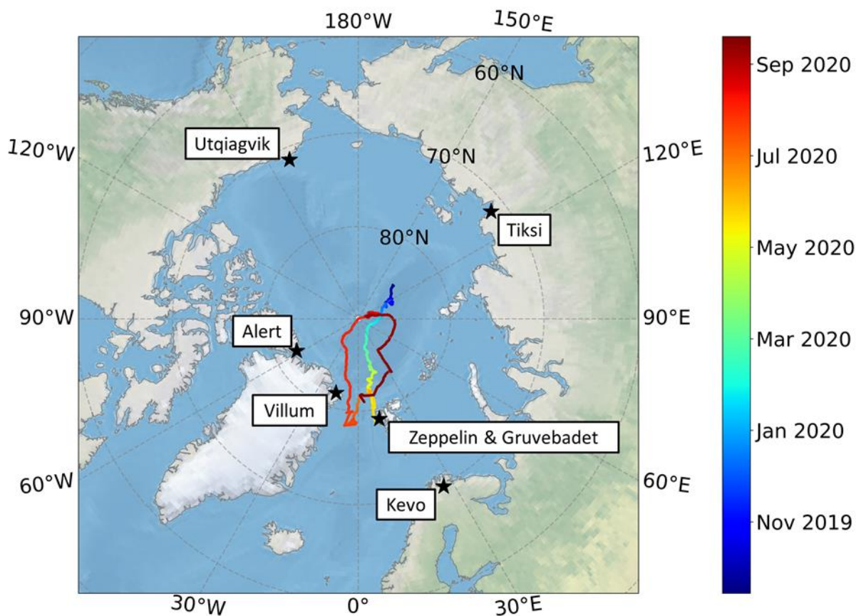
140 Figure 1: The drift track during MOSAiC. The color bar depicts the time of year. The black stars show the location of the land-based sites across the Arctic that are referred to in this study. Note that Zeppelin and Gruvebadet are both located in Ny-Ålesund, Svalbard, Norway, however, the two stations are located at different altitudes. Gruvebadet is ~50 m above sea level, whereas Zeppelin is ~500 m above sea level.
