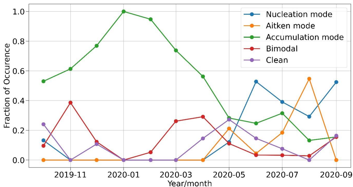
340 Figure 5: The monthly fraction of occurrence for the PNSD clusters. The fraction of occurrence shows the total number of days per month that each cluster is represented compared to all other PNSD clusters.
