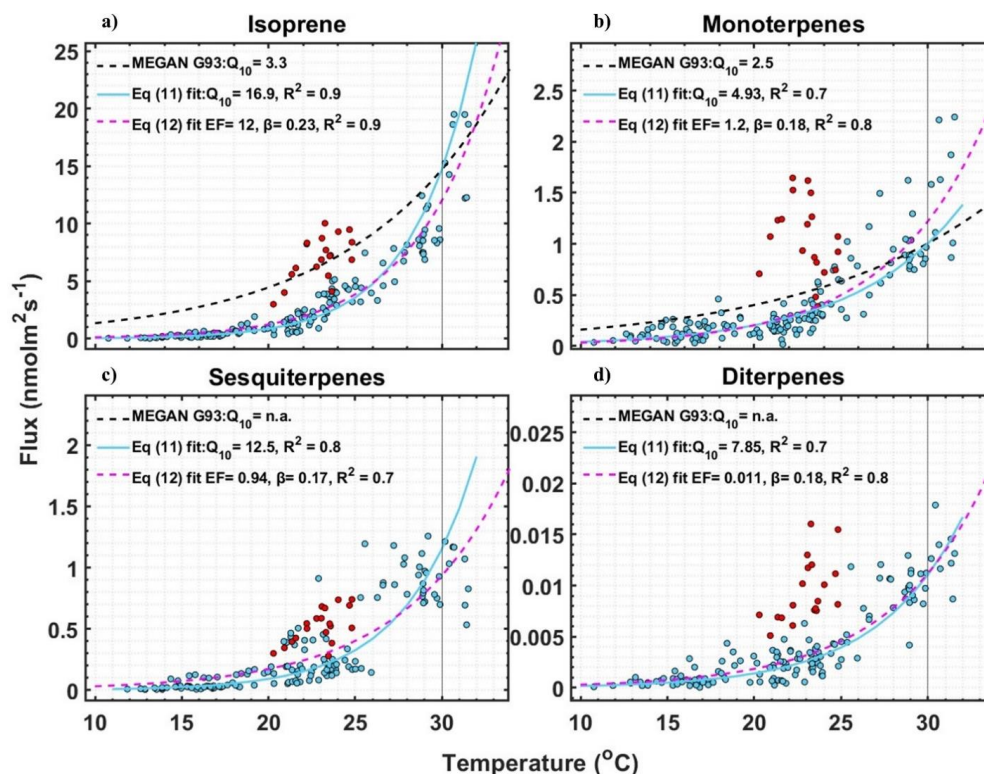
Figure 3. Measured fluxes of (a) isoprene, (b) monoterpene, (c) sesquiterpene, and (d) diterpenes fluxes vs. temperature of data points that passed EC quality criteria and that have PAR > 1000 μmol m -2 s -1 . Q 10 values were calculated by fitting the data with Eq 11. EF and β are calculated by fitting the data with Eq 12. The dashed black line shows the relationship with leaf temperature of the temperature activity factor (C T ) of the G93 model (Guenther et al., 1993), scaled to match emissions at 30°C. The red data points are the flux measurements after the maximum temperature day, 22nd June 2021, when the air temperature crossed 31°C and are not included in the fits.
