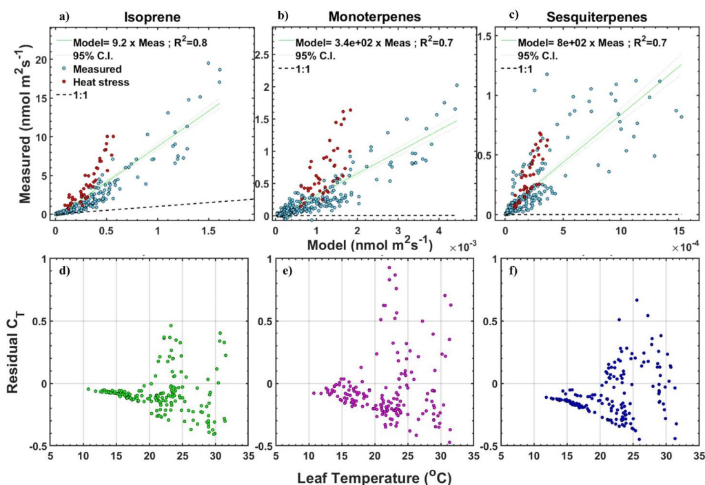
Figure 4. Measured vs. MEGANv2.1 emission for (a) isoprene, (b) MTs, and (c) SQTs of data points that passed EC quality criteria. The red color-coded data points are the flux measurements after 22nd June 2021 and are included in the fits. Residual C_T (measured C_T – MEGANv2.1 C_T ) of (d) isoprene, (e) MTs, and (f) SQTs vs. leaf temperature of data 485 points that passed EC quality criteria and that have PAR > 1000 \mu\text{mol m}^{-2}\text{s}^{-1} for the whole campaign.
