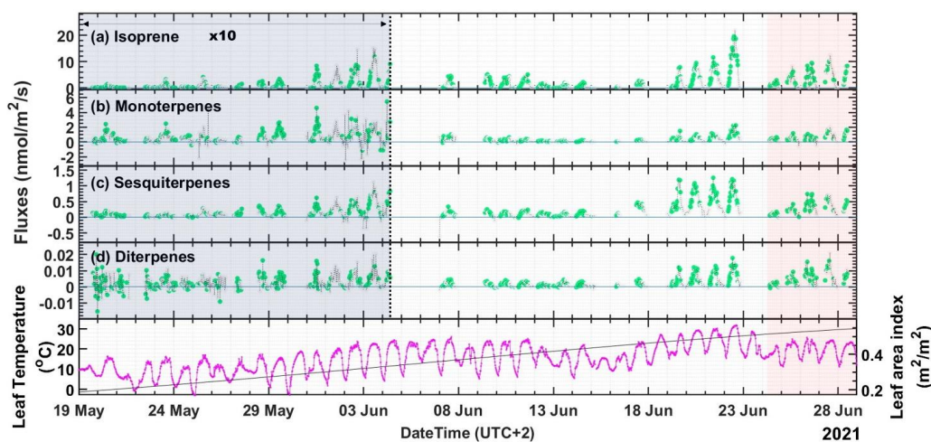
Figure 2. Fluxes of terpenes (a-d) and leaf temperature with leaf area index (LAI) (bottom panel) measured throughout the campaign. Note that the panels (a)-(d) are split into two, and the flux measurements up to 4 June are multiplied by 10 to increase the visibility of the lower values earlier in the campaign. Fluxes colored in green (class 1-3) are good flux periods and are used for fundamental research. The gray data points can only be used for orientation of flux or other
