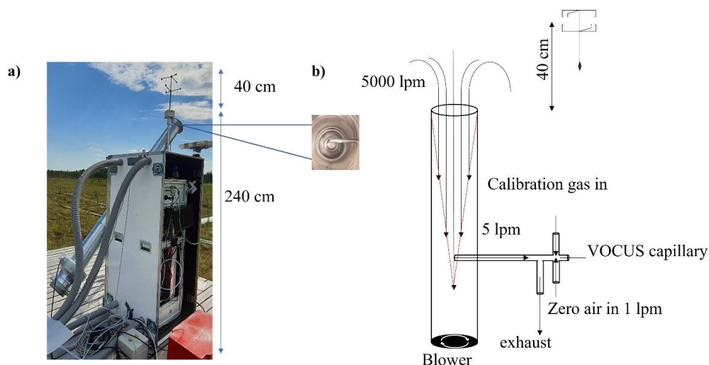
Figure 1. a) Eddy covariance flux measurement setup with high-flow inlet with the core sampling inlet visible when looking straight into the main inlet (inset), and b) schematic of the flows involved in sampling, calibrating and zeroing.
