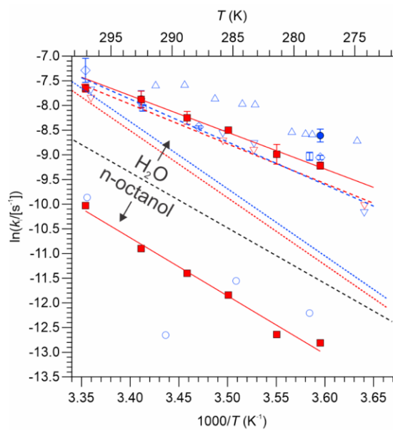
Figure 6. Natural logarithm of k_1 of PAN (blue color) and PPN (red color) in DI water and n-octanol plotted versus 1000/T . Data from this work are shown as solid symbols (● for PAN and ■ for PPN). Literature data: × (Holdren et al., 1984). Δ (Kames et al., 1991). ∇ (Kames and Schurath, 1995). ◇ (Frenzel et al., 2000). ○ (Roberts, 2005). Error bars for the data by Roberts (2005) are omitted for clarity. The dashed blue and red lines (---) are the expressions by Kabir et al. (2014) for thermal dissociation of PAN and PPN, respectively. The dashed, black line serves as a visual indicator to separate results obtained with n-octanol (bottom portion of graph) from those obtained with DI water (top).
