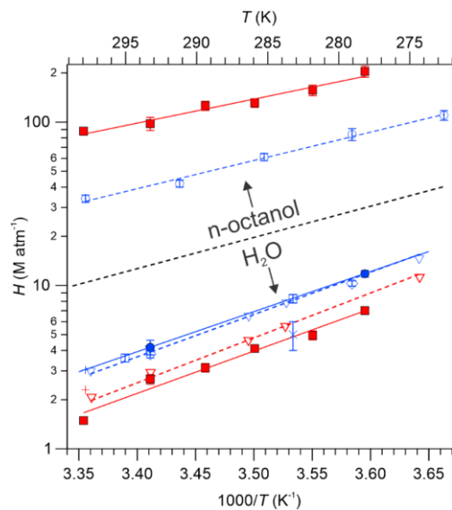
Figure 5. Henry's law constants for PAN (blue color) and PPN (red color) for in n-octanol and DI water as functions of temperature. Data from this work are shown as solid symbols (● for PAN and ■ for PPN). Data from Figure 6 of Kames and Schurath (1995) for PAN and PPN were extracted using "Engauge Digitizer" software (Mitchell, 2021) and are shown as ▽ and --. Other literature data are shown as follows: □ (Lee, 1984). × (Holdren et al., 1984). △ (Kames et al., 1991). ◇ (Frenzel et al., 2000). ○ and -- (Roberts, 2005). + (Raventos-Duran et al., 2010). The dashed, black line serves as a visual indicator to separate results obtained with n-octanol (top portion of graph) from those obtained with DI water (bottom).
