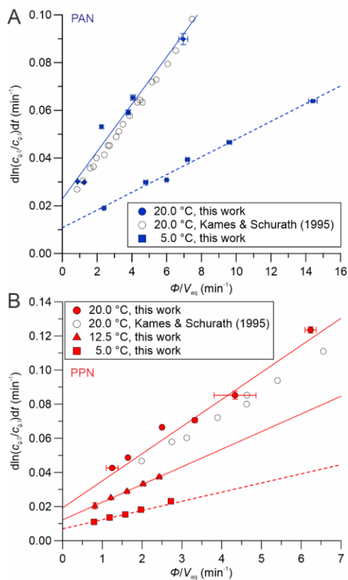
Figure 4. (A) Plots of \ln(c_{g,0}/c_{g,t})/dt versus \Phi/V_l for PAN in DI water at 20.0 °C (●) and 5.0 °C (■). Literature data at 20.0 °C were extracted from Figures 4 and 5 of Kames and Schurath (1995) using "Engauge Digitizer" software (Mitchell, 2021) and are shown as open symbols (○). The lines are linear fits to the data at each temperature. (B) Same plot as panel (A) but for PPN in DI water and also showing data at 12.5 °C (▲).
