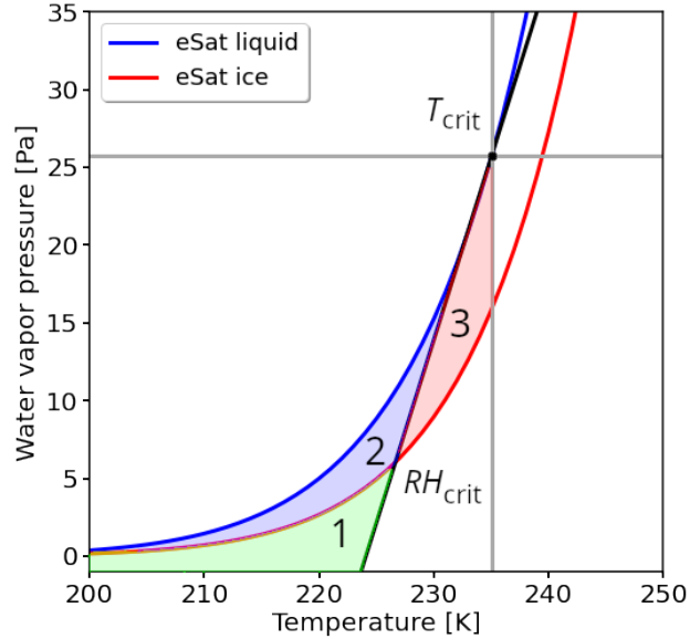
Figure 2. Water-vapor-pressure–temperature diagram with saturation water vapor pressure over ice (red curve) and liquid water (blue curve). Conditions prone to the formation of NPSs are shown in green (R1-NPC); conditions prone to the formation of PC are shown in blue (R2-PC). The potential reservoir for spreading contrail is highlighted in red (R3-R). The critical temperature and relative humidity determined by the Schmidt–Appleman criterion are located on the black line, which separates potential contrail formation (left) from no contrail formation (right).
