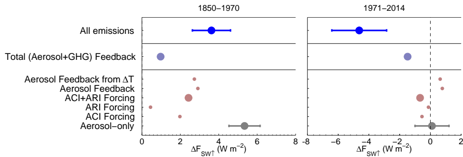
Figure A6. As for Fig. 10 except for the HADGEM-based DAMIP experiments.
