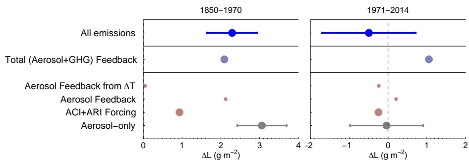
Figure A8. As for Fig. 12 except for the HADGEM-based DAMIP experiments.
