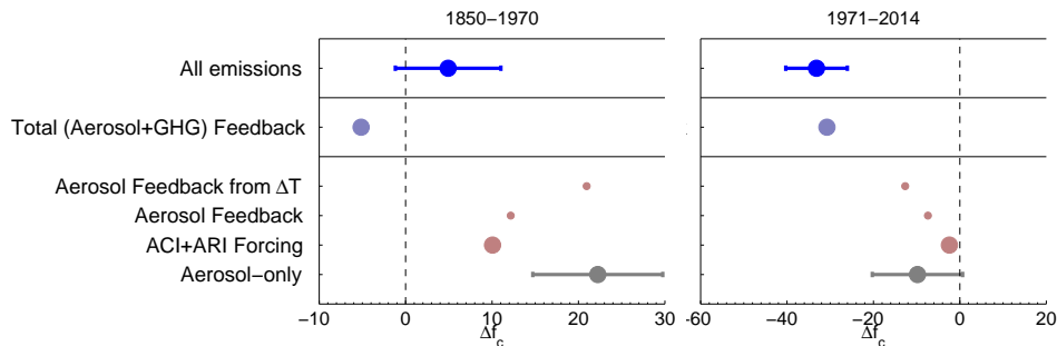
Figure 11. As for Fig. 10 except for f_c and that the aerosol forcing term is not further split into ACI and ARI contributions.
