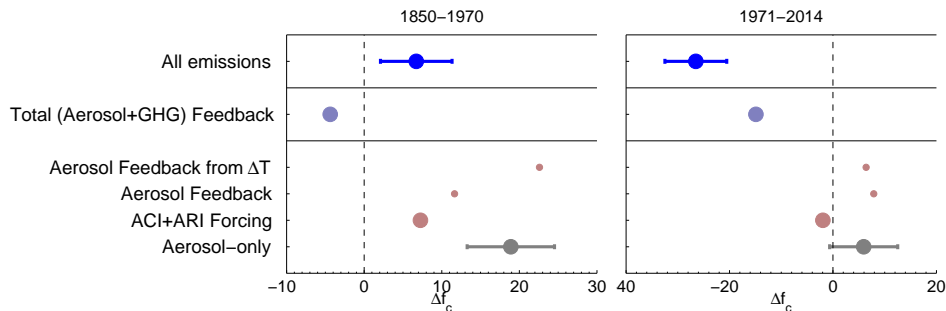
Figure A7. As for Fig. 11 except for the HADGEM-based DAMIP experiments.
