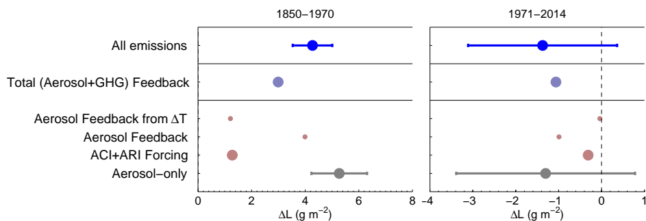
Figure 12. As for Fig. 10 except for L and that the aerosol forcing term is not further split into ACI and ARI contributions.
