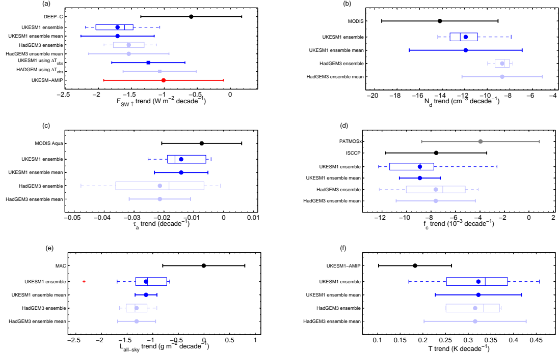
Figure 14. Model trends compared to observed trends for time periods chosen to match the available observations: 1985-2014 for Deep-C F_{SW\uparrow} observations; 2003-2014 for MODIS N_d and MODIS \tau_a ; 1983-2009 for PATMOSx and ISCCP f_c ; 1988-2014 for MAC LWP; 1985-2014 for the surface temperature UKESM atmosphere-only (AMIP) dataset (more data is available for surface temperature, but this period was chosen to coincide with the F_{SW\uparrow} time period). For F_{SW\uparrow} in (a) estimates of the model trend that would occur if the model surface temperature was correct (i.e., equal to the observed temperatures) are also shown (“using \Delta T_{obs} ”; \Delta F_{SW\uparrow,corrected} in Eqn. 6). For the models box and whisker plots of the trends across all ensemble members are shown along with the trend from the ensemble mean timeseries and its uncertainty. The box and whisker plots show the minimum and maximum as whiskers (or errors bars), except when there are outliers when the error bars are the minimum and maximum of the non-outlier values. Outliers are values that are more than 1.5 times the interquartile range away from the bottom or top of the box and are represented as plus signs. The box edges are the 25th and 75th percentiles, the line within the box is the median and the filled circle is the mean.
