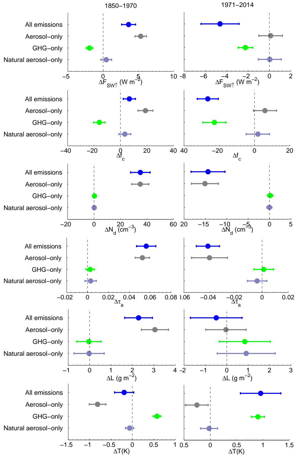
Figure A3. As for Fig. 7 except for the DAMIP and HadGEM simulations. A natural aerosol-only bar is now shown from the DAMIP-HistNat experiment.
