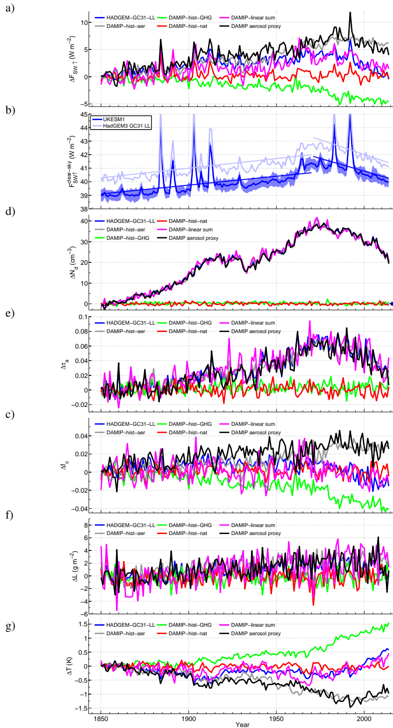
Figure A1. As for Fig. 6 except for the various single-forcing DAMIP simulations. Lines are shown for the HadGEM-GC3.1 model (which is the model used for the DAMIP experiments) with all forcings applied, the aerosol only forcing DAMIP run (DAMIP-hist-aer), the greenhouse gas only forcing run (DAMIP-hist-GHG), the natural only forcing run (DAMIP-hist-nat), the sum of the perturbations from all of the single forcing runs (DAMIP-linear-sum) and the estimate of the aerosol emissions perturbations calculated by subtracting the greenhouse gas-only values from the all-emissions HadGEM values (DAMIP aerosol proxy).
