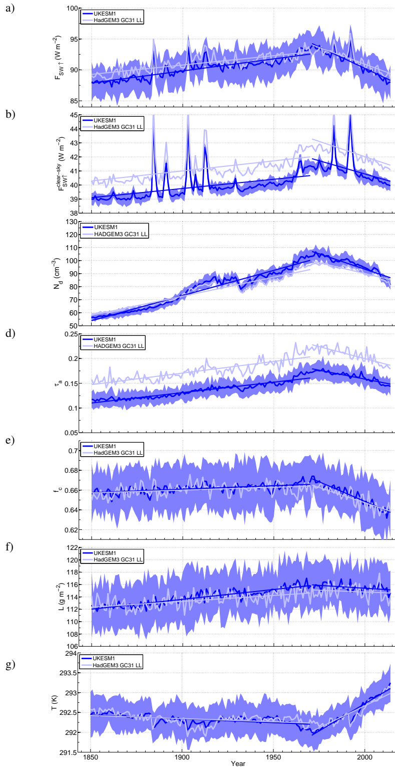
Figure 2. Timeseries of annual mean values of various quantities from the UKESM1 model spatially averaged over the North Atlantic region (18-60° N, 0-75° W; ocean-only gridpoints with sea-ice regions excluded, see text for details). The blue shading denotes \pm 2 times the standard deviation across the ensemble for UKESM1 only. a) the all-sky upwelling SW flux at TOA ( F_{SW\uparrow} ); b) the all-sky upwelling SW flux at TOA ( F_{SW\uparrow}^{\text{clear-sky}} ); c) The vertically averaged (weighted by liquid water content) cloud droplet concentration ( N_d ); d) the aerosol+dust
