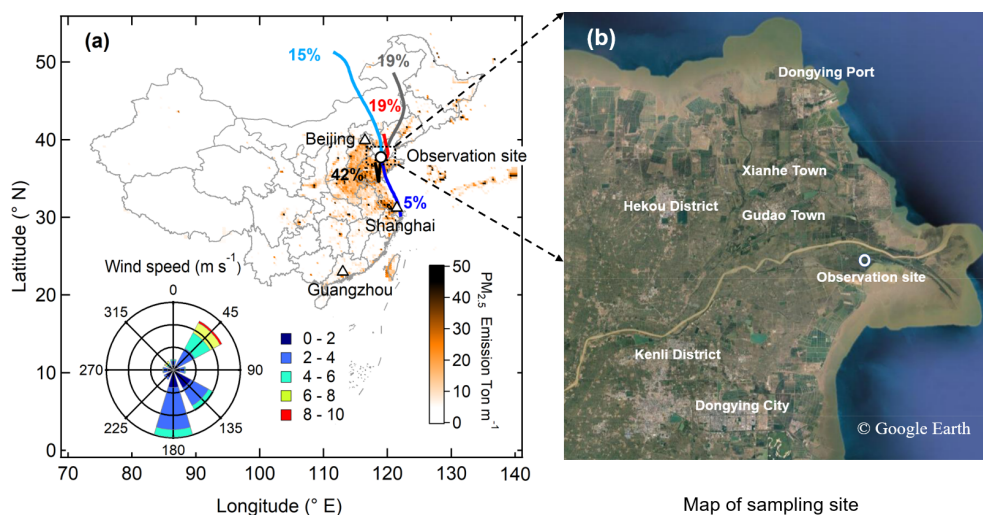
Figure 1. (a) Location of observation site (circle) in China, along with wind speeds, wind directions, and back trajectories of air masses during this campaign. The map is color-coded according to \text{PM}_{2.5} emission inventory (M. Li et al., 2017). (b) Map of the Yellow River Delta National Nature Reserve (YRDNNR) region, labeled with the sampling site (circle) and adjacent cities and towns (source: Google Earth).
