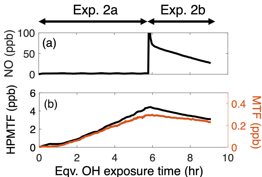
575 Figure 4: (a) NO concentration measured by the \text{NO-NO}_2\text{-NO}_x analyzer in Exp.2. At OH exposure \sim 5.8 h, 70 ppb of NO was injected into the chamber. (b) Time series of HPTMF- ^{12}\text{C}_2 and MTF- ^{12}\text{C}_2 in Exp. 2. The decay of HPMTF and MTF were used to estimate their reaction rate coefficients with OH.
