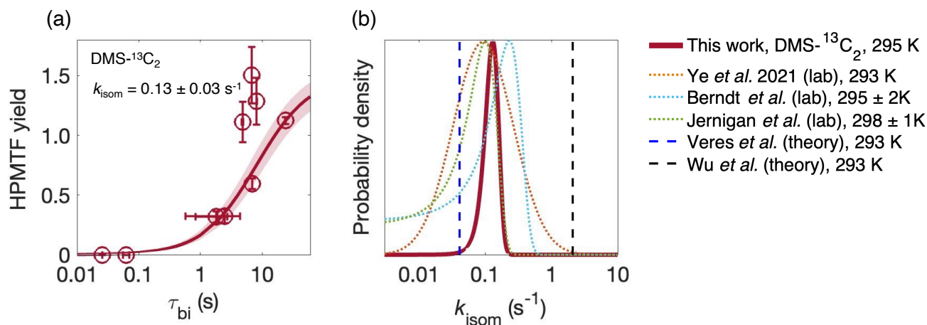
570 Figure 3: (a) The yield of HPMTF in the abstraction channel as function of the bimolecular lifetime \tau_{bi} of \text{CH}_3\text{SCH}_2\text{OO} from the \text{DMS-}^{13}\text{C}_2 data. The shaded area is 1\sigma of the fit, which takes into account uncertainty in both \tau_{bi} (arising from errors in [\text{NO}] and [\text{HO}_2] ) on the x axis, and instrument noise on the y axis. Uncertainty in the CIMS sensitivity to HPMTF affects the absolute measurements but not the inflection point of the curve, or the derived value of k_{isom} . (b) Comparison of k_{isom} from this work with previous determinations of k_{isom} at 293-298 K (Berndt et al. , 2019; Jernigan et al. , 2022a; Veres et al. , 2020; Wu et al. , 2015; Ye et al. , 2021).
