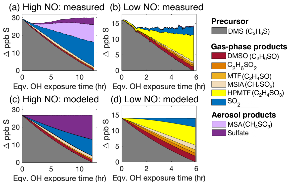
560 Figure 2: Stacked plots showing the total sulfur measured (a and b) and modeled (c and d) under high-NO (a and c) and low-NO (b and d) conditions. Panels a and c are for Exp. 1 and Panels b and d are for Exp. 2a. Data shown in (b) are from DMS- ^{12}C_2 and DMS- ^{13}C_2 combined. Products with a formula of C_2H_6SO_2 may be DMSO _2 and/or CH_3SCH_2OOH ; under high-NO conditions, they are likely to be predominantly DMSO _2 . Minor products detected but not listed in the legend due to their very low concentrations include CH_2SO_2 (a sulfene or thioacid) and CH_3SO_6N (likely methanesulfonyl peroxyxynitrate). Note that y axes denote the changes in concentrations of the precursor and products.
