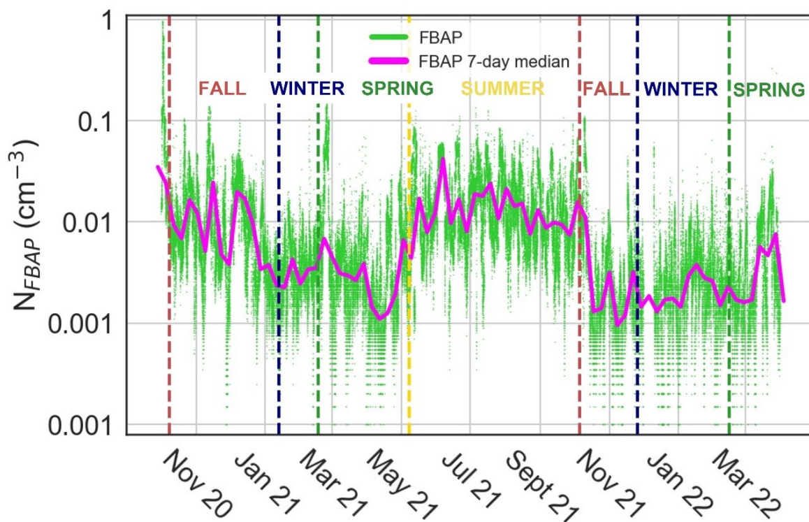
210 Figure 1: Overview of fluorescent biological aerosol particle number concentration ( N_{\text{FBAP}} ) between 6 October 2020 and 1 April 2022. Green dots represent individual N_{\text{FBAP}} 5 min data averages and magenta curve shows running 7-day median values. Vertical dashed lines indicate the first day of each season as identified by the Swedish Meteorological and Hydrological Institute. N_{\text{FBAP}} abundance is seen to increase steeply at the intersection of spring and summer (~ 8 215 May 2021) and decrease steeply in the beginning of fall (~6 October 2021). The highest N_{\text{FBAP}} concentrations were measured in the summer and the lowest concentrations were measured in the winter periods.
