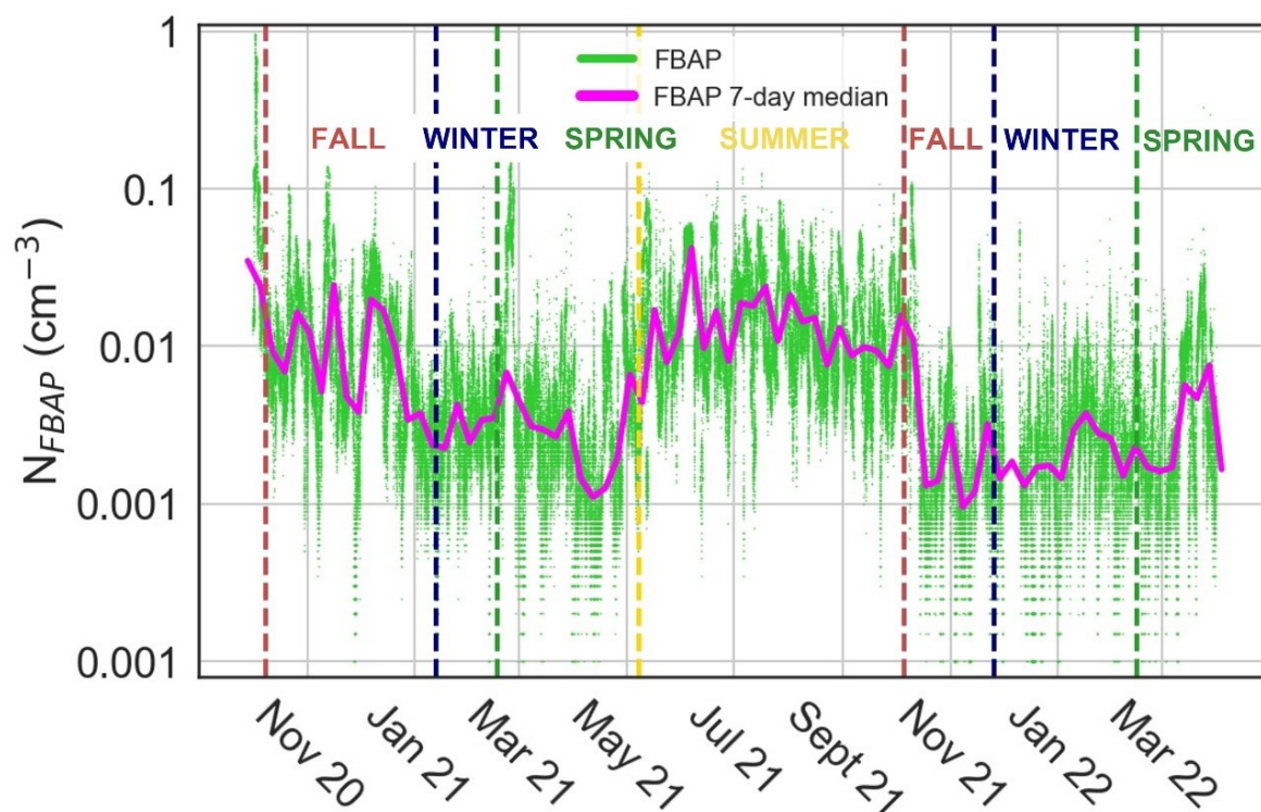
215 Figure 1: Overview of fluorescent biological aerosol particle number concentration ( N_{\text{FBAP}} ) between 6 October 2020 and 1 April 2022. Green dots represent individual N_{\text{FBAP}} 5 min data averages and magenta curve shows running 7-day median values. Vertical dashed lines indicate the first day of each season as identified by the Swedish Meteorological and Hydrological Institute. N_{\text{FBAP}} abundance is seen to increase steeply at the intersection of spring and summer ( \sim 8
