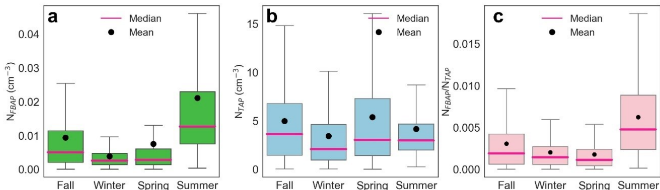
255 Figure 3. Seasonal statistical distribution of fluorescent biological aerosol particle number concentration (left), total supermicron aerosol particle number concentration (middle) and their ratio (right) as box-whisker plots. Lower and upper limits of box represent 25 th and 75 th percentiles, respectively. Vertical bars at the end of lower and upper vertical bars represent 5 th and 95 th percentiles, respectively. Outliers were removed from the plots to make them easier to read.
