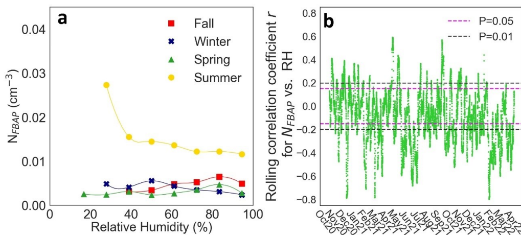
405 Figure 6: Seasonal association between N_{\text{FBAP}} concentrations and relative humidity. Median N_{\text{FBAP}} concentration as a function of relative humidity for each season (a) and the 7-day rolling correlation coefficient r for hourly mean N_{\text{FBAP}} and relative humidity (RH) for the full campaign (b). Horizontal dashed lines indicate the range at which the correlation was nonsignificant at levels 0.05 (magenta) and 0.01 (black). In most cases (46 %) the relationship observed was nonsignificant with very low correlation coefficients.
