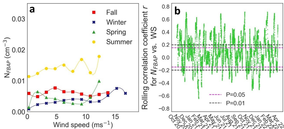
445 Figure 7: The relationship between FBAP number concentrations and wind speed on a seasonal basis (a) and the rolling correlation for the relationship over the full campaign (b). An overall positive relationship was observed between NFBAP and wind speed for all seasons, which can be observed in both figures, but in many cases the relationship was nonsignificant.
