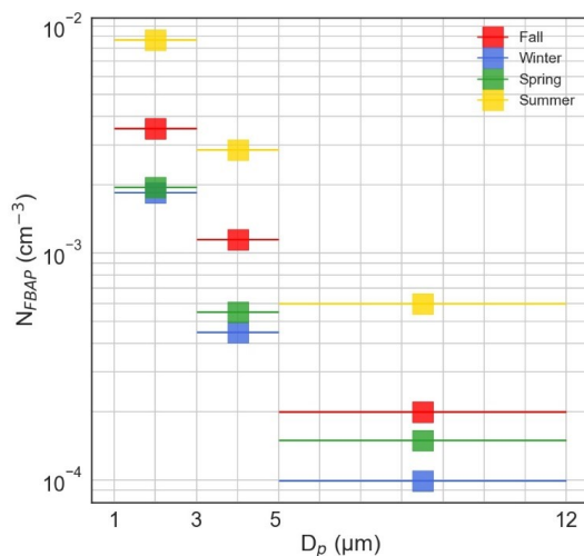
Figure 4: Fluorescence biological aerosol particle (FBAP) number size distribution for the full campaign for three different size bins: 1-3 \mu m, 3-5 \mu m and 5-12 \mu m.
