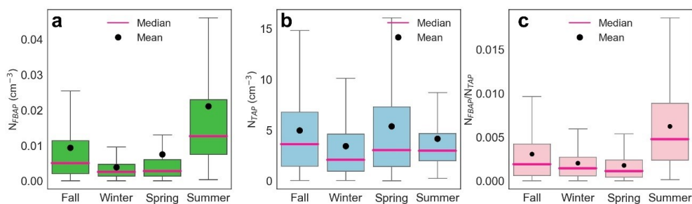
Figure 3. Seasonal statistical distribution of fluorescent biological aerosol particle number concentration (left), total supermicron aerosol particle number concentration (middle) and their ratio (right) as box-whisker plots. Lower and upper limits of box represent 25 th and 75 th percentiles, respectively. Vertical bars at the end of lower and upper vertical bars represent 5 th and 95 th percentiles, respectively. Outliers were removed from the plots to make them easier to read.
