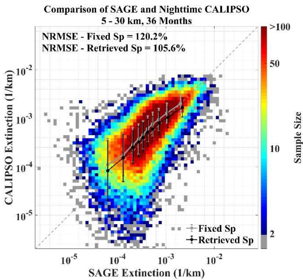
Figure 9. The colored scatter plot is the same as that in Figure 5a, but the CALIPSO extinction is retrieved using fixed lidar ratios of 50 and 28.75 sr in the stratosphere and troposphere from June 2017 to May 2020, respectively. The gray and black lines are the mean value of each 10% quantile (as in Figure 5a) of the CALIPSO retrieved extinction using the fixed and our retrieved lidar ratios, respectively.
