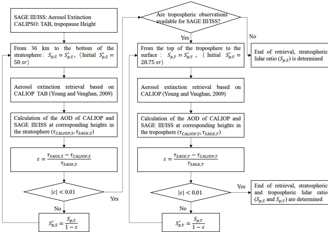
155 Figure 2. Flowchart for the retrieval of lidar ratio by using SAGE III/ISS AOD as a constraint.
