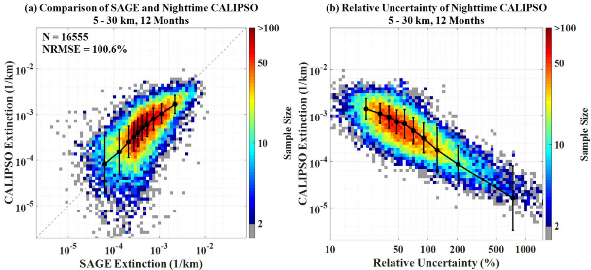
245 Figure 5. (a) Correlation plots of the retrieval within the matching grid of CALIPSO nighttime and SAGE III/ISS product from 5 km to 30 km for 12 months of validation. The color bar represents the sample size. The black bins represent the mean values of each 10% quantile (0-10%, 10-20%...and 90-100%) of SAGE III/ISS 521 nm aerosol product and corresponding CALIPSO retrieval. The I-type bars indicate the standard error of each 10% quantile CALIPSO retrieval. (b) The relative uncertainty of one-degree CALIPSO extinction.
