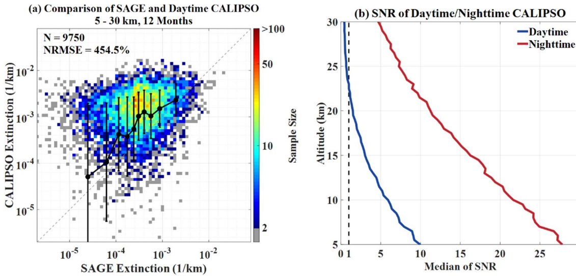
260 Figure 6. (a) Same as in Figure 5a, but at daytime. (b) SNR profiles of the TAB at 20 km horizontal resolution at daytime (blue) and nighttime (red). The SNR is calculated according to SNR = \mu / \sigma based on the pre-processed TAB with 20 km horizontal resolution in the matching range, where \mu and \sigma are the mean and the standard deviation of the signal, respectively.
