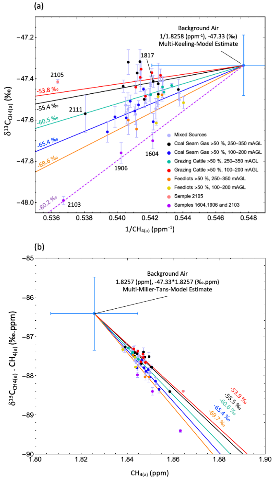
Figure 5. Multiple regression with shared \text{CH}_4(b) and \delta^{13}\text{C}_{\text{CH}_4(b)} for the Keeling model ((a), solid lines, Eq. 1) and the Miller-Tans model ((b), solid lines, Eq. 3) for the category subsets listed in the colour key. Refer to Table A6 for all regression results and their error statistics. The \delta^{13}\text{C}_{\text{CH}_4(s)} signature for each category is listed near the lines of best fit for each category. The dashed purple line in (a) shows a Keeling model (Eq. 1) fitted to IFAA samples 1604, 1906, and 2103 (for this regression \text{CH}_4(b) and \delta^{13}\text{C}_{\text{CH}_4(b)} were fixed to match the results of the multi-Keeling-model regression with shared \text{CH}_4(b) and \delta^{13}\text{C}_{\text{CH}_4(b)} ). To highlight the subtle differences in the multiple regression best fit parameters, the derived \text{CH}_4(b) and \delta^{13}\text{C}_{\text{CH}_4(b)} values are given to an extra significant figure in (a) and (b) compared to the measurement precision. All error bars are one standard deviation.
