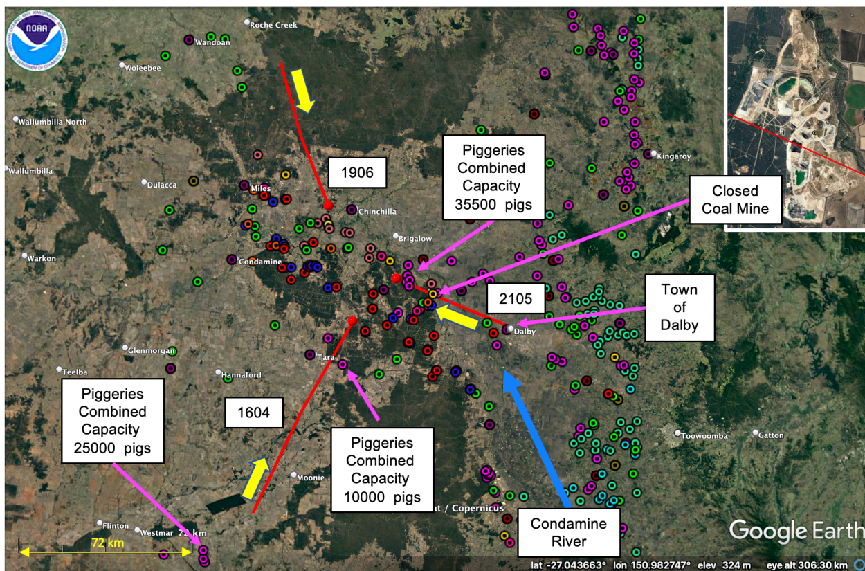
660 Figure 7. Two-hour back-trajectory path lines (red) for IFAA samples 1604, 1906 and 2105. Refer to Fig. A1 for the point source colour key. Yellow arrows show the wind direction. The Condamine River flows from south-east to north-west (blue arrow) (image © Google Earth).
