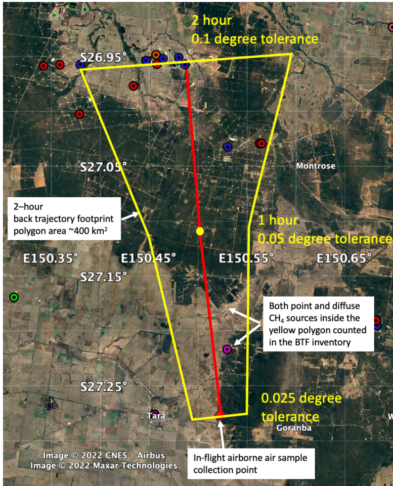
Figure A2. A representative BTF inventory polygon for IFAA sample 1817. The red line shows the 2-hour back trajectory determined using HYSPLIT. Refer to Fig. A1 for the point source colour key (image ©Google Earth).
