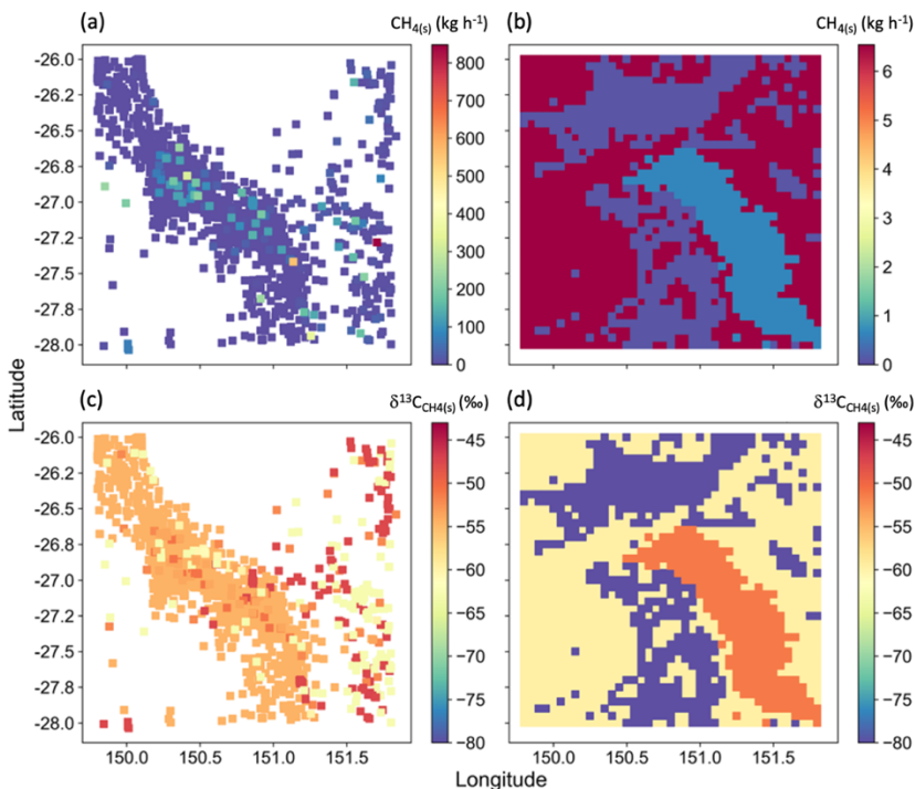
350 Figure 2. Maps of the UNSW BU inventory ( 5 \times 5 \text{ km} for each grid cell) in the southeast portion of the Surat Basin CSG fields showing the estimated \text{CH}_{4(s)} emissions for point (a) and distributed (b) sources and assigned \delta^{13}\text{C}_{\text{CH}_{4(s)}} for point (c) and distributed (d) sources.
