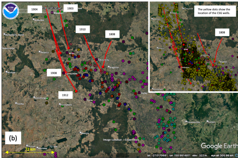
1510 Figure A4. Two-hour HYSPLIT back-trajectory path lines (red) for the points used in the grazing cattle Keeling-model regression analysis. (a) HYSPLIT back trajectories Grazing Cattle > 50 % BU inventory, altitude 250–350 m AGL. (b) HYSPLIT back trajectories Grazing Cattle > 50 % BU inventory, altitude 100–200 m AGL. Refer to Fig. A1 for the point source colour key (image ©Google Earth).
