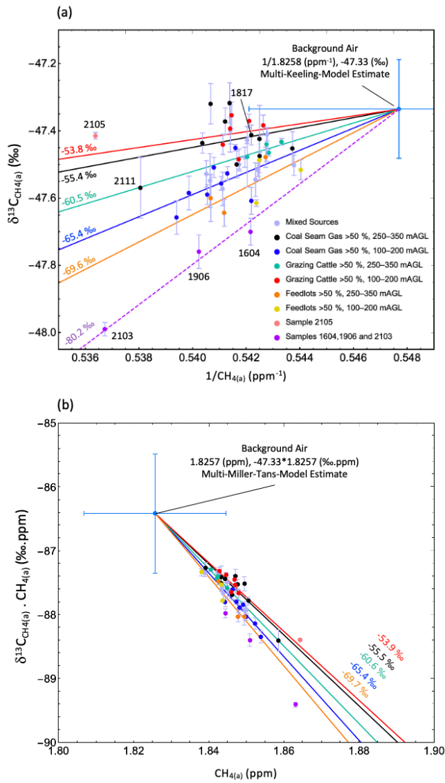
815 Figure 5. Multiple regression with shared CH_{4(b)} and \delta^{13}C_{CH_4(b)} for the Keeling model ((a), solid lines, Eq. 1) and the Miller-Tans model (b), solid lines, Eq. 3) for the category subsets listed in the colour key. Refer to Table A6 for all regression results and their error statistics. 820 The \delta^{13}C_{CH_4(a)} signature for each category is listed near the lines of best fit for each category. The dashed purple line in (a) shows a Keeling model (Eq. 1) fitted to IFAA samples 1604, 1906, and 2103 (for this regression CH_{4(b)} and \delta^{13}C_{CH_4(b)} were fixed to match the results of the multi-Keeling-model regression with shared CH_{4(b)} and \delta^{13}C_{CH_4(b)} ). To highlight the subtle differences in the multiple regression best fit parameters, the derived CH_{4(b)} and \delta^{13}C_{CH_4(b)} values are given to an extra significant figure in (a) and (b) compared to the measurement precision. All error bars are one standard deviation.
