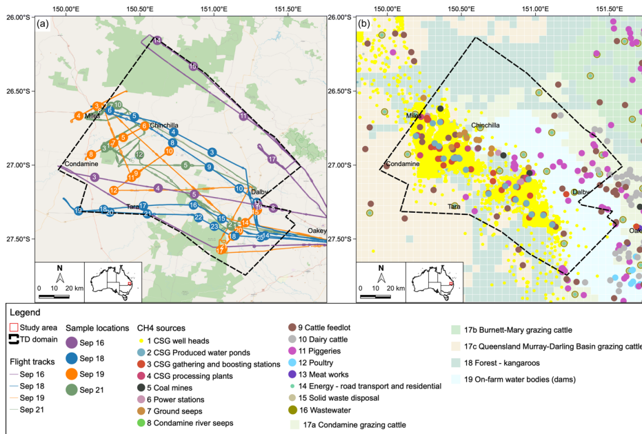
305 Figure 1. Map of the study area with flight tracks and in-flight atmospheric air (IFAA) sample locations (a) (inset map shows the location in south-eastern Queensland) and map of the CH 4 sources in the area (b). (Inset map data: Australian Government (2020), Administrative 310 Boundaries © Geoscience Australia. Base map and data from OpenStreetMap and OpenStreetMap Foundation). The black dashed polygon shows the extent of the TD domain, where the strong correlation between the UNSW BU inventory and the TD mass balance emission estimate was established in Neininger et al. (2021). The diffuse CH 4 emissions were determined for each Australian Bureau of Statistics district (Condamine, Burnett-Mary, and Queensland Murray-Darling Basin) and land use (mixed cropping and grazing, irrigated agriculture, and forest) using annual agricultural production data.
