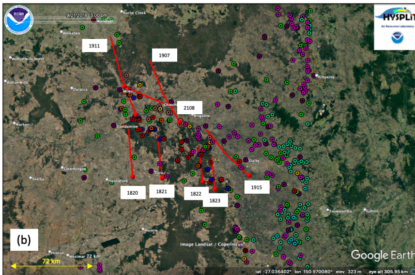
1505 Figure A3. Two-hour HYSPLIT back-trajectory path lines (red) for the points used in the coal seam gas Keeling-model regression analysis. (a) HYSPLIT back trajectories CSG > 50\% BU inventory, altitude 250–350 mAGL . (b) HYSPLIT back trajectories CSG > 50\% BU inventory, altitude 100–200 mAGL . Refer to Fig. A1 for the point source colour key (image ©Google Earth).
