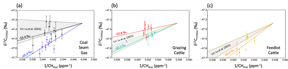
Figure 6. Expected versus measured \delta^{13}\text{C}_{\text{CH}_4(a)} for each \text{CH}_4 source category. The expected source category \delta^{13}\text{C}_{\text{CH}_4(s)} values from Lu et al. (2021), Table A2, are shown as thin continuous Keeling lines (without number values) for the upper and lower Bayesian credible interval for the category (where the credible interval is analogous to the 95 % confidence interval). The thick lines represent Keeling lines based on the IFAA samples (including derived source signatures). The IFAA sample point and measurement uncertainty are also shown for each category data set. The categories are: (a) CSG >50 % BTF inventory, 100–200 mAGL (blue) and CSG >50 % BTF inventory, 250–350 mAGL (black); (b) Grazing Cattle >50 % BTF inventory, 100–200 mAGL (red) and Grazing Cattle >50 % BTF inventory, 250–350 mAGL (green); (c) Feedlots >50 % BTF inventory, 100–350 mAGL (yellow points (100–200 mAGL) and orange points (250–350 mAGL)). All error bars are one standard deviation.
