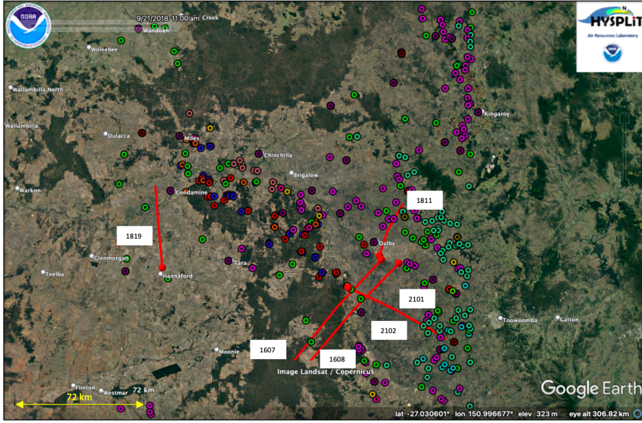
Figure A5. Two-hour HYSPLIT back-trajectory path lines (red) for the points used in the feedlot Keeling-model regression analysis. Each green dot indicates the position of a feedlot (image ©Google Earth).
