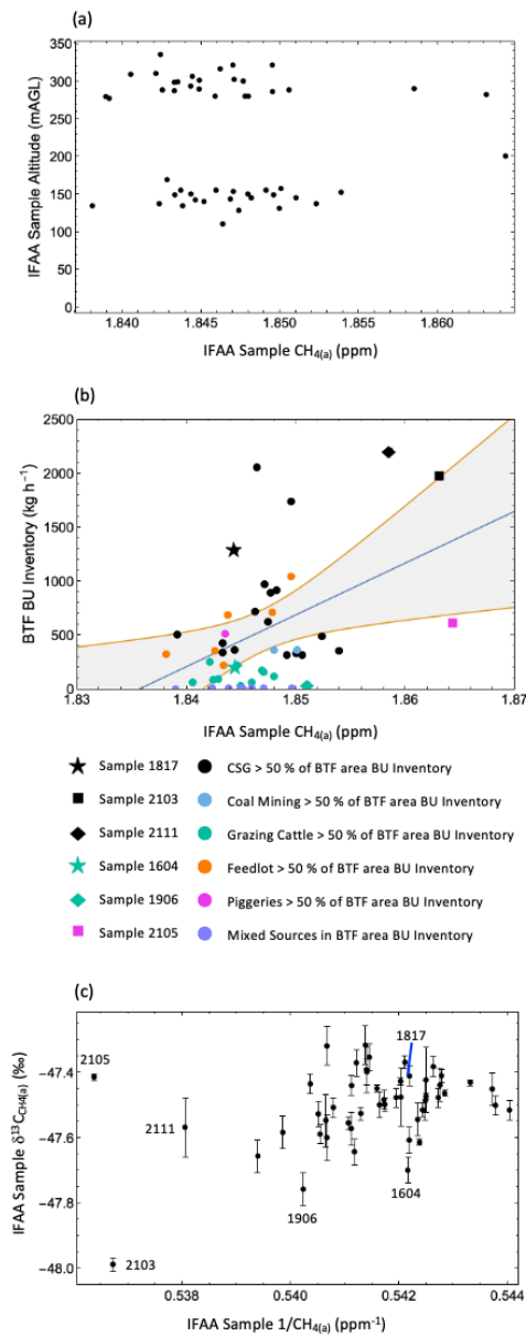
Figure 3. IFAA sample observations between altitudes 100–350 mAGL. (a) IFAA sample altitude (mAGL) versus IFAA sample CH 4(a) (ppm). This plot highlights the sampling at altitudes of approximately 150 m and 300 m. (b) Back trajectory footprint bottom-up (BTF BU) inventory CH 4 (kg h -1 ) versus IFAA sample CH 4(a) (ppm). The linear regression fit highlights the moderate correlation ( R^2 = 0.59 ) between the two variables. The grey zone is the 95% confidence level. (c) A Keeling plot: IFAA samples δ 13 C CH 4(a) versus IFAA sample 1/CH 4(a) (ppm) (The error bars are one standard deviation. For 1/CH 4(a) the errors are too small to be observable; IFAA samples 1604, 1817, 1906, 2103, 2105 are discussed in detail in the main text).
