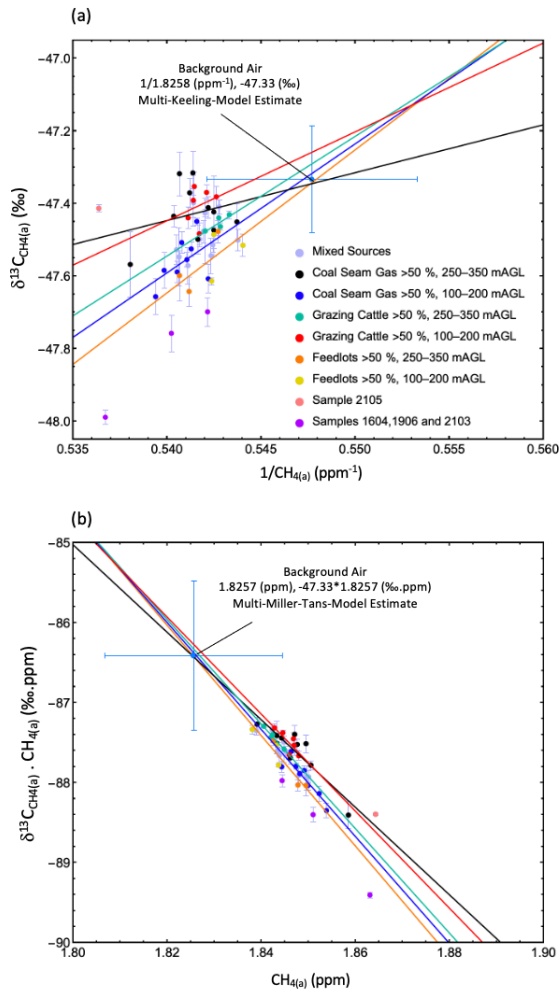
1620 Figure B1. Least squares regression for two-endmember mixing models fitted to individual source category data sets using (a) the Keeling model (Eq. 1) and (b) the Miller-Tans model (Eq. 2). For reference the background air values for \text{CH}_{4(b)} and \delta^{13}\text{C}_{\text{CH}_4(b)} determined from the multi-Keeling and multi-Miller-Tans model regressions are displayed in plots (a) and (b), respectively. The regression statistics for each category are listed in Table B1. Both graphs highlight that when the models are fitted to the individual source category data sets the lines of best fit do not converge to a common value for background air. All error bars are one standard deviation.
