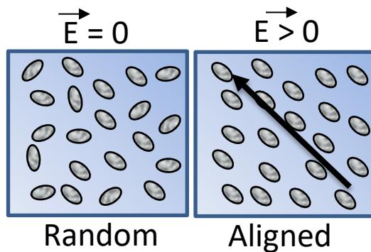
Figure 3: Dust particles in suspension are normally assumed as randomly distributed (right-left panel). But in the presence of an electric field (right panel), they tend to orient along (or precess around) the direction of the field
