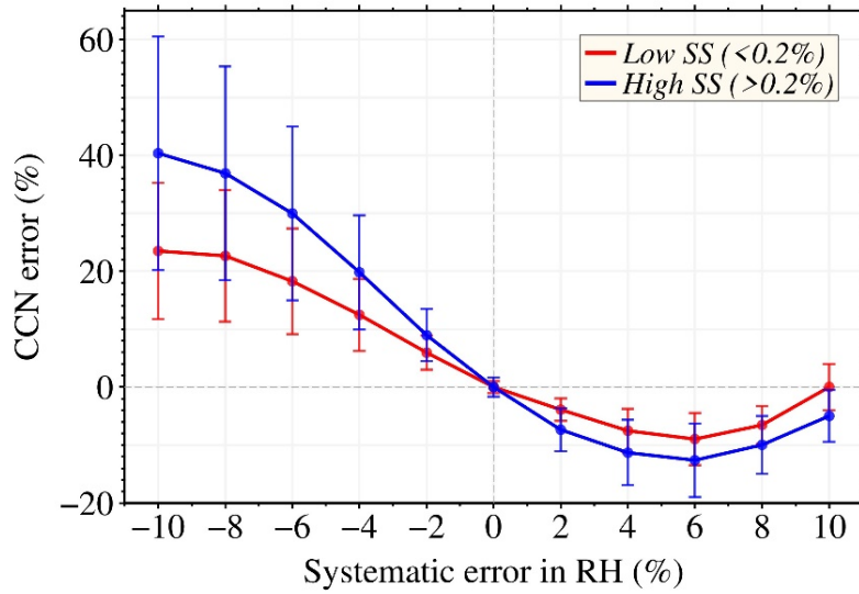
1606 Figure 4: Systematic errors in retrieved N_{CCN} . This represent the errors in retrieved N_{CCN} as a 1607 function of systematic error in RH, combines for all aerosol subtypes, at low ( \leq 0.2\% ) and high 1608 ( > 0.2\% ) supersaturations. The markers denote the mean value and the error bars represent the 1609 standard deviation.
