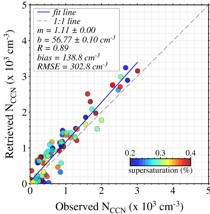
1641 Figure 7: Comparison between retrieved and observed N CCN . The comparison between ECLiAP 1642 retrieved N CCN from HSRL-2 lidar measurements and the measured NCCN values from CCN 1643 counter. The HSRL-2 and CCN counter data were collected from the multiple flights during NASA- 1644 ORACLES airborne campaigns conducted in 2017-2018. The color bar displays the observed 1645 values of supersaturation for each measurement and the NCCN were retrieved on the same 1646 supersaturation for the direct comparison. The slope and intercept of the best fit line are given in 1647 the key by m and b , respectively. The gray dash line indicates the unit slope line and blue solid 1648 line indicates the regression line.
