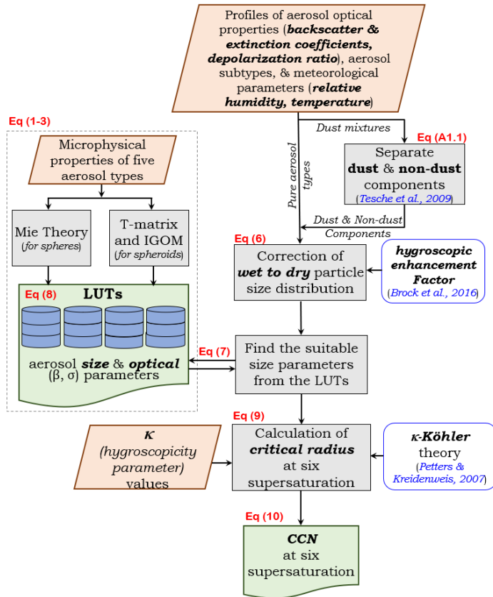
1588 1589 Figure 2: Flowchart of ECLiAP algorithm for the retrieval of N_{CCN} from lidar measurements. 1590 The steps within the dotted line box describes the pre-processing which includes the calculation 1591 of aerosol optical properties using Mie scattering theory (T-matrix/IGOM for dust) to build look- 1592 up-tables for five aerosol models. The steps outside the dotted line box represent the retrieval 1593 process of N_{CCN} from the given inputs of aerosol optical properties and meteorological 1594 parameters. The chart also refers to the used equations associated to the particular retrieval 1595 process.
