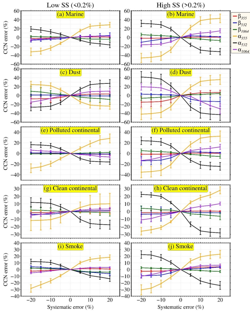
1599 Figure 3: Systematic errors in retrieved N_{CCN} . This represent the errors in retrieved N_{CCN} as a 1600 function of systematic errors in backscatter and extinction coefficients at all three wavelengths for 1601 low ( \leq 0.2\% ) and high ( > 0.2\% ) supersaturations and for all five aerosol subtypes as. The markers 1602 denote the mean value and the error bars represent the standard deviation.
