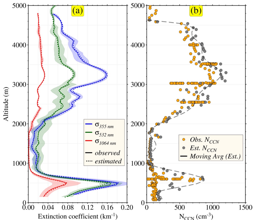
1621 Figure 6: Comparison between retrieved and observed vertical profiles of aerosol extinction 1622 coefficients and N_{CCN} . The ECLiAP retrieved (a) aerosol extinction coefficients at 355, 532 and 1623 1064 nm and (b) N_{CCN} were compared against the one observed during NASA ORACLEs 1624 airborne campaign. The lidar signals were mainly influenced by the mixture of smoke and 1625 dust or marine aerosols. The relationship between HSRL-2 measured aerosol extinction 1626 coefficients (solid lines) and retrieved (dotted line) by an algorithm in the left panel. The right 1627 panel illustrates the comparison of retrieved N_{CCN} using lidar measurements and measured by 1628 CCN counter. The dashed line in the right panel shows the moving average of retrieved N_{CCN} 1629 values. CCN counter measured N_{CCN} at supersaturation ranging from 0.32%-0.34% for the 1630 selected region (described in Figure S4), therefore, the retrieval of N_{CCN} was carried out at 1631 supersaturation of 0.34%.
