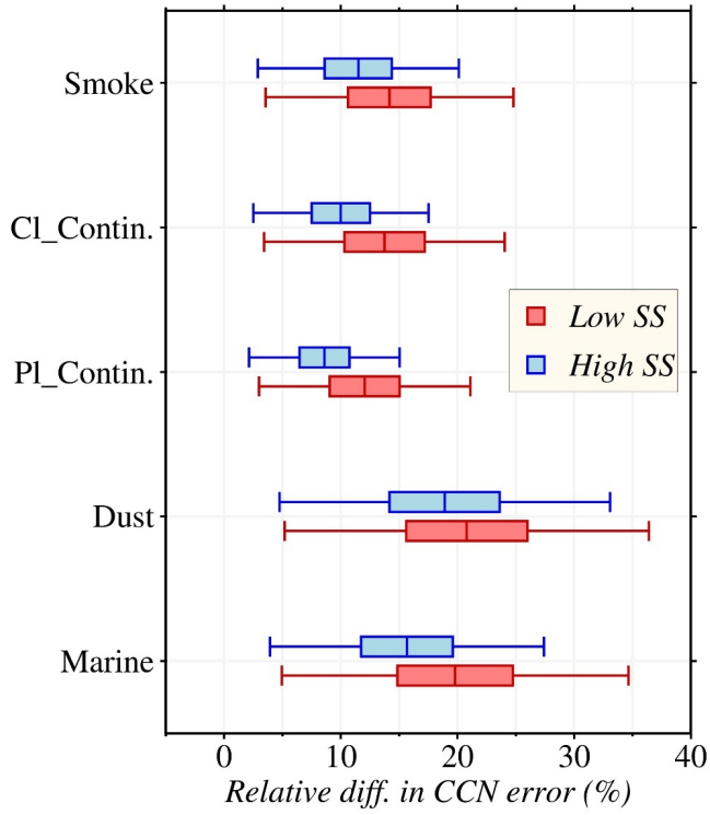
1679 Figure 10: Relative difference in CCN error between 3\beta+2\alpha and 3\beta+3\alpha . The CCN error were 1680 calculated against the given inputs using Eq. (11) for both the 3\beta+2\alpha and 3\beta+3\alpha techniques 1681 individually. Later the relative difference of CCN error has calculated from the individual CCN 1682 errors at low and high supersaturations for each aerosol subtypes.
