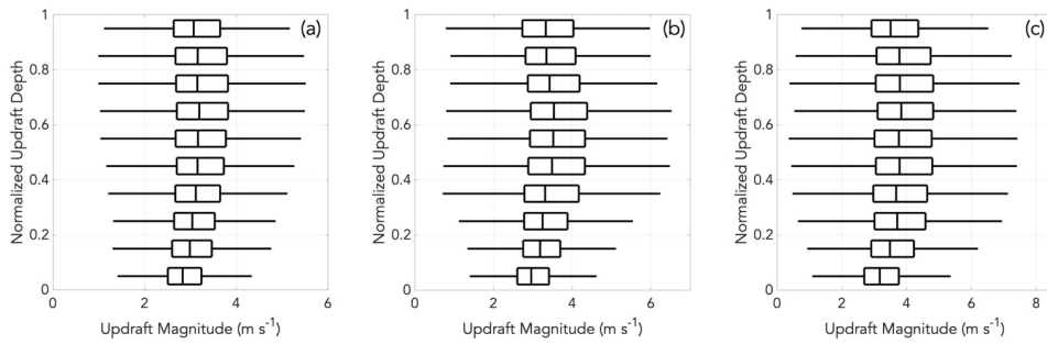
825 Figure 5. For all 13 COMBLE cases, box-and-whisker plots of updraft magnitude as a function of normalized updraft depth for (a) updrafts with a depth less than 1 km, (b) updrafts with a depth between 1 and 2 km, and (c) updrafts with a depth greater than 2 km.
