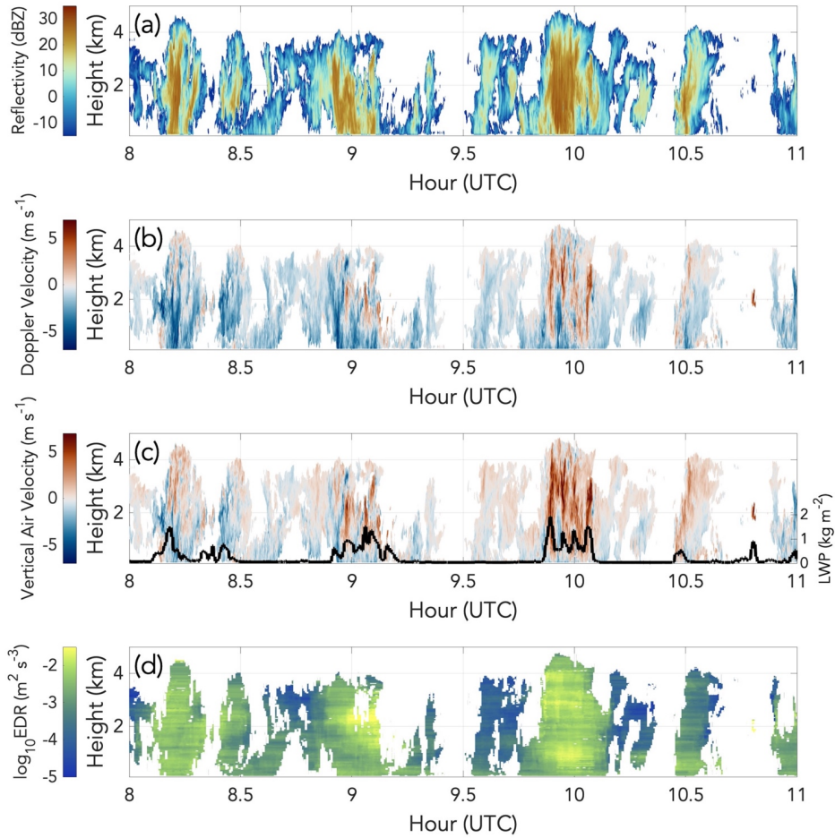
815 Figure 2. Time-height mapping from 8-11 UTC on March 28 th , 2020 of a) KAZR radar reflectivity, b) KAZR Doppler velocity, c) retrieved vertical air velocity and liquid water path, and (d) retrieved eddy dissipation rate.
