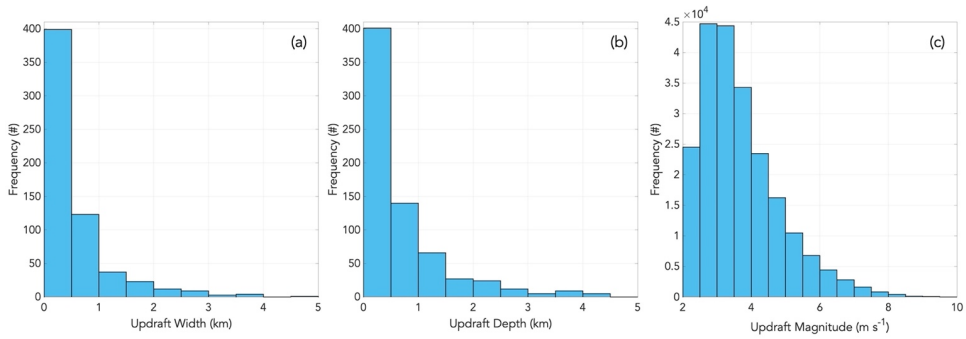
Figure 3. For all 13 COMBLE cases, histograms of a) updraft chord length (width) in km, b) updraft vertical extent in km, and c) the range of magnitudes in the updraft in ms -1 .
