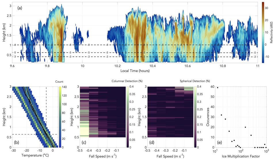
855 Figure 9. For December 31 st , 2019, (a) time-height mapping during 9:36-11 LT of KAZR radar reflectivity (colors) and INTERPSONDE isotherms (dashed black lines); (b) a joint PDF of temperature and height (colors) from 32 radiosondes launched during the 13 cases along with the three temperature profiles from December 31 st (black); and the percentage of Doppler spectra with columnar detections (c) and spherical detections (d) in each fall speed-height bin during 0-18:15 LT.
