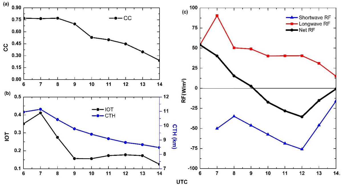
Figure 7/A2: The variations of (a) CC, (b) mean IOT and mean CTH, and (c) SW, LW and net RF within the area indicated by a red box in Fig. 2
